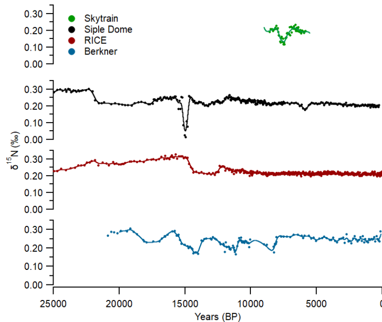
Figure 5. \delta^{15}\text{N} profiles from previously measured coastal WAIS ice cores, Skytrain (this study), Siple Dome (as published in Morgan et al., 2022), RICE (as published in Lee et al., 2020) and Berkner (as published in Capron et al., 2013).
