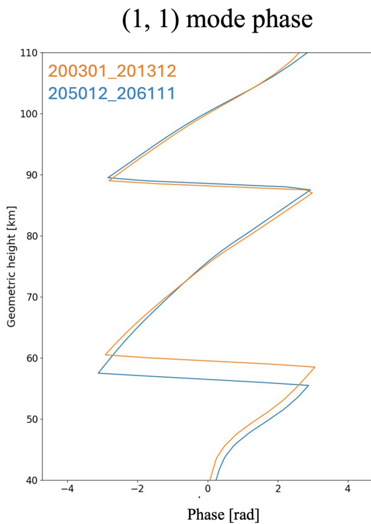
Figure S2. Phases of the tides in 2003–2013 and 2050–2061.
