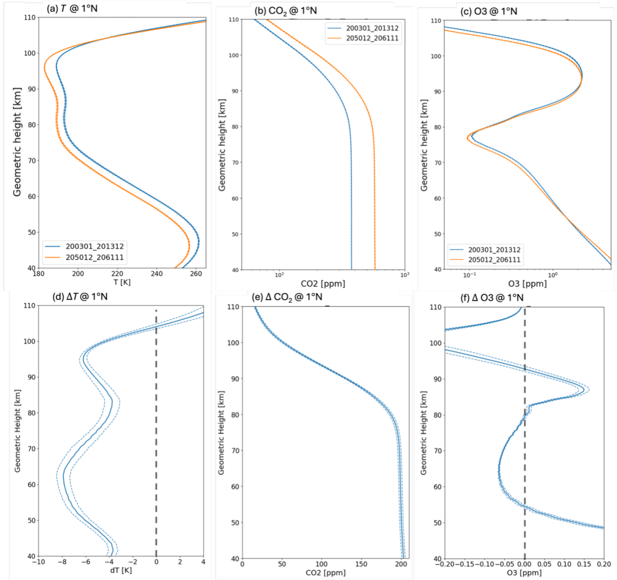
Figure 8. (a) Vertical profile of temperature at 1°N in 200301–201312 (blue) and 205012–20611 (orange). (b) same as (a) but for \text{CO}_2 concentration. (c) same as (a) but for \text{O}_3 concentration. (d) Difference in temperature at 1°N (205012–20611 minus 200301–201312). (e) same as (d) but for \text{CO}_2 concentration. (f) same as (d) but for \text{O}_3 concentration. Dashed lines represent \pm 1 -sigma standard error intervals.
