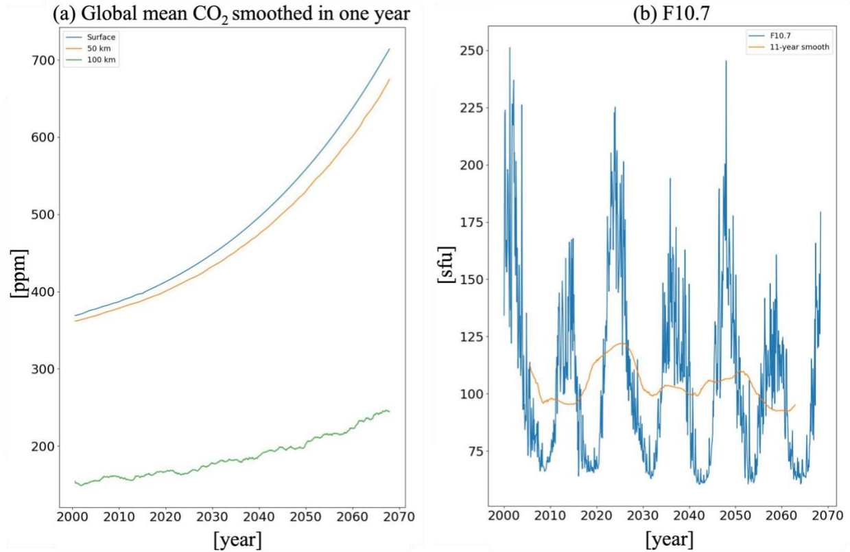
2016); that is, it is specified using historical observations up to 2014, and from 2015 onward, it is simulated using the solar forcing based on historical observational data from 1850 to 1924 levels (Figure 1b). Since future solar forcing cannot be reliably predicted, we used past values following CMIP6. Figure 1. (a) Global mean CO 2 concentrations, smoothed over one year. The blue, orange, and green lines represent CO 2 concentrations at the surface, 50 km, and 100 km altitudes, respectively. (b) F10.7 solar flux (blue) and its 11-year smoothed trend (orange).
