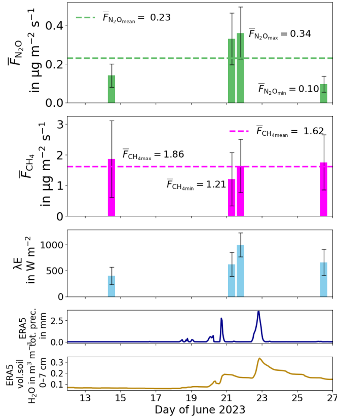
Figure 8. Flight average fluxes of N_2O and CH_4 for four flights conducted during the GHGMon campaign. Green bars represent F_{N_2O} , red bars F_{CH_4} and thin black bars the associated total error margin. The blue bars in the third row are latent heat fluxes, \lambda E . The lowermost subplots indicate the total precipitation and volumetric soil water content from the surface down to -7 cm, for the region between 53.3°N, 5.2°W and 52.2°N, 6.2°W, both inferred from ERA5 reanalysis data.
