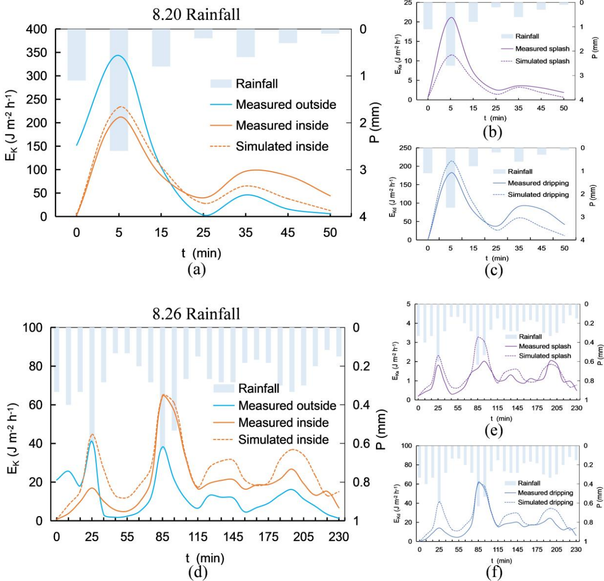
280 Figure 5. Comparison of kinetic energy of rainfall outside the canopy during two rainfall events (a) 8.20 total kinetic energy of
