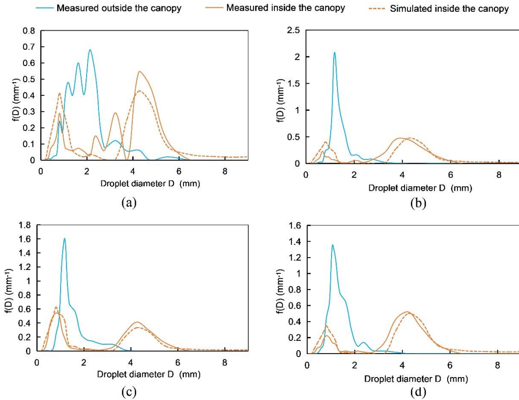
255 Figure 4. Comparison of raindrop spectra outside the canopy and inside the canopy during two rainfall events. f(D) is the volumetric drop-size distribution function (Volume fraction per millimeter (mm -1 )), plotted based on the volume-based frequency. The total area under the entire curve is normalized to 1. (a) Raindrop spectrum of 0-10 min rainfall on 8.20 (b) Raindrop spectrum of 30-40 min rainfall on 8.20 (c) Raindrop spectrum of 0-10 min rainfall on 8.26 (d) Raindrop spectrum of 150-160 min rainfall on 8.26. The OTT Parsivel 2 laser spectrometer uses a non-uniform binning scheme to represent drop size distributions. The full diameter range (0.0625-24.5 mm) is divided into 32 classes with variable bin widths: 0.125 mm for D < 1.25 mm, 0.25 mm for 1.25-2.5 mm, 0.5 mm for 2.5-5.0 mm, and 1.0 mm for D > 5.0 mm. The figure is plotted using the midpoint of each bin as the representative value.
