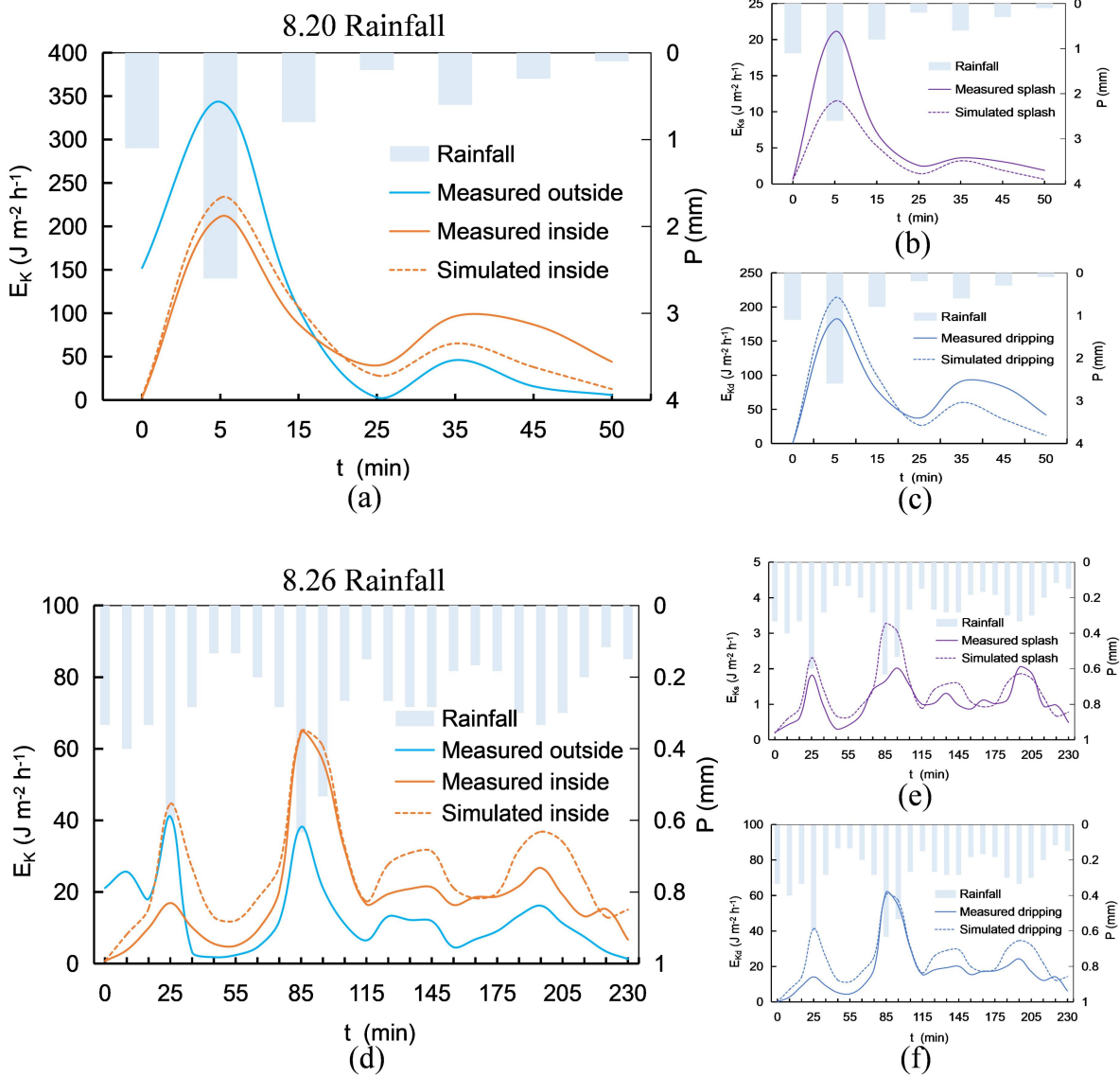
285 Figure 5. Comparison of kinetic energy of rainfall outside the canopy during two rainfall events (a) 8.20 total kinetic energy of rainfall (b) 8.20 kinetic energy of splashing drops under the canopy (c) 8.20 kinetic energy of dripping drops under the canopy (d) 8.26 total kinetic energy of rainfall (e) 8.26 kinetic energy of splashing drops under the canopy (f) 8.26 kinetic energy of dripping drops under the canopy.
