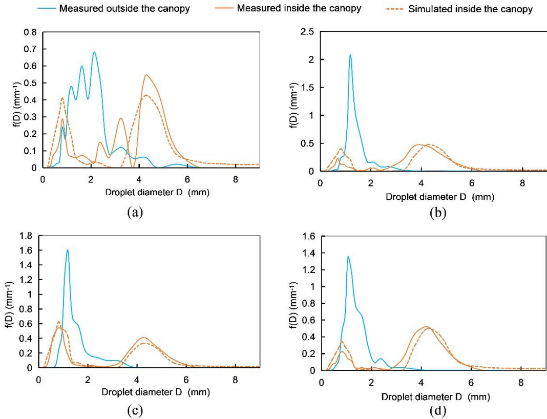
Figure 4. Comparison of raindrop spectra outside the canopy and inside the canopy during two rainfall events. f(D) is the volumetric drop-size distribution function (Volume fraction per millimeter ( \text{mm}^{-1} )), plotted based on the volume-based frequency. The total area under the entire curve is normalized to 1. (a) Raindrop spectrum of 0-10 min rainfall on 8.20 (b) Raindrop spectrum of 30-40 min rainfall on 8.20 (c) Raindrop spectrum of 0-10 min rainfall on 8.26 (d) Raindrop spectrum of 150-160 min rainfall on 8.26. The OTT Parsivel 2 laser spectrometer uses a non-uniform binning scheme to represent drop size distributions. The full diameter range (0.0625-24.5 mm) is divided into 32 classes with variable bin widths: 0.125 mm for D < 1.25 mm, 0.25 mm for 1.25-2.5 mm, 0.5 mm for 2.5-5.0 mm, and 1.0 mm for D > 5.0 mm. The figure is plotted using the midpoint of each bin as the representative value.
