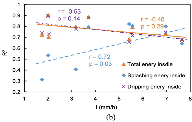
Figure 7. Sensitivity Analysis Between Model Metric R^2 and External Influencing Factors: (a) Wind Speed, (b) Rainfall Intensity. r is Correlation coefficient, and p -value indicates the significance of the linear relationship from the t-test ( p < 0.05 is significant).
