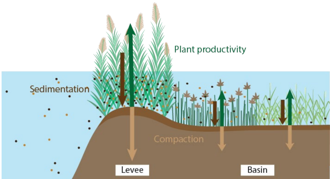
375 Figure 8: Conceptual overview of processes that likely contribute to the much higher organic carbon accumulation rate on levees compared to basins. Length of the arrows indicate the gradient in sedimentation (dark brown), compaction (light brown) and vegetation productivity (green).
