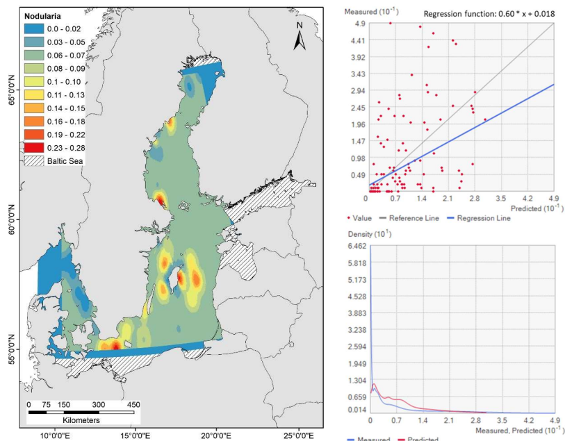
430 Figure 5: Spatial prediction map of Co-kriging interpolation (left) and distributions of the cross-validation statistics (right), estimated using kernel density, show the prediction regression scatterplot, the regression function of the concentration and predicted area distribution of nodularin ( \mu\text{g l}^{-1} ) at different sampling sites across the Baltic Sea. Grading colors in key legend corresponds to predicted concentrations of nodularin ( \mu\text{g l}^{-1} ). The blue and red lines correspond to the measured and predicted values of nodularin ( \mu\text{g l}^{-1} ). Predicted area distribution and concentrations of nodularin are based on the measured abundances of Nodularia spumigena .
