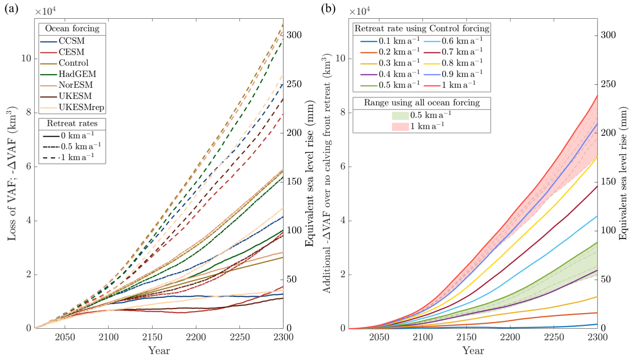
Figure 3. (a) -\Delta\text{VAF} for all RR0, RR0.5 and RR1 experiments. (b) -\Delta\text{VAF}_{\text{add}} for all retreat rates using Control forcing, along with -\Delta\text{VAF}_{\text{add}} for all RR0.5 and RR1 experiments with the range at each retreat rate shaded.
