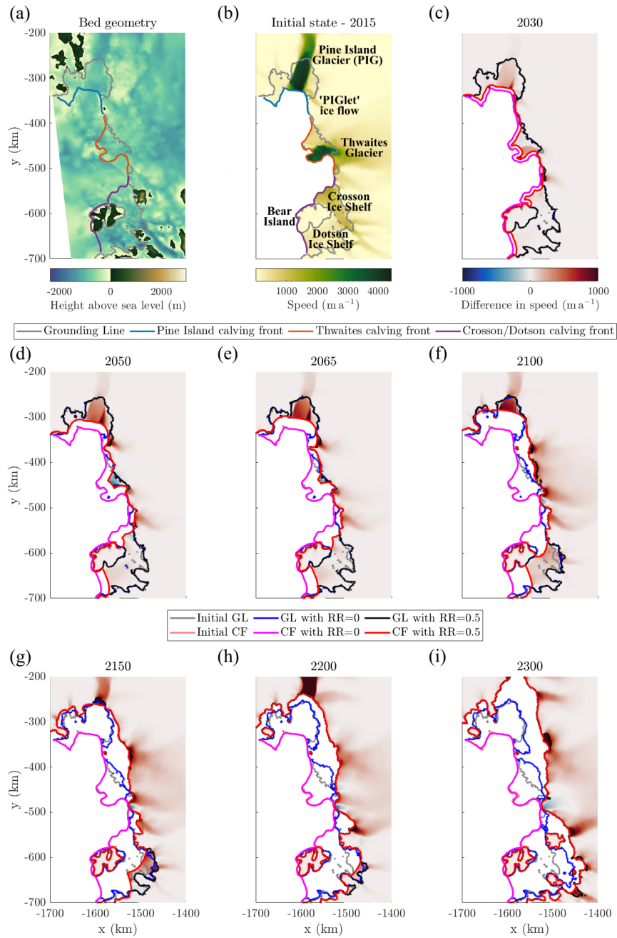
Figure 1. (a) The bed geometry from BedMachine. (b) The initial speed, grounding line and calving fronts, indicating which parts of the calving front are counted with each catchment region in our discussion. (c-i) Snapshots of differences in ice speed between Control_RR0.5 and Control_RR0 at different years of the simulation. Videos of the Control_RR0 experiment and the differences in ice speed and thickness above flotation for Control_RR0.5 (this figure) and Control_RR1 when compared to it are available as supplementary files.
