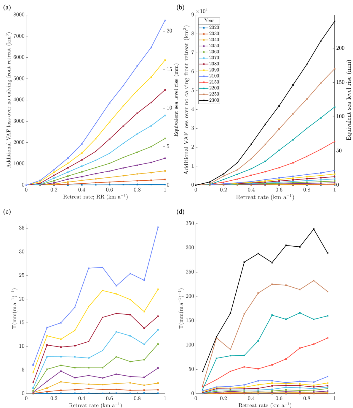
Figure 2. (a-b) The relationship between the retreat rate and -\Delta\text{VAF}_{\text{add}} for the Control forcing. (c-d) The values of \Upsilon calculated at each 0.1 \text{ km a}^{-1} step. In all cases, each line represents a specific year during the simulations. (a,c) Years up to 2100. (b,d) Years up to 2300.
