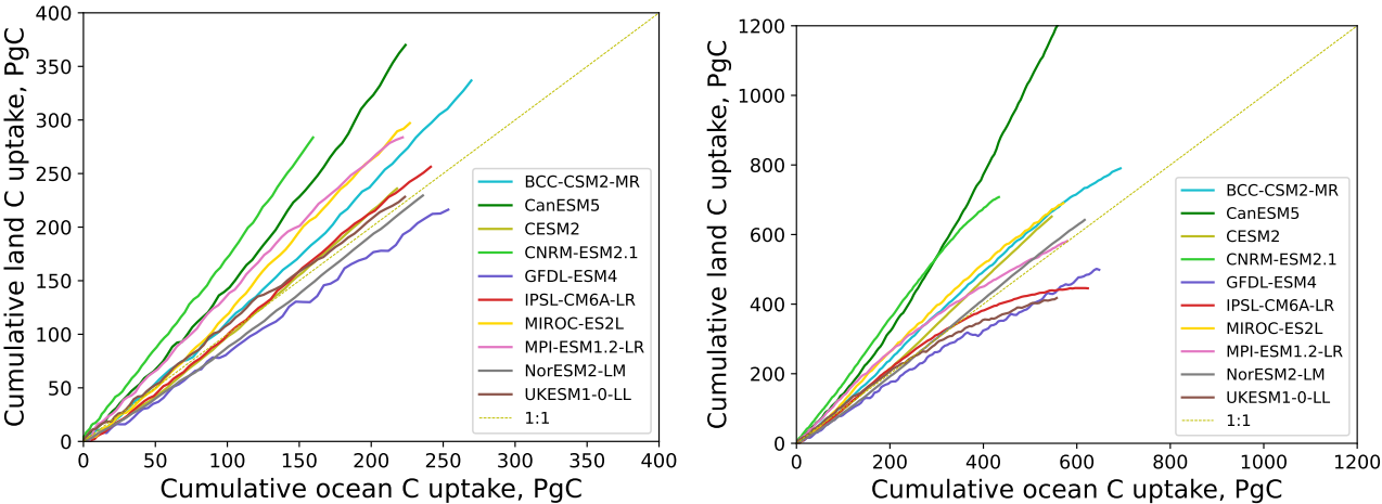
Figure A1. Cumulative land vs cumulative ocean carbon uptake in the C4MIP experiments for up to 2xCO 2 (left) and up to 4xCO 2 levels (right), data from Arora et al. (2020)
