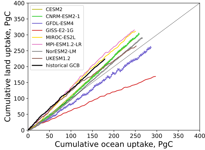
Figure 1. Cumulative land vs ocean carbon uptakes in the flat10 experiments for the first 100 years. Historical land vs ocean carbon sinks provided by in the Global Carbon Project Budget (GCB) (Friedlingstein et al., 2023) for the period 1850-2022 are shown by continuous black line. Note that The land fluxes do not account for sink in GCB is calculated from simulations in which \text{CO}_2 and climate evolved over the historical period, while the land cover stayed at its pre-industrial level (no land use changes). The thin dash line is the 1:1 ratio.
