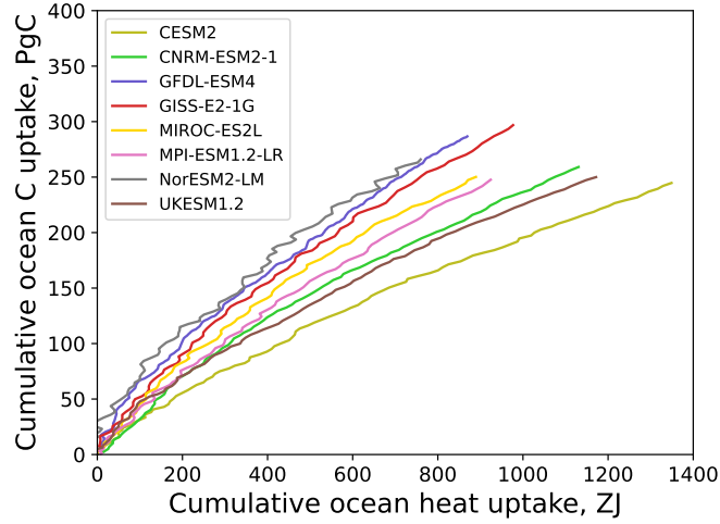
Figure 2. Analogous to Figure 1 Changes in cumulative ocean carbon (PgC) and heat uptakes (Zeta Joules) in the flat10 experiments.
