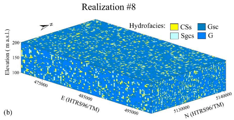
305 Figure 5. T-PROGS results in MA1: (a) Entropy factors in the vertical direction generated by a Markov chain model from borehole logs - diagonal boxes represent unobservable auto-transitions, gray boxes display values computed for the background material; (b) the representative stochastic hydrofacies model of the Varaždin aquifer (vertical exaggeration is 50-fold).
