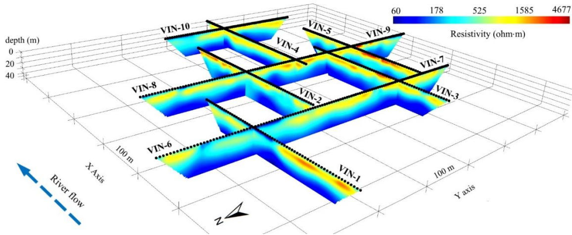
225 Figure 3. Pseudo 3D ERT model for the 10 profiles measured in the Vinokovščak wellfield.
