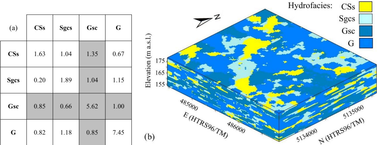
335 Figure 7. T-PROGS results in MA2: (a) Entropy factors in the vertical direction generated by a Markov chain model from borehole logs; (b) one of the geostatistical realizations of the spatial distribution of hydrofacies in the Vinokovščak wellfield area, constructed using ERT-derived lens lengths with a grid resolution of 20x20x1 m (vertical exaggeration is 20-fold).
