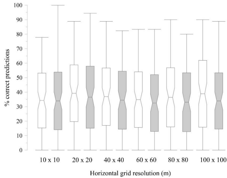
345 Figure 8. Comparison of prediction accuracy of models in the Vinokovščak area based on ERT-derived lens lengths (white box-whisker plots) and default lens lengths (gray plots) at different grid resolutions. Note: The edges of the box represent the standard deviation, the whiskers represent the minimum and maximum, and the central line represents the mean of the data.
