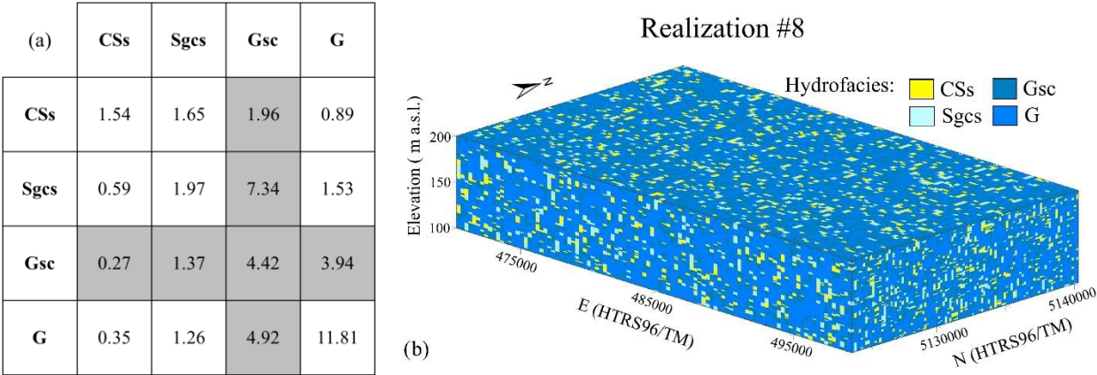
295 Figure 5. T-PROGS results in MA1: (a) Entropy factors in the vertical direction generated by a Markov chain model from borehole logs - diagonal boxes represent unobservable auto-transitions, gray boxes display values computed for the background material;(b) the representative stochastic hydrofacies model of the Varaždin aquifer (vertical exaggeration is 50-fold).
