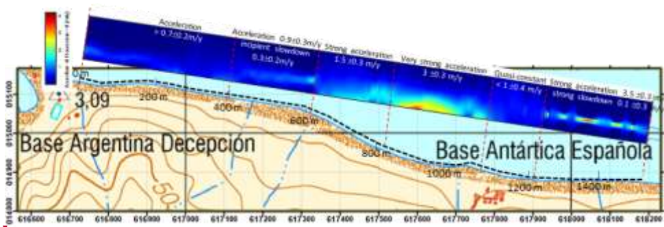
Figure 8. Distribution of the interpreted non-linear behaviour and short-term erosion trends (in m/year) with the best fitted model (SL4) in the six recognised sectors in which the study area has been segmented.
