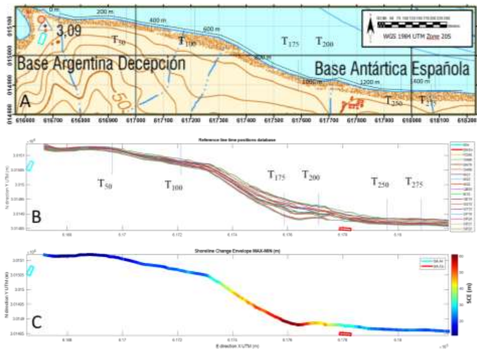
Figure 3. A) Detail in the study area marking the distances over the coastline measured from the western boundary and three of the control transects selected in this work (T50, T175 and T275). B) Catalogue of 16 polygonal lines extracted from the processing of the images in the study area and their discretisation into points with TBM (points on the polylines). C) Shoreline change envelope (SCE) between the first reference line (FIDASE 1956) and the last one (SAR PAZ 2022).
