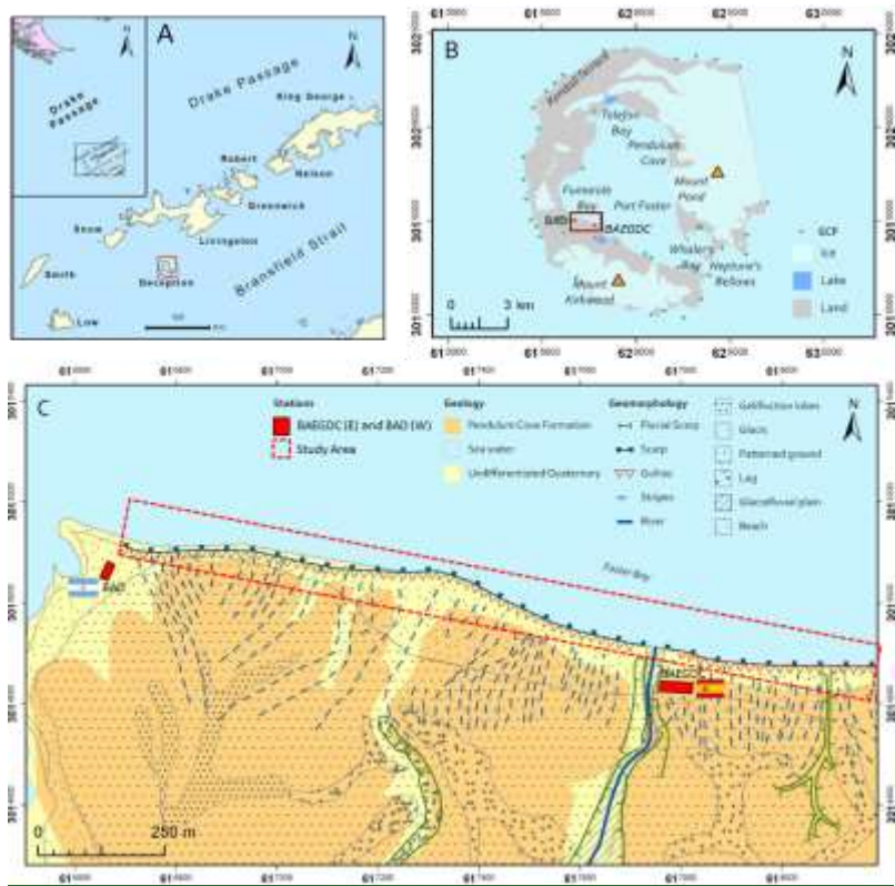
265 Figure 1. A) Location of study area at Deception Island (South Shetlands, Antarctica Maritime). B) Toponyms, scientific stations and main ice, water and land extents distribution. C) Detailed geomorphology of the cliffed coastal area between Argentinean (BAD) and Spanish (BAEGDC) scientific Antarctic stations in this study (modified from Geological Map of Deception Island in Smellie, 2002, Geomorphological Map of Deception Island in Goyanes, 2015, and de Pablo et al., 2017). Coordinate system UTM WGS84, zone 20S, EPSG:32720.
