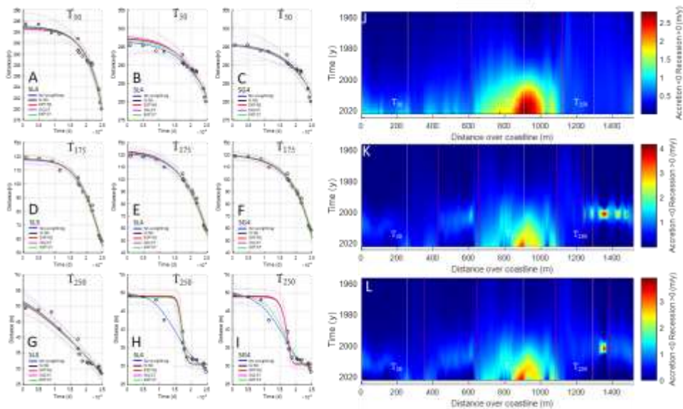
Figure 6. A) to J) Sigmoidal regression results from SL3, SL4 and SG4 models to distance vs. time (days since FD56) at control transects 50, 175 and 250 (solid curves) with their 95% prediction intervals across the fit range (dotted curves around each sigmoidal model), applying the four weighting schemes considered in this work (Table 4) and without weighting. Instantaneous rate of change R(t) space-time map (in m/y) fitted with the J) SL3, K) SL4 and L) SG4, with weighting EXP-ST, along the time interval [1956, 2022] for each i^{\text{th}} transect ( i=1..294 ) in the study area. The detected changes in R(t) dynamics, along the study area, are marked with red dashed lines on each map, see their explanation in the main text.
