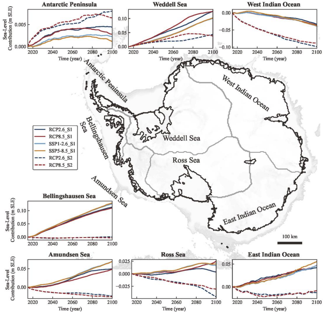
335 Figure 10: The mean contribution of the AIS seven sectors to sea-level rise from 2015 to 2100 (m SLE). The solid and dashed lines represent projections from the S1 and S2 initial states, respectively, under different climate scenarios, with the S2 predicted results being part of the LOW21 ensemble projections (red for RCP 8.5, blue for RCP 2.6).
