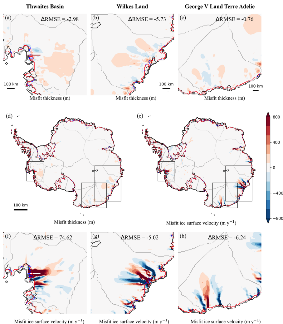
Figure 6: Comparison of spin-up ice thickness and velocity misfits between S1 and S2. (a–c) Ice thickness differences (S1 relative to S2) in the TB, WL, and GVL, respectively. (f–h) Ice surface velocity misfits in the TB, WL, and GVL, respectively. The difference in root mean square error ( \Delta\text{RMSE} ) between S1 and S2, compared to observations ( \Delta\text{RMSE} = \text{RMSE}_{\text{S1}} - \text{RMSE}_{\text{S2}} ). (d) and (e) present the deviations in ice thickness and surface velocity between two experiments, with three black boxes highlighting regions showing the most significant discrepancies. Grounding lines: S2 (blue), S1 (red), and observed data (black) from BedMachine v.3 (Morlighem et al., 2019). The profile line locations corresponding to Fig. 8 are in Thwaites Glacier: (a), (d) brown; (f) white.
