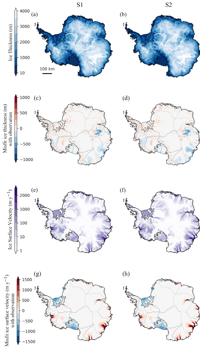
Figure 4: Comparing simulated initial state with observations. Modeled ice thickness (m) and surface ice velocity ( \text{m y}^{-1} ) at the end of spin-up. The left column shows ice thickness and ice surface velocity results from S1, alongside their difference from observation (Morlighem et al., 2019; Mouginot et al., 2019). The right column shows the corresponding results from S2, sharing common color bars with S1.
