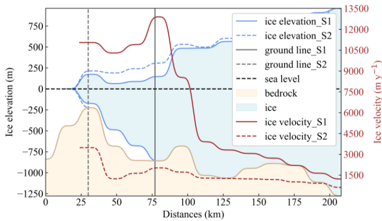
Figure 78: Comparison between S1 and S2 along the Thwaites Basin transect after spin-up. Ice elevation (blue line), ice surface velocity (brown line), and grounding-line positions for S1 and S2 are indicated by the grey solid and dashed lines, respectively. Sea level: black dashed line.
