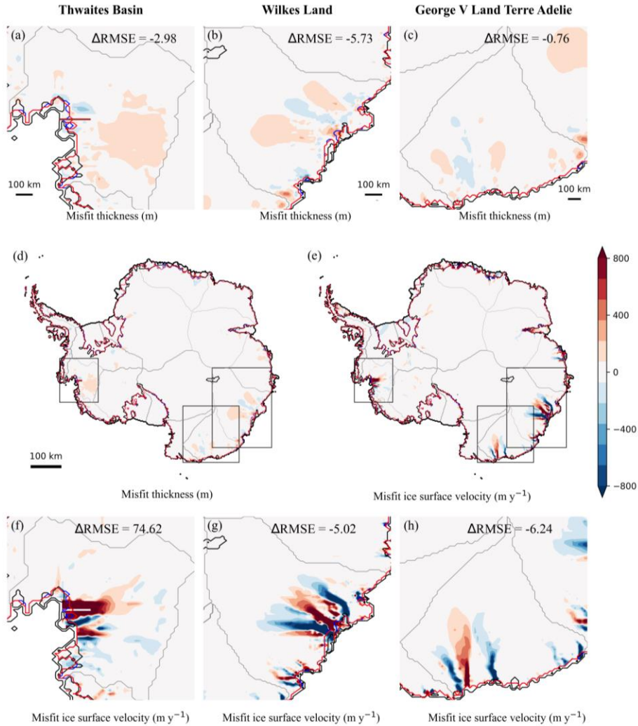
225 Figure 56: Comparison of spin-up ice thickness and velocity misfits between S1 and S2. (a–c) Ice thickness differences (S1 relative to S2) in the TB, WL, and GVL, respectively. (f–h) Ice surface velocity misfits in the TB, WL, and GVL, respectively. The difference in root mean square error ( \Delta\text{RMSE} ) between S1 and S2, compared to observations ( \Delta\text{RMSE} = \text{RMSE}_{S1} - \text{RMSE}_{S2} ). (d) and (e) present the deviations in ice thickness and surface velocity between two experiments, with three black boxes highlighting regions showing the most significant discrepancies. Grounding lines: S2 (blue), S1 (red), and observed data (black) from BedMachine v.3 (Morlighem et al., 2019). The profile line locations corresponding to Fig. 78 are in Thwaites Glacier: (a), (d) brown; (f) white. 230
