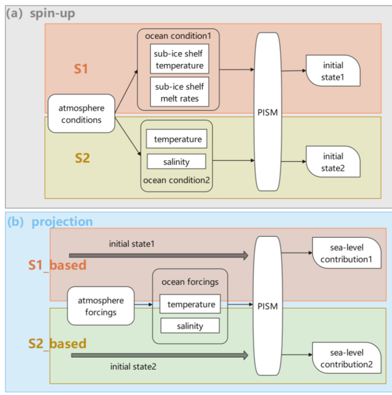
Figure 3: Overview of model initialization and projection processes. The schematic summarizes the model setup during (a) spin-up and (b) projection, using observed basal melt rates together with ice-shelf basal temperature (S1, orange box in a) and Southern Ocean temperature and salinity (S2, yellow box in a; LOW21). The projections initialized from these two states are denoted as S1-based and S2-based (LOW21), respectively.
