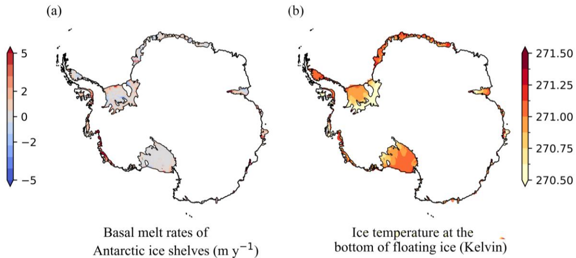
Figure 1: Ocean conditions used in S1. (a) observation of sub-ice shelf basal melt rates ( Rignot et al., 2013 ); (b) Temperature field beneath ice shelves ( Chambers et al., 2021 ).
