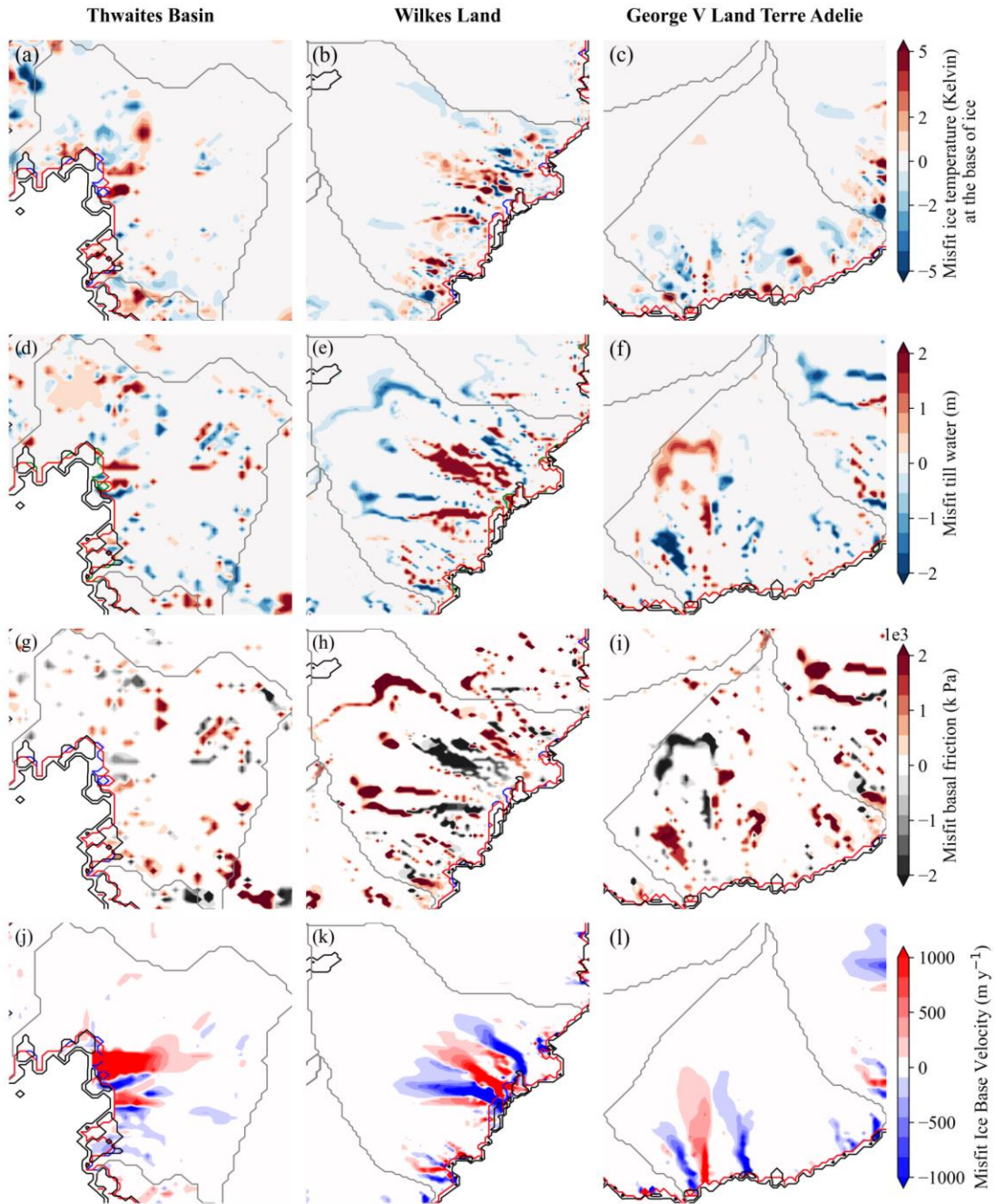
Figure 67: Spatial distribution of misfits (S1 relative to S2) in basal ice temperature field (Kelvin) (a-c), basal till water content (m) (d-f), basal friction (k Pa) (g-i), and basal velocity ( \text{m y}^{-1} ) (j-l) in the three basins. The blue and red lines indicate the grounding-line positions for S2 and S1, respectively, while the black line represents the observed grounding line from BedMachine v.3.
