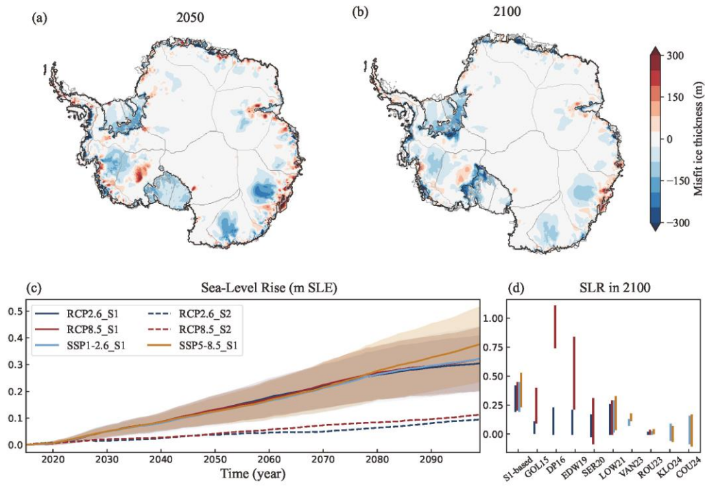
Figure 89: Ice sheet thickness misfits and projected contribution of the AIS to sea-level rise (m SLE). Spatial differences in the projected mean ice thickness between the multi-scenario (RCP 2.6 and RCP 8.5) ensemble means based on S1 and S2 in 2050 (a) and 2100 (b). (c) Predicted sea-level rise for “SGO scenario” to “SGF scenario” simulations under four scenarios (color shading) and mean values (color lines). The dashed lines represent projections from the S2 initial state—a set of results from the LOW21 ensemble projections: red for RCP 8.5, blue for RCP 2.6. (d) Projected contributions to sea-level rise (SLR) by 2100 based on S1, compared to other studies: CHU13 (Church et al., 2013), GOL15 (Golledge et al., 2015), DP16 (DeConto & Pollard, 2016), EDW19 (Edwards et al., 2019), SER20 (Seroussi et al., 2020), LOW21 (Lowry et al., 2021), VAN23 (van der Linden et al., 2023), KLO24 (Klose et al., 2024), and COU24 (Coulon et al., 2024).
