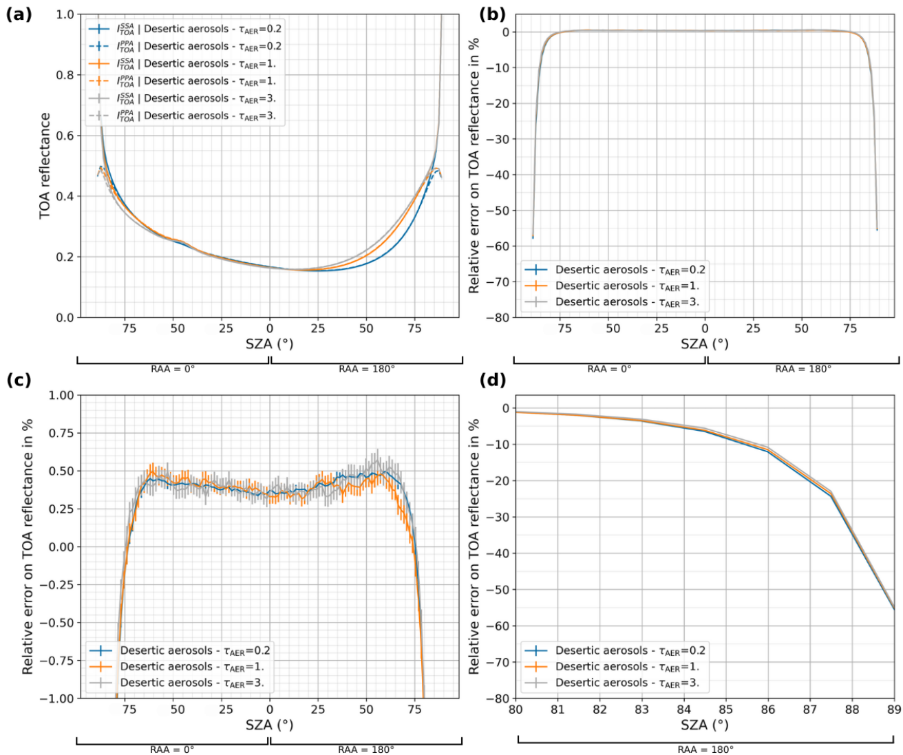
Figure 11. Comparison of PPA and SSA simulations for several AOD values as a function of SZA, for channel VIS 0.4 in a US standard atmosphere with a Lambertian surface of albedo 0.1, with VZA = 45° in the principal relative azimuthal plane, with 1e8 photons. (a) Simulated TOA reflectances. (b) Calculated relative error between PPA and SSA simulated TOA reflectances. (c) Same plot zoomed-in between -1 % and 1 %. (d) Same plot zoomed-in for SZA over 80°.
