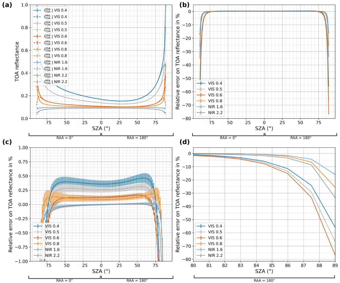
Figure 4. Comparison of PPA and SSA simulations for several FCI VIS and NIR spectral channels as a function of SZA, with \text{VZA} = 45^\circ in a US standard aerosol-free atmosphere with a Lambertian surface of albedo 0.1, in the principal relative azimuthal plane, with 1e7 photons. (a) Simulated TOA reflectances. (b) Calculated relative error between PPA and SSA simulated TOA reflectances. (c) Same plot zoomed-in between -1 % and 1 %. (d) Same plot zoomed-in for SZA over 80^\circ .
