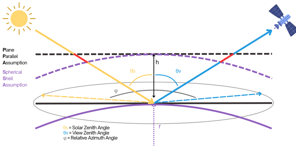
Figure 1. Schematic diagram of the PPA and SSA geometries, highlighting the optical path error (in red color). h is the height-altitude of the atmosphere, r is the Earth radius, \theta_s is the solar zenith angle, \theta_v is the view zenith angle and \varphi is the relative azimuth angle.
