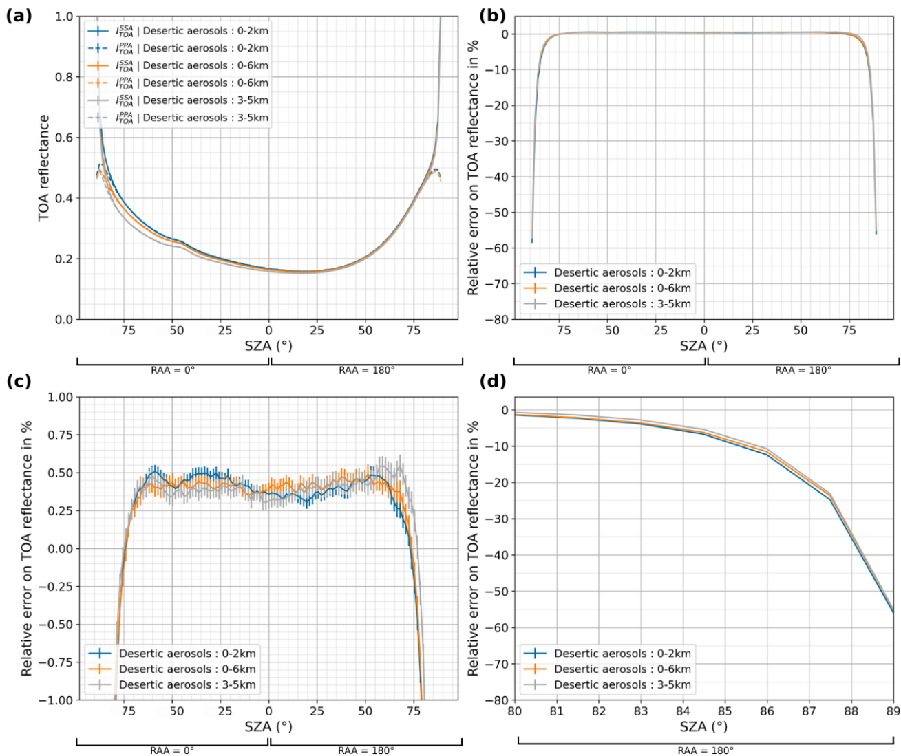
Figure 10. Comparison of PPA and SSA simulations for aerosol layers of different altitudes as a function of SZA, for channel VIS 0.4 in a US standard atmosphere with a Lambertian surface of albedo 0.1, in the principal relative azimuthal plane, with 1e8 photons. (a) Simulated TOA reflectances. (b) Calculated relative error between PPA and SSA simulated TOA reflectances. (c) Same plot between -1% and 1%. (d) Same plot but for SZA over 80^\circ .
