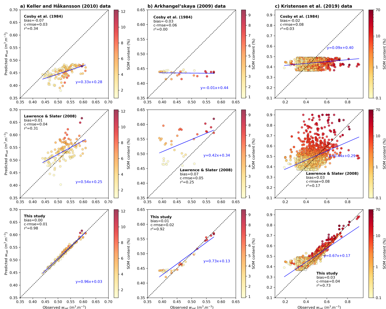
Figure 4. Comparison of observed and predicted soil porosity across three in situ datasets: (a) Keller and Håkansson (2010), (b) Arkhangel'skaya (2009), and (c) Kristensen et al. (2019). Each row corresponds to a different prediction method: the first row uses the mineral-soil PTF of Cosby et al. (1984), which ignores the presence of organic matter; the second row applies the method of Lawrence and Slater (2008), which includes SOM effects using a simplified approach; and the third row shows results from the process-based framework developed in this study. The 1:1 line is shown in black, and the blue line represents the linear regression between predicted and observed values where its slope and intercept provide an additional measure of agreement. Finally, skill scores are given for each panel.
