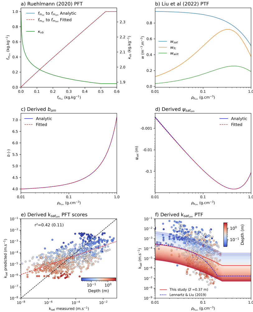
Figure 1. Derived hydrodynamic properties for SOM domain as a function of its apparent bulk density ( \rho_{b,om} ) for the Brooks and Corey (1964) model. (a) Conversion function from organic carbon fraction ( f_{m,oc} ) to organic matter fraction ( f_{m,om} ), shown in both analytic (blue) and fitted (red dashed) forms, using the Van Bemmelen factor ( \kappa_{vb} ) as described by the PTF of Ruehlmann (2020). (b) Volumetric water contents at saturation ( w_{sat} ), field capacity ( w_{fc} ), and wilting point ( w_{wilt} ) estimated with the PTFs of Liu et al. (2022). (c–d) Derived pore-size distribution index ( b_{om} ) and air-entry potential ( \psi_{sat,om} ) from analytical and fitted solutions. (e) Evaluation of the predicted saturated hydraulic conductivity ( k_{sat,om} ) against observed data from Morris et al. (2022), with points colored by depth. The coefficient of determination ( r^2 ) is shown for the current model, with the value obtained using the PTF of Lennartz and Liu (2019) indicated in parentheses for comparison. Black and red dashed lines are the 1:1 line and the best fit, respectively. (f) Predicted k_{sat,om} as a function of \rho_{b,om} and depth (shaded contours). The red line corresponds to the mean observed depth \bar{z} . Results are compared with the depth-independent PTF from Lennartz and Liu (2019). Observations are shown as points, colored by sampling depth.
