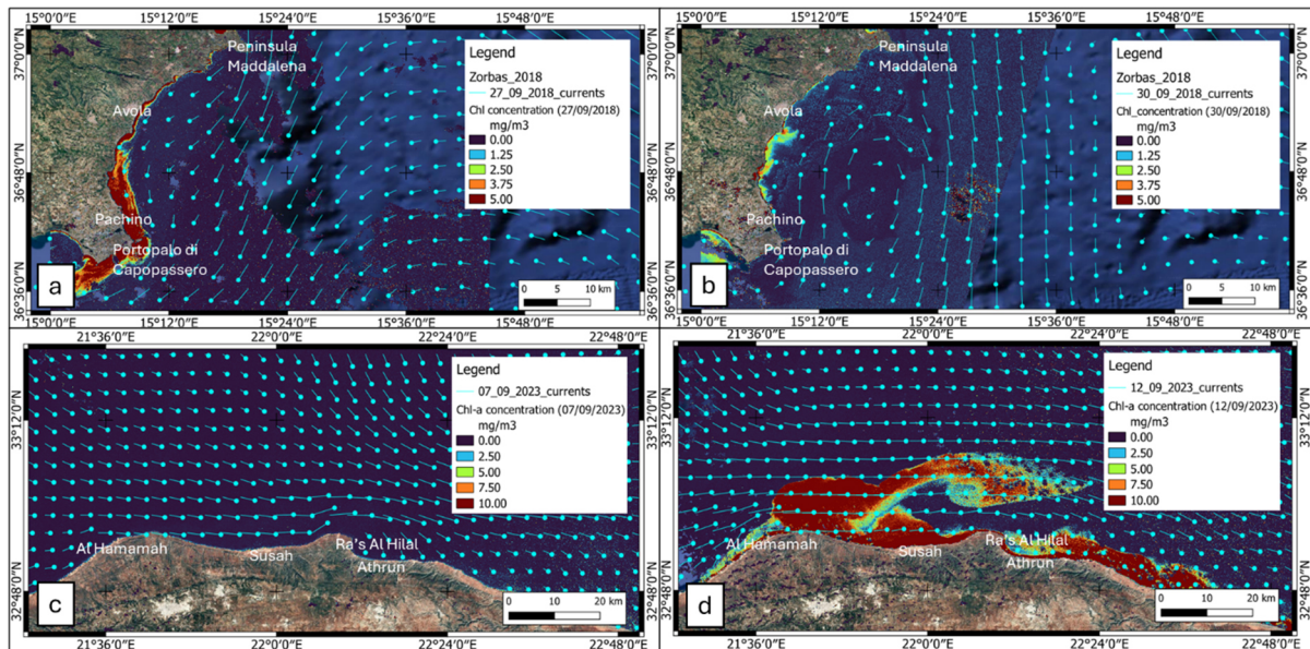
Figure 9. Surface changes of Chl-a assessed from Sentinel 2 MSI images with current vectors derived from Copernicus reanalysis (background maps provided by © Google Earth); a) Chl-a concentration off southeastern Sicily prior to the occurrence of medicane Zorbas (27 September 2018); b) Chl-a concentration after the impact of medicane Zorbas (30 September 2018); c) Chl-a concentration along the Libyan coasts prior to the occurrence of Daniel (07 September 2023); d) Chl-a concentration after the impact of Daniel (12 September 2023).
