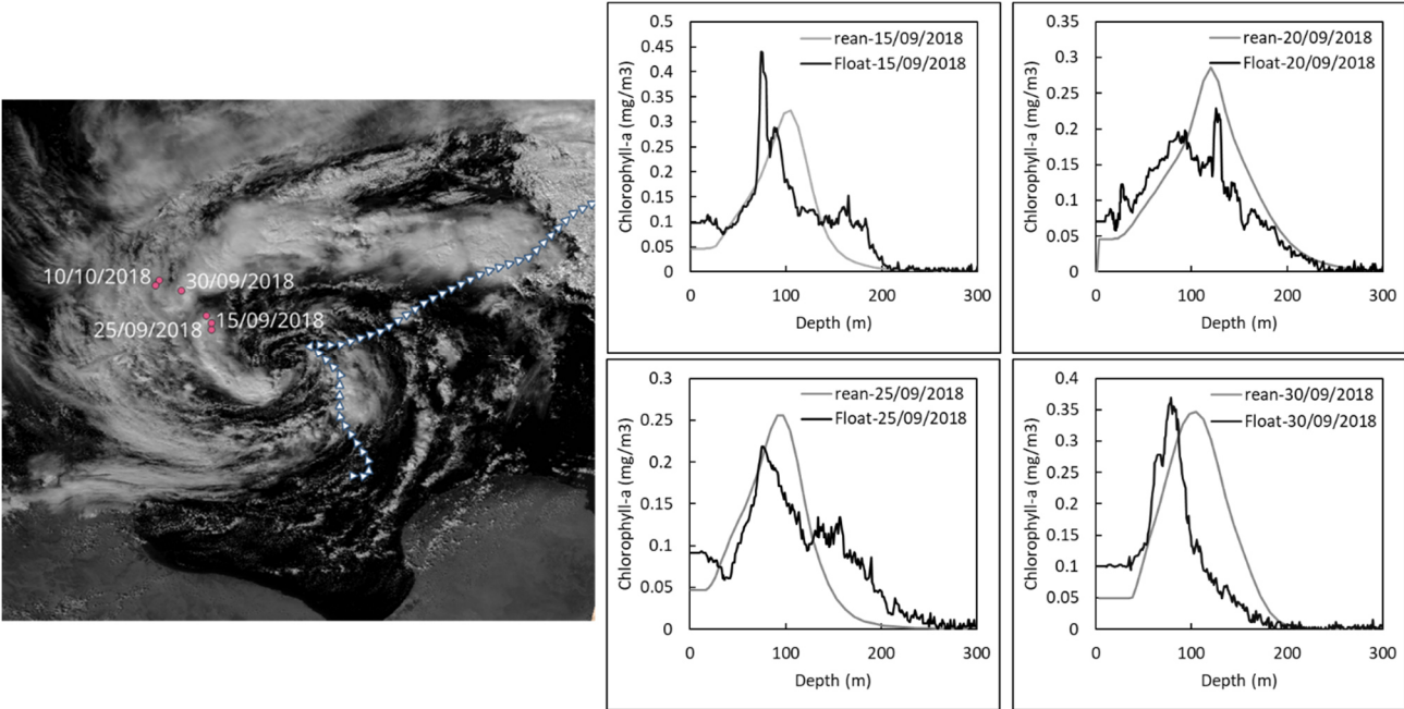
Figure 3. Comparison between reanalysis products (rean-date in the panels) and ARGO float data (float-date in the panels) for the medicane Zorbas occurred in the Ionian Sea; the Chl-a profiles from reanalysis were extracted in the same location as the float measurements.
