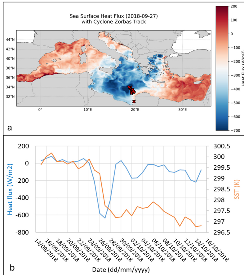
Figure 11. Decrease in heat fluxes and SST during the occurrence of medicane Zorbas; a) day of highest intensity of heat fluxes; b) time series of SST and surface heat fluxes extracted in the cyclogenesis location (0.04 x 0.04 degrees grid resolution).
