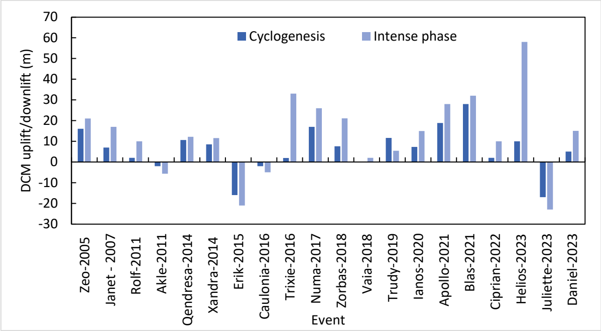
Figure 6. DCM uplift measured at the cyclone centres from the Copernicus reanalysis dataset, considering as temporal range the difference between 1 day prior to the cyclogenesis and 1 day after the cyclolysis (maximum total duration of 120 hours); different bars indicate different locations (blue for the cyclogenesis and light blue for the most intense phase locations).
