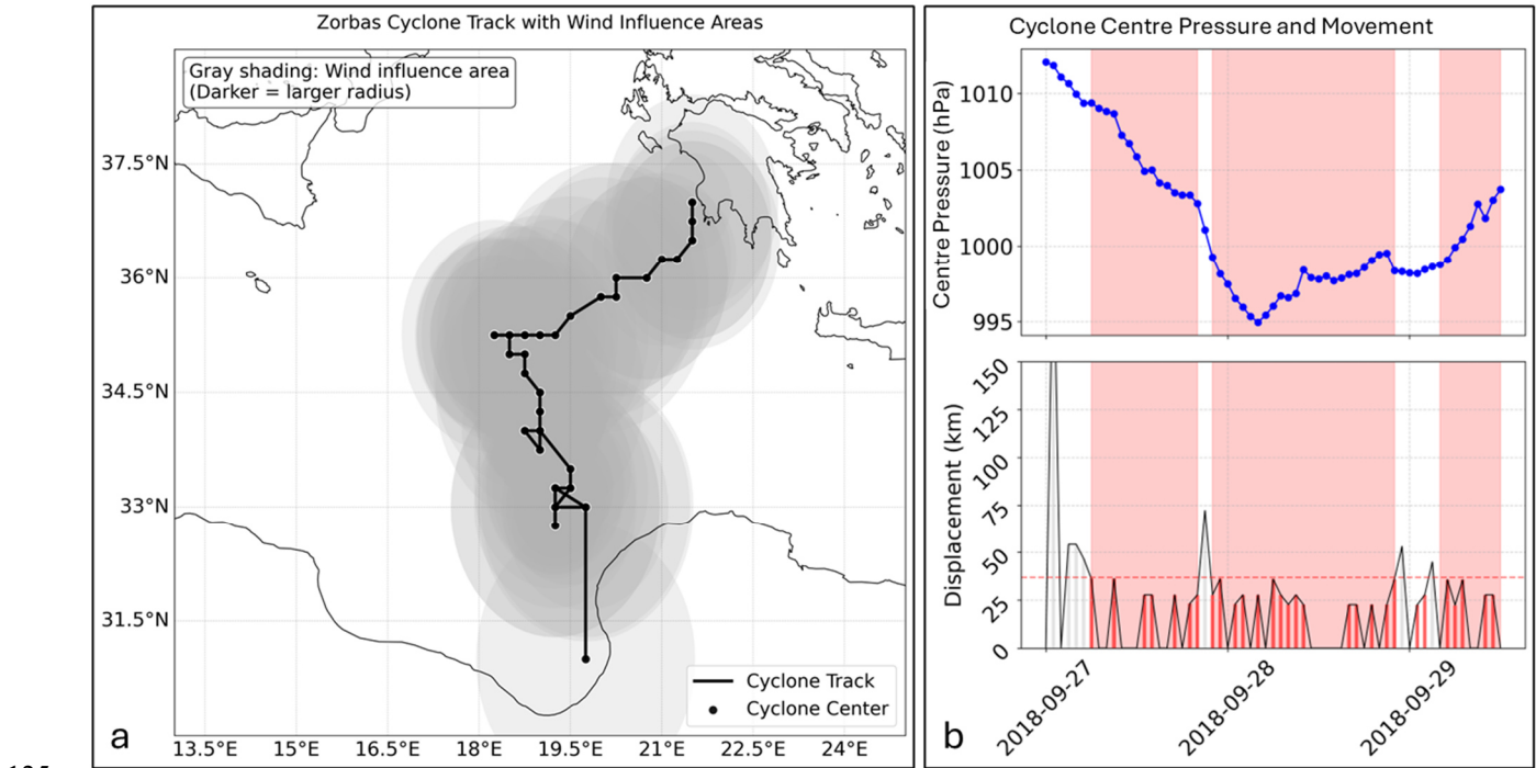
Figure 2. Assessment of the stationarity phase of a cyclone from MSLP data (case of medicane Zorbas); a) extraction of minimum MSLP point with value of centre (minimum) pressure and the maximum wind speed at 10 m height within a 200 km radius from the cyclone centre (gray shading areas); b) centre pressure along the cyclone track and displacements assessed across each minimum MSLP point, red bars indicate the displacement when it was shorter than 36 km in 4 hours, while shaded red areas indicate the long lasting slow-moving phases.
