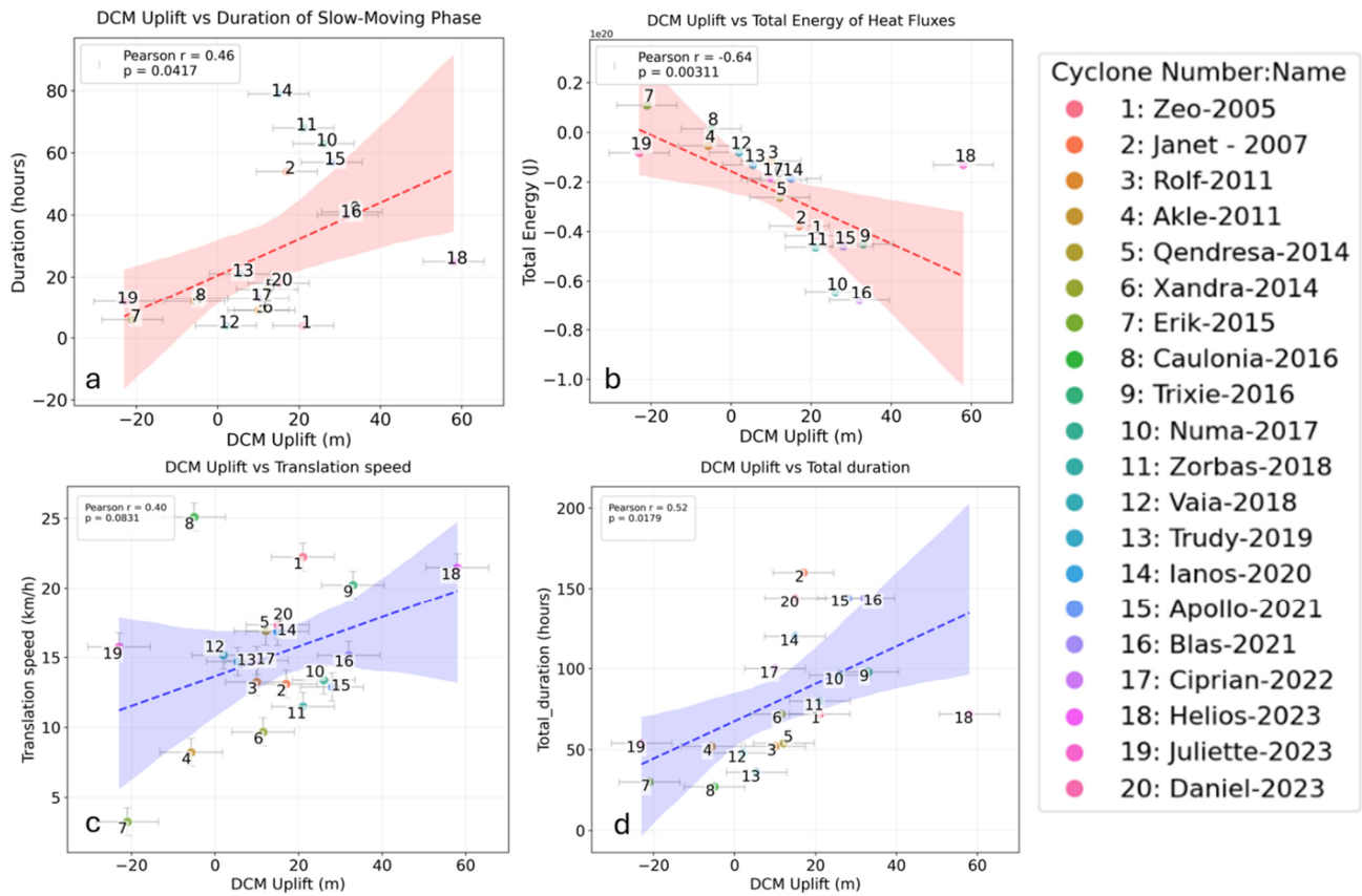
Figure 10 – Correlation between DCM uplift and duration and intensity of the Mediterranean cyclones; a) positive correlation between duration of slow-moving phases and DCM uplift; b) negative correlation between total energy lost by sea water and DCM uplift; c) correlation between translation speed assessed during slow-moving phase and DCM uplift; d) positive correlation between total duration of cyclones (including no-stationary phases) and DCM uplift.
