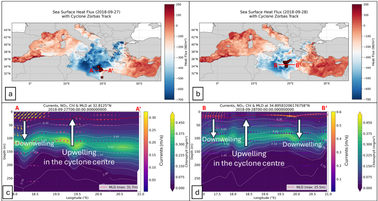
Figure 5. Heat fluxes and cross-section of biogeochemical variables during medicane Zorbas (27–29 September 2018); a–b) Heat fluxes maps assessed on 27/09/2018 and 28/09/2018, with cross-sections marked in red (x in red indicates the minimum MSLP value recorded on each date); c–d) Cross-sections showing: Chl-a concentration (viridis colormap), Nitrate concentration in \text{mmol/m}^3 (white contour lines), Current vectors (plasma-colored arrows), Mixed layer depth (MLD, red dashed line).
