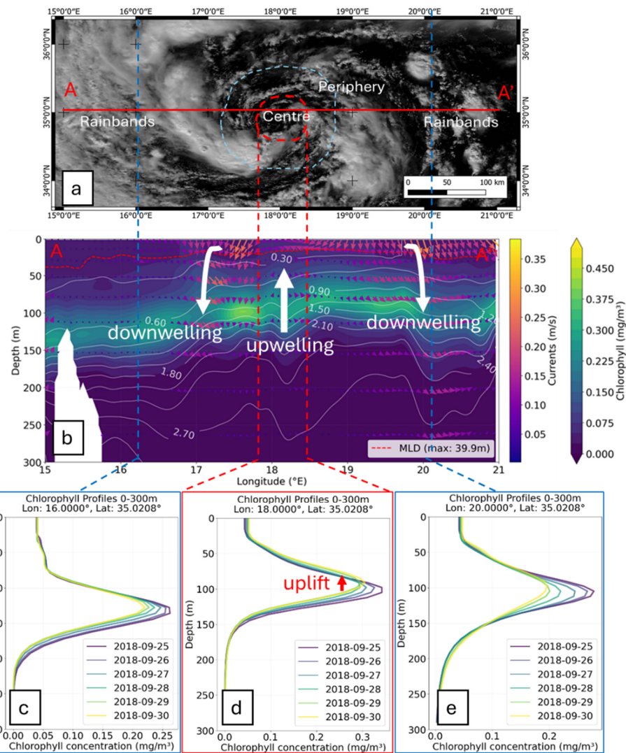
Figure 12. Features of Chl-a changes related to the structure of the medicane Zorbas; the cyclone centre highlighted the DCM uplift and upwelling, while periphery and rainbands display alternating downwelling and upwelling; a) satellite image of medicane Zorbas (MODIS image-acquired on 28 September 2018) highlighting the cyclone centre and periphery; b) cross-section of biogeochemical variables referred to the time of MODIS image showing: Chlorophyll-a concentration (viridis colormap), Nitrate concentration in mmol/m 3 (white contour lines), Current vectors (plasma-colored arrows), Mixed layer depth (MLD, red dashed line); c-d-e) changes in DCM assessed from Chl-a vertical profiles (note the DCM uplift in the cyclone centre).
