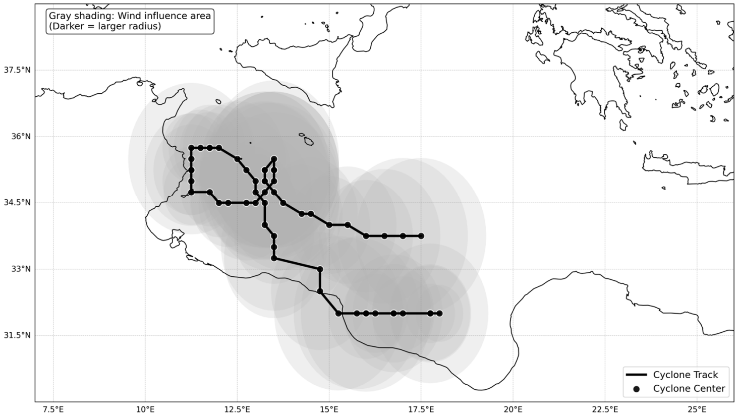
Zeo Cyclone Track with Wind Influence Areas
