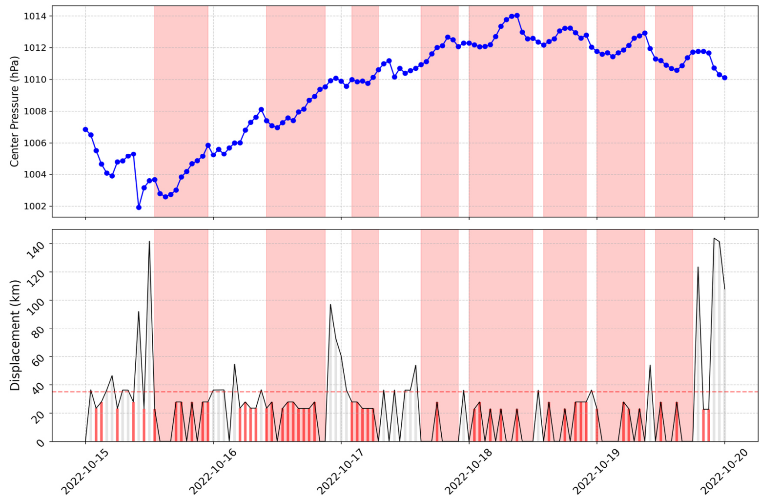
Cyclone Center Pressure and Movement
