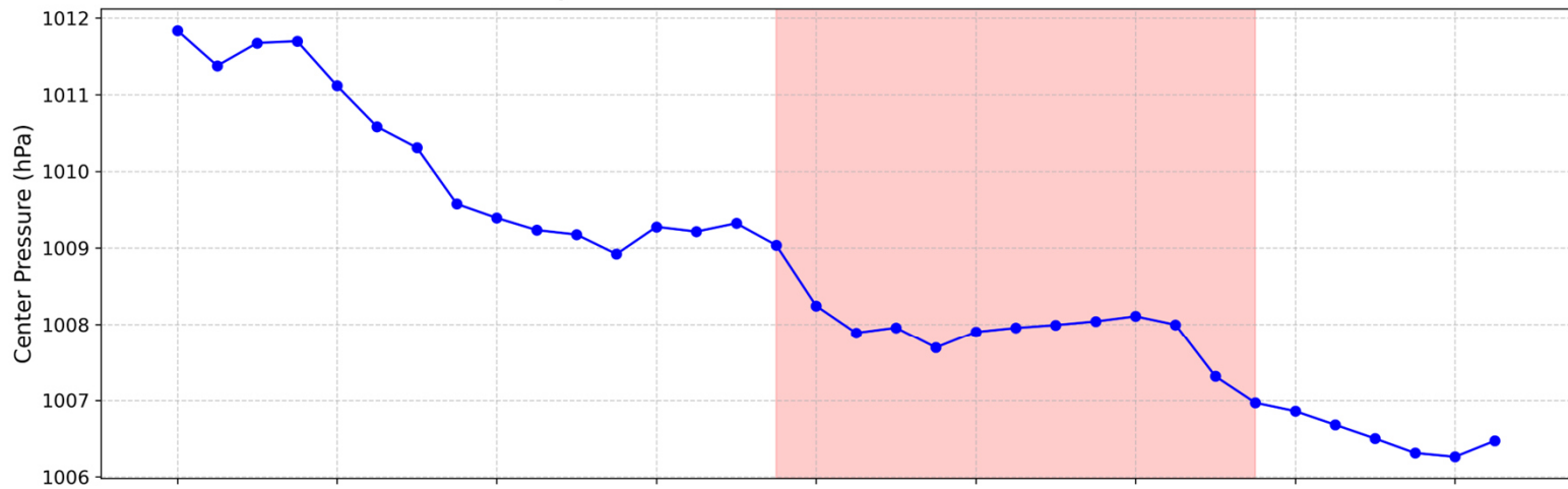
Cyclone Center Pressure and Movement
