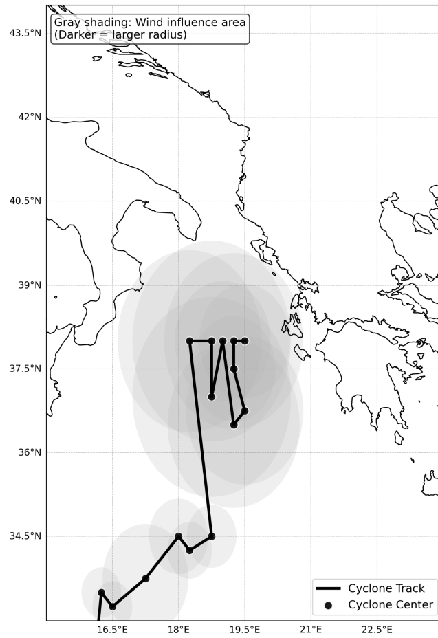
Cyclone Center Pressure and Movement
