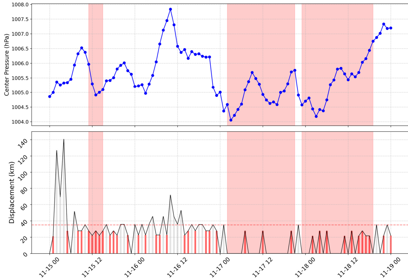
Cyclone Center Pressure and Movement
