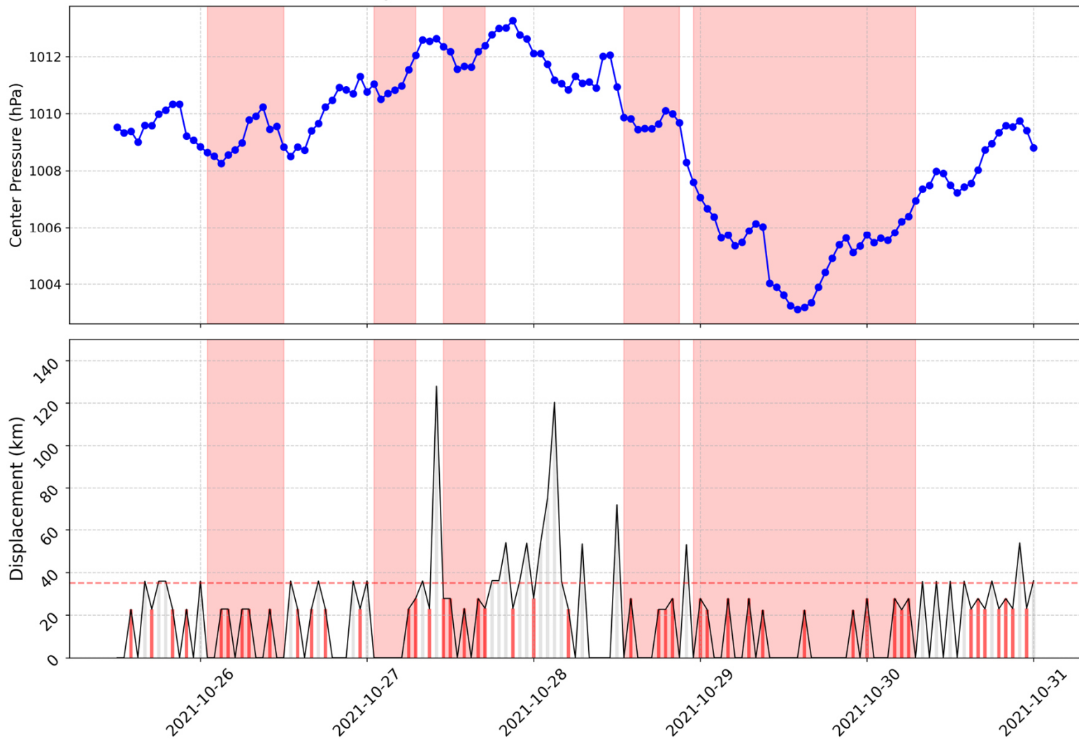
Cyclone Center Pressure and Movement
