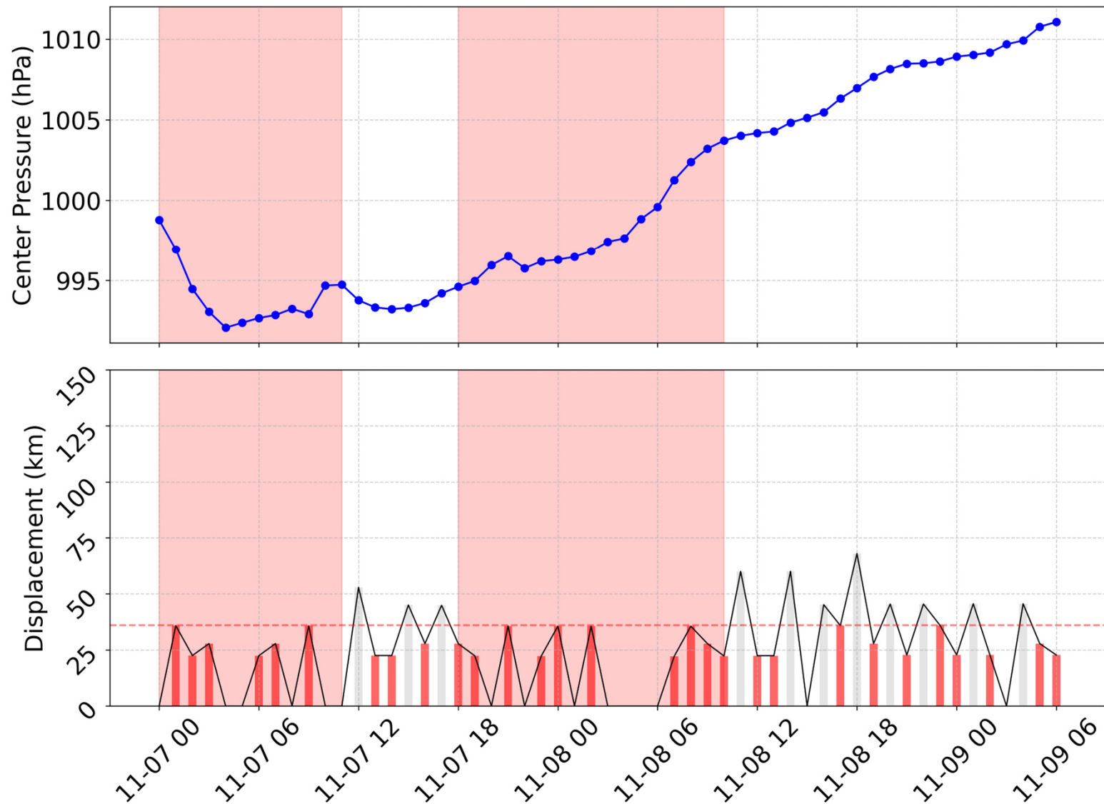
Cyclone Center Pressure and Movement
