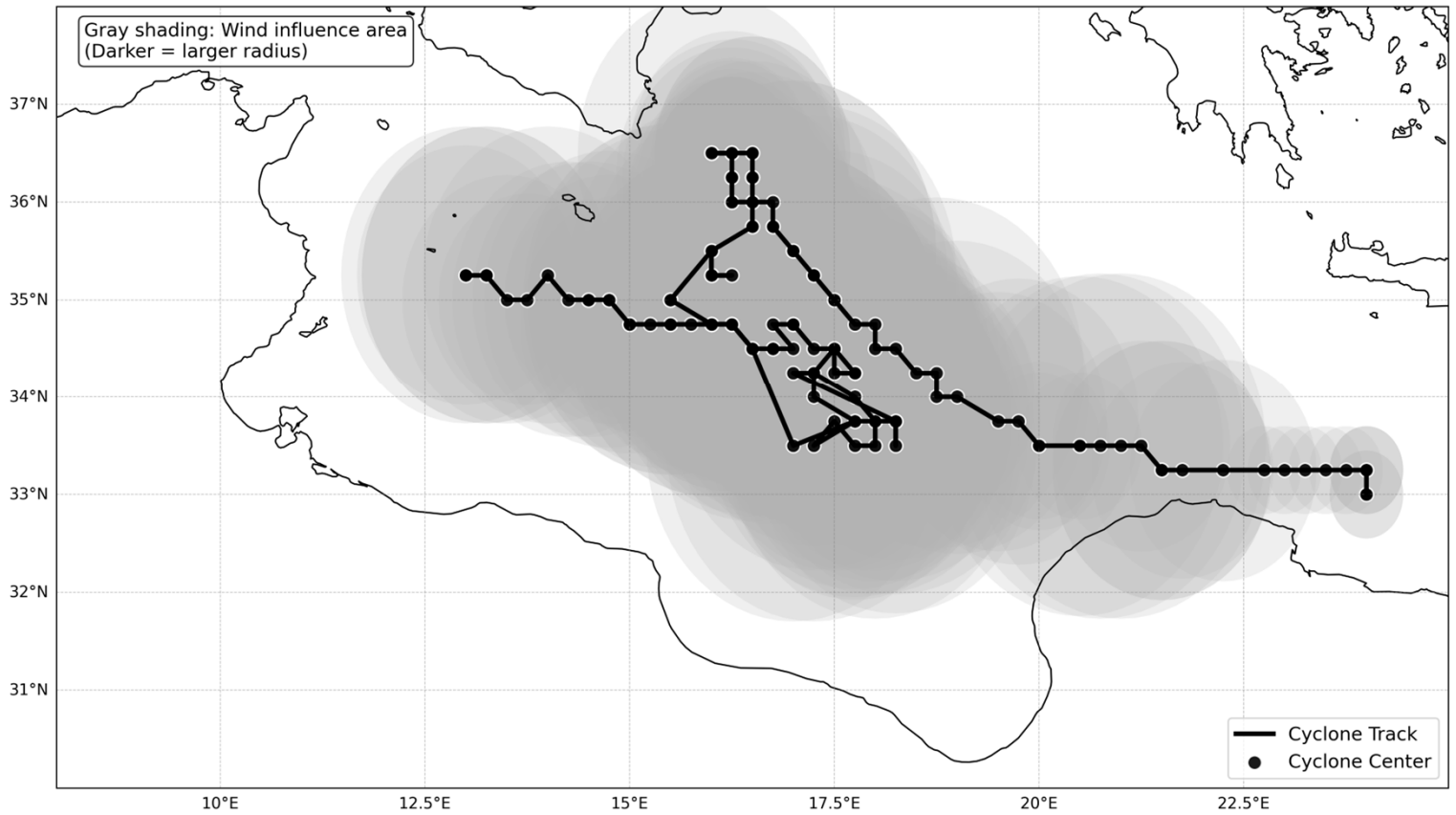
Apollo Cyclone Track with Wind Influence Areas
