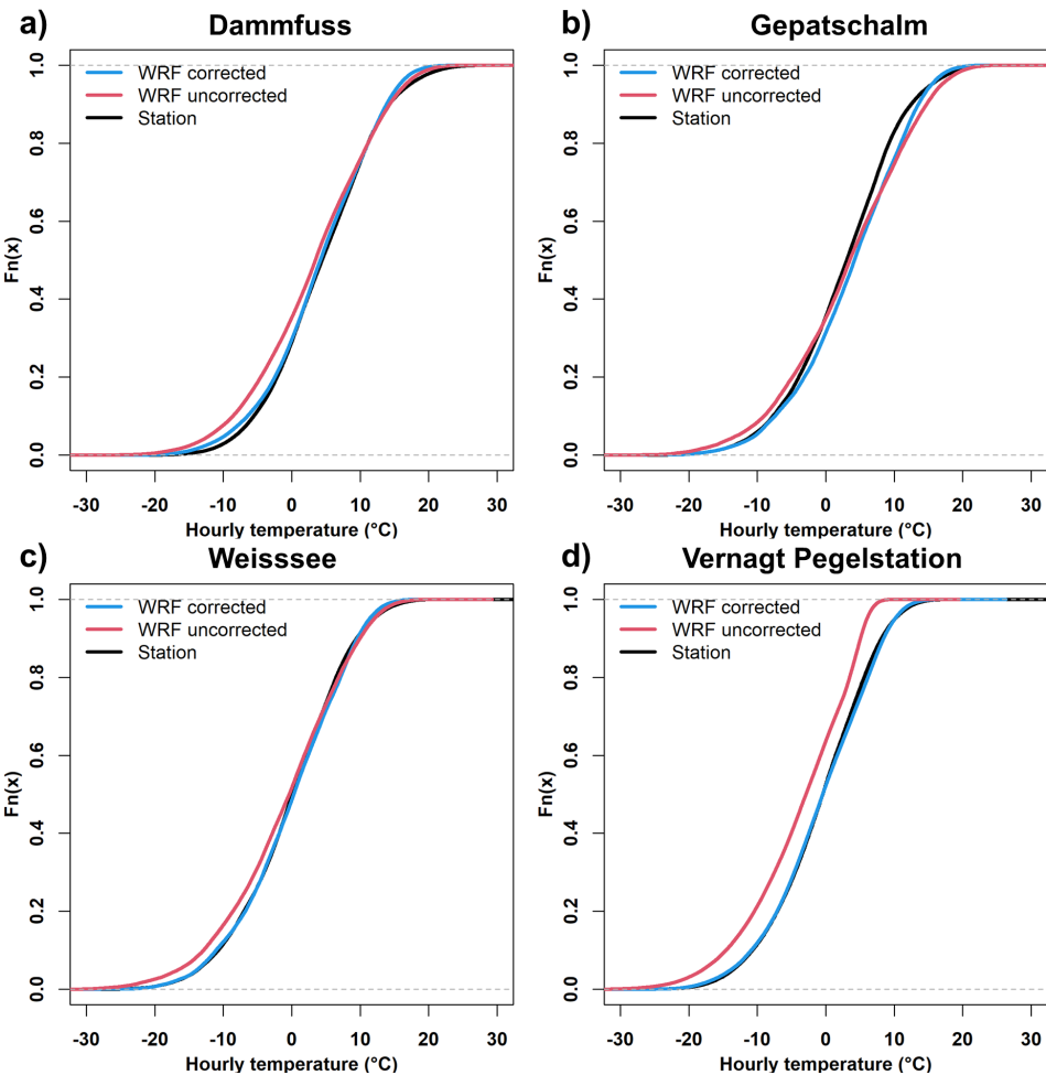
Figure 5. Empirical cumulative distribution functions (ECDF) of observed hourly temperature (black line), uncorrected WRF temperature (red line), and corrected WRF temperature (blue line) at different stations a) Dammfuss (WRF land use category Woodland Mosaic), b) Gepatschalm (WRF land use category Evergreen Needleleaf), c) Weisssee (WRF land use category Wooded Tundra), and d) Vernagt Pegelstation (WRF land use category Snow or Ice).
