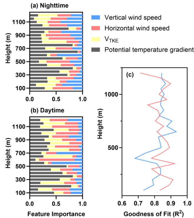
Figure 10. Results of feature importance analysis for the impacts of potential temperature gradient, mechanical turbulence, horizontal wind speed, and vertical wind speed on the UVPM gradient during a) nighttime and b) daytime, respectively. c) model goodness of fit (coefficients of determination, R^2 ) in the calculation.
