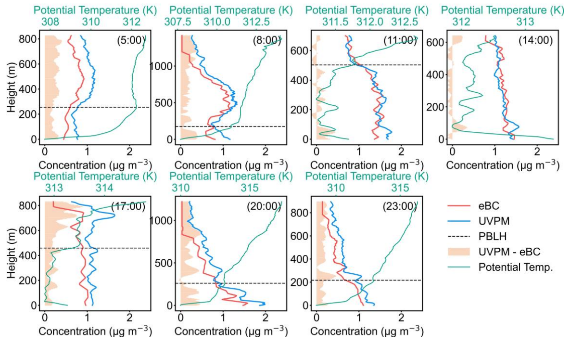
Figure 6. Diurnal variations in profiles of eBC, UVPM and potential temperature on July 27, 2024. The red line represents eBC, the blue line represents UVPM, and the green line
