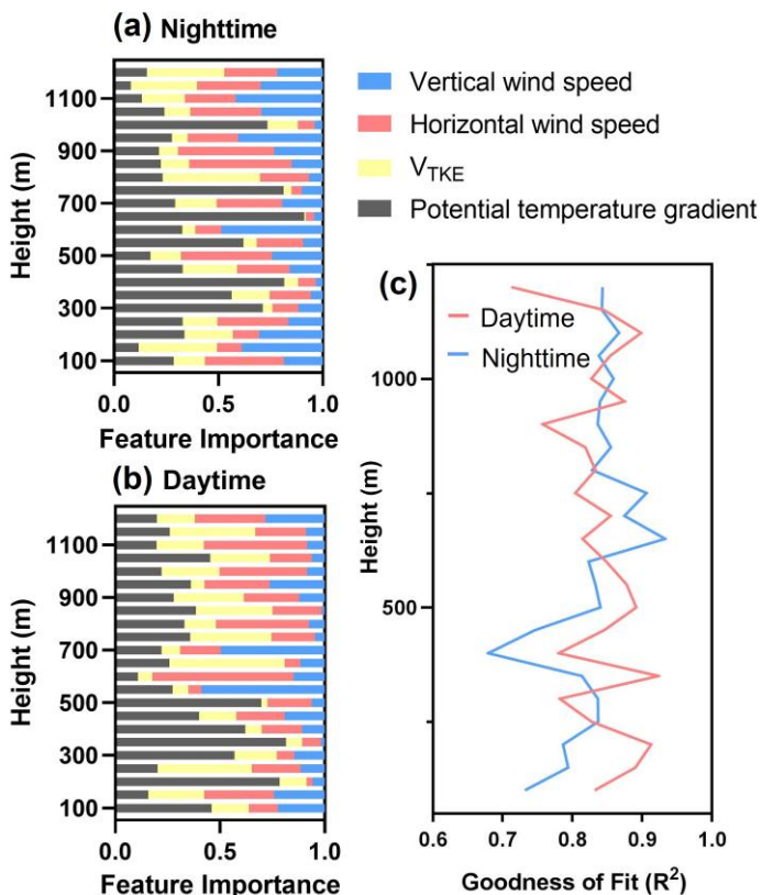
Figure 10. Results of feature importance analysis for the impacts of potential temperature gradient, mechanical turbulence, horizontal wind speed, and vertical wind speed on the UVPM gradient during a) nighttime and b) daytime, respectively. c) model goodness of fit (coefficients of determination, R^2 ) in the calculation.
