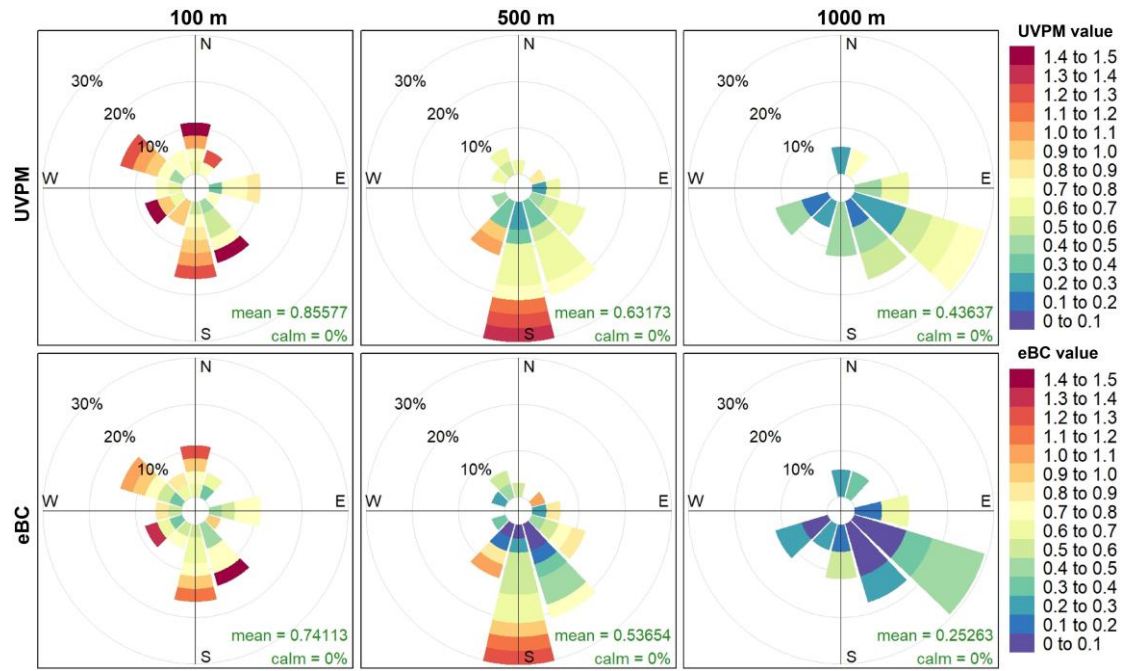
Figure 8. Conditional probability function (CPF) diagrams of the 90 th percentile of the UVPM and eBC concentrations with respect to wind speed and direction at the heights of 100 m, 500 m and 1000 m above ground level.
