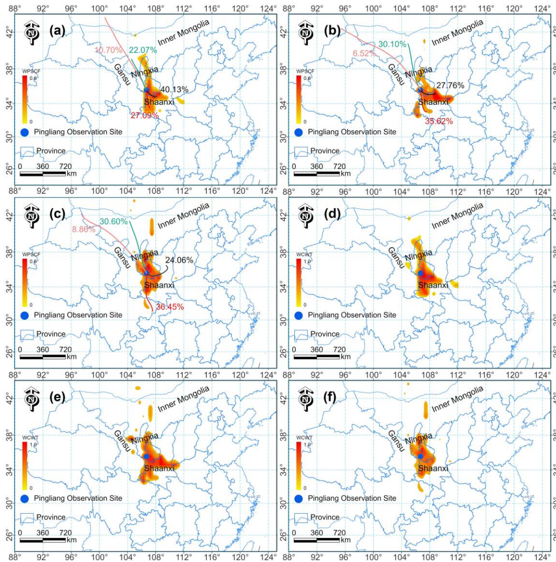
Figure 7. Backward trajectory clustering and WPSCF analysis results of air masses at heights of a) 100 m, b) 500 m, and c) 1000 m during the observation period, respectively. WCWT analysis results of air masses at heights of d) 100 m, e) 500 m, and f) 1000 m during the observation period, respectively.
