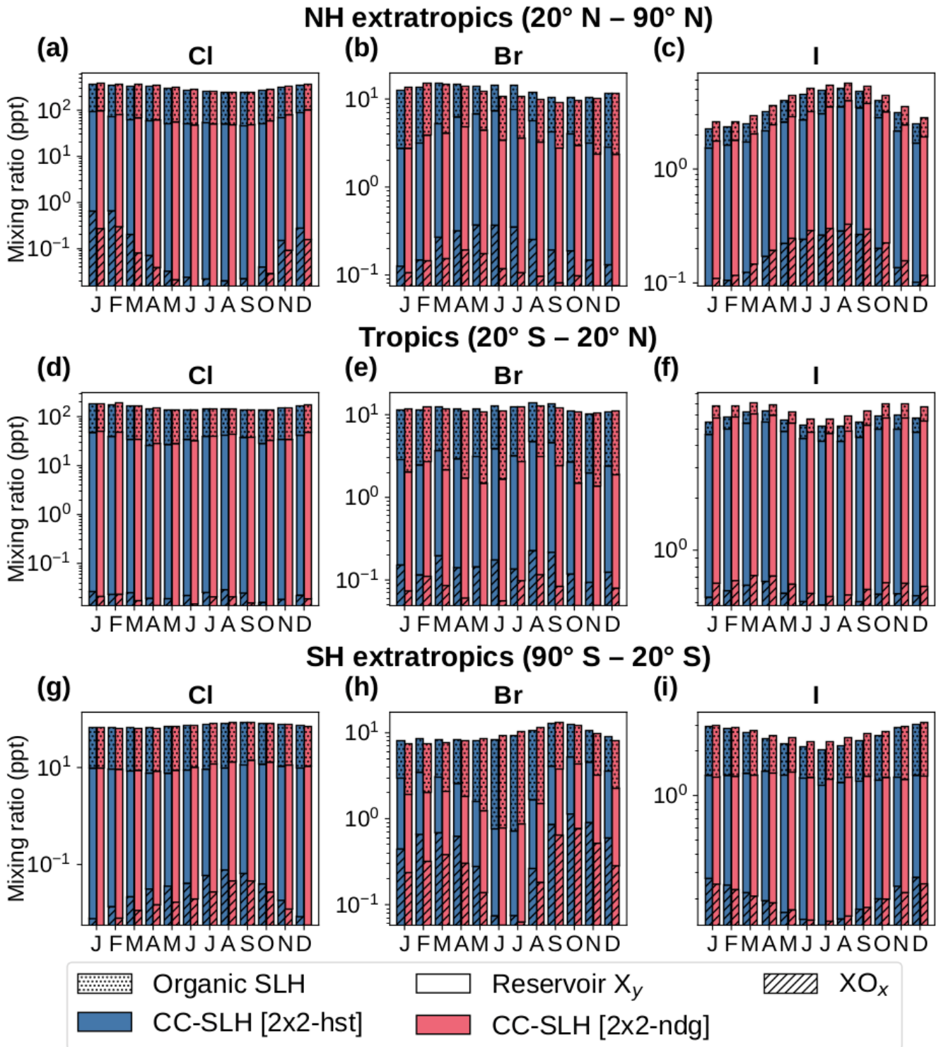
Figure 12: Seasonal distribution of total SLH abundance during present-day (2015–2020) for a-c) Northern Hemisphere (NH = 20° N–90° N) extratropics; d-f) Tropical (20° N–20° S) mean; and g-i) Southern Hemisphere (SH = 20° S–90° S) extratropics. Each coloured stacked bar distinguishes the contribution from organic VSL x (stippled bars), reactive ( XO_x , striped bars) and reservoir (empty unhatched bars) halogens (i.e., the sum of reactive XO_x plus reservoir species representing total inorganic halogens, X_y ) for the nudged CC-SLH [2×2-ndg] and free-running CC-SLH [2×2-hst] experiments.
