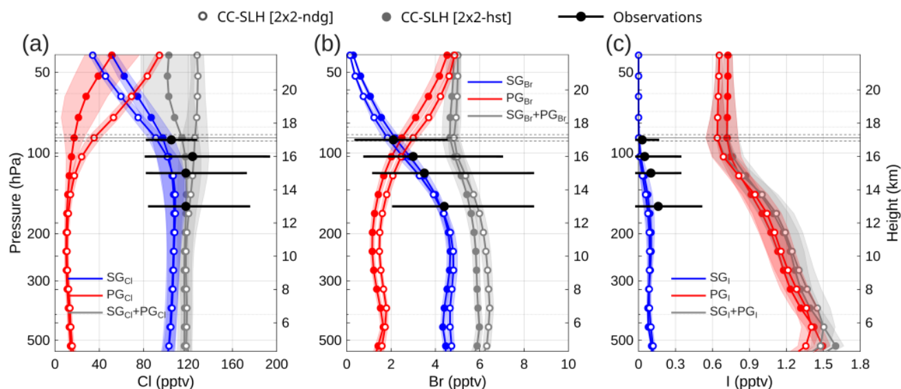
Figure 4: Tropical mean vertical profile of organic SLH source gases (SG x ) and product gases (PG x ) during present-day (2015–2020) for a) chlorine, b) bromine and c) iodine. The SGs profiles (blue lines) correspond to the nudged CC-SLH [2×2-ndg] (empty symbols) and the free-running CC-SLH [2×2-hst] (filled symbols) experiments, while PGs profiles (red lines) are obtained as the difference with respect to the corresponding CC-NOH sensitivity (see text for details). The total additional halogen abundance due to SLH (SG x + PG x ) is shown in grey. The tropical (20° N–20° S) mean and spread (i.e., ± the interannual standard deviation for the 2015–2020 period) are shown with solid lines and coloured shading, respectively. Average and range of observed VSL mixing ratios in the tropical tropopause layer compiled in Table 1-5 of WMO (2022) are shown in black symbols and solid-thick horizontal lines at 13, 15, 16 and 17 km, respectively. The solid and dashed horizontal lines indicate the tropical mean tropopause height ± standard deviation.
