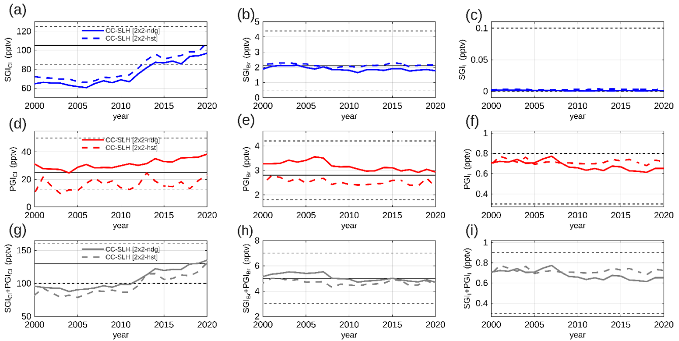
Figure 5: Temporal evolution of tropical ( 20^{\circ}\text{ N}–20^{\circ}\text{ S} ) source gas injection ( \text{SGI}_X , top-row), product gas injection ( \text{PGI}_X , middle-row) and total SLH injection ( \text{SGI}_X + \text{PGI}_X , bottom-row) to the stratosphere from 2000 to 2020 for the nudged CC-SLH [2x2-ndg] (solid lines) and free-running CC-SLH [2x2-hst] (dashed lines) experiments. Individual results for (a, d, g) chlorine, (b, e, h) bromine and (c, f, i) iodine are respectively shown on the left, middle and right columns, respectively. The reported best estimate and range of SGI and PGI for each individual family compiled in Table 1-6 of WMO (2022) are respectively represented by horizontal solid and dashed lines on each panel. Intermediate species \text{COCl}_2 , \text{CHCl}_2\text{O}_2 and \text{COFCl} (see Fig. S3) are assumed to contribute to \text{PGI}_{\text{Cl}} .
