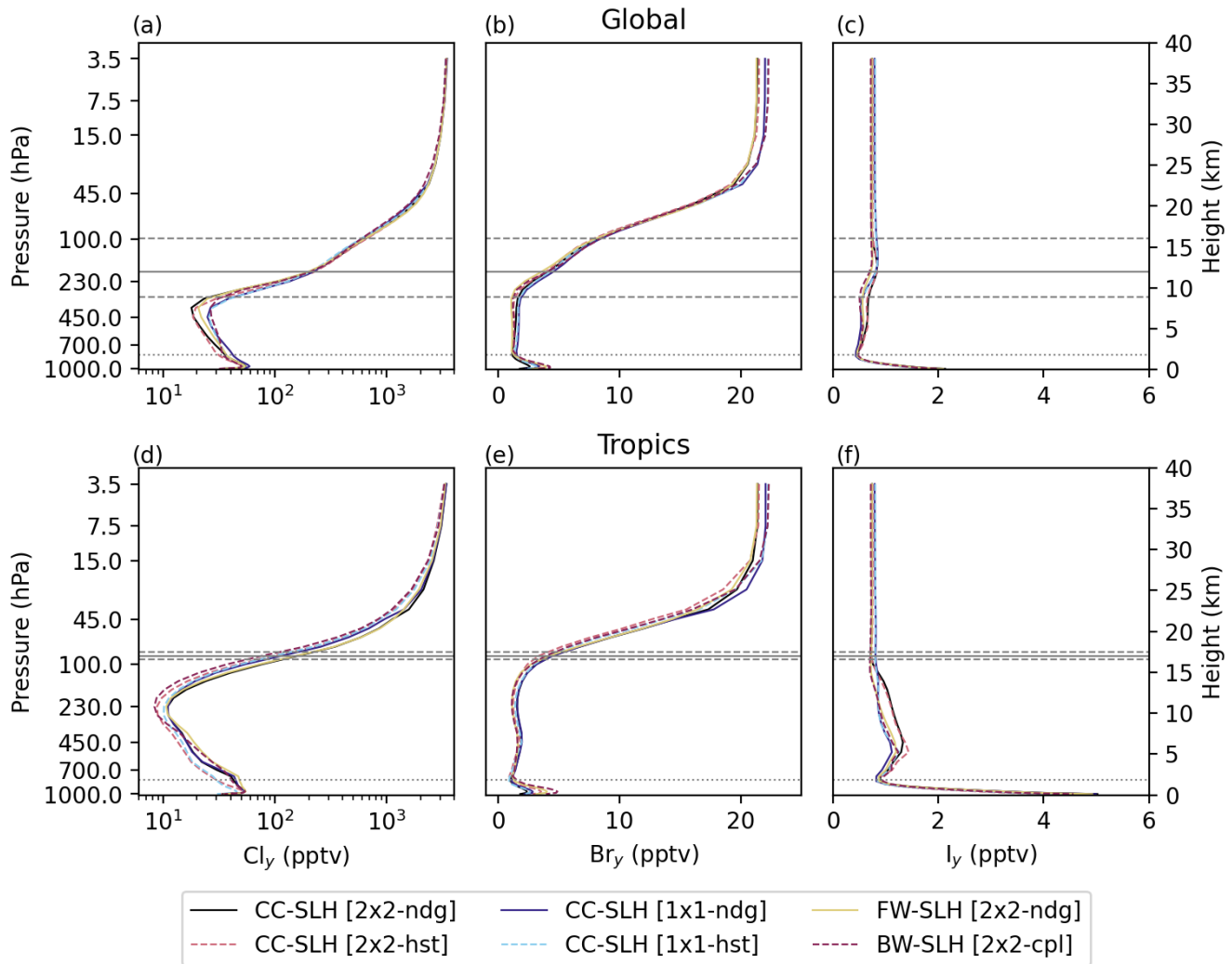
Figure 19: Comparison of global ( 90^\circ N - 90^\circ S ; top-row) and tropical ( 20^\circ N - 20^\circ S ; bottom-row) mean vertical profiles of total inorganic halogen abundance ( X_y ) between the 6 different CESM2-SLH experiments. Left, middle and right columns show results for (a, d) chlorine, (b, e) bromine and (c, f) iodine. The horizontal solid and dashed lines show the global or tropical mean tropopause height \pm standard deviation, while the horizontal dotted line corresponds to P = 850 hPa.
