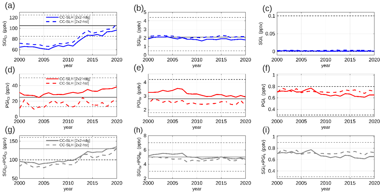
Figure 5: Temporal evolution of tropical (20°N – 20°S) source gas injection (SGI x , top-row), product gas injection (PGI x , middle-row) and total SLH injection (SGI x + PGI x , bottom-row) to the stratosphere from 2000 to 2020 for the nudged CC-SLH [2×2-ndg] (solid lines) and free-running CC-SLH [2×2-hst] (dashed lines) experiments. Individual results for (a, d, g) chlorine, (b, e, h) bromine and (c, f, i) iodine are respectively shown on the left, middle and right columns, respectively. The reported best estimate and range of SGI and PGI for each individual family compiled in Table 1-6 of WMO (2022) are respectively represented by horizontal solid and dashed lines on each panel. Intermediate species COCl 2 , CHCl 2 O 2 and COFCl (see Fig. S3) are assumed to contribute to PGI Cl .
