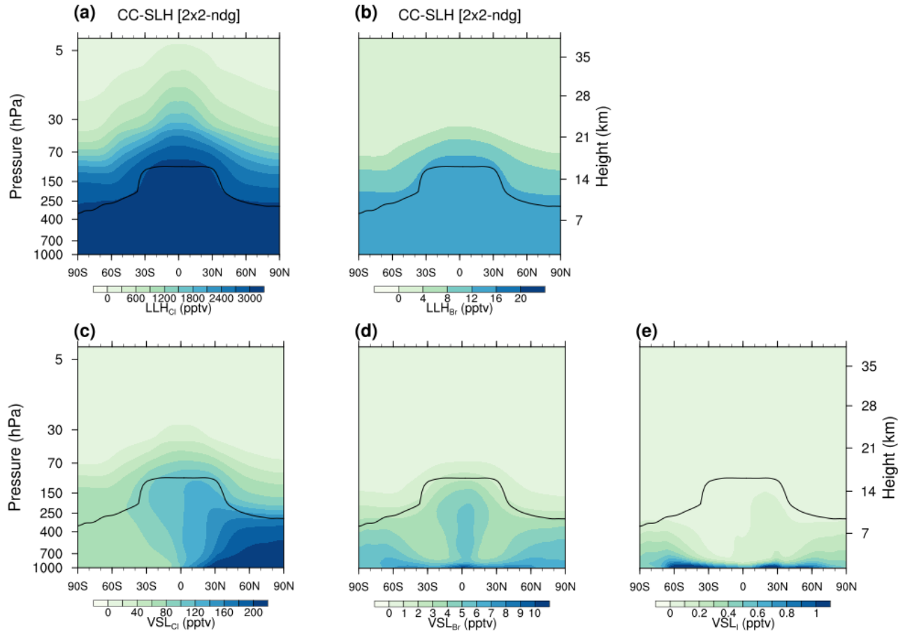
Figure 7: Zonal average distribution of the organic halogen fraction during present-day (2015–2020) for the nudged CC-SLH [2x2-ndg] experiments. Top row shows the long-lived (LL) distribution for a) chlorine (LLCl) and b) bromine (LLBr). Note that CEM2-SLH does not include long-lived iodine species. Bottom row shows the very short-lived (VSL) distribution for c) chlorine (VSLCl), d) bromine (VSLBr) and e) iodine (VSLI). The black solid line shows the mean model tropopause.
