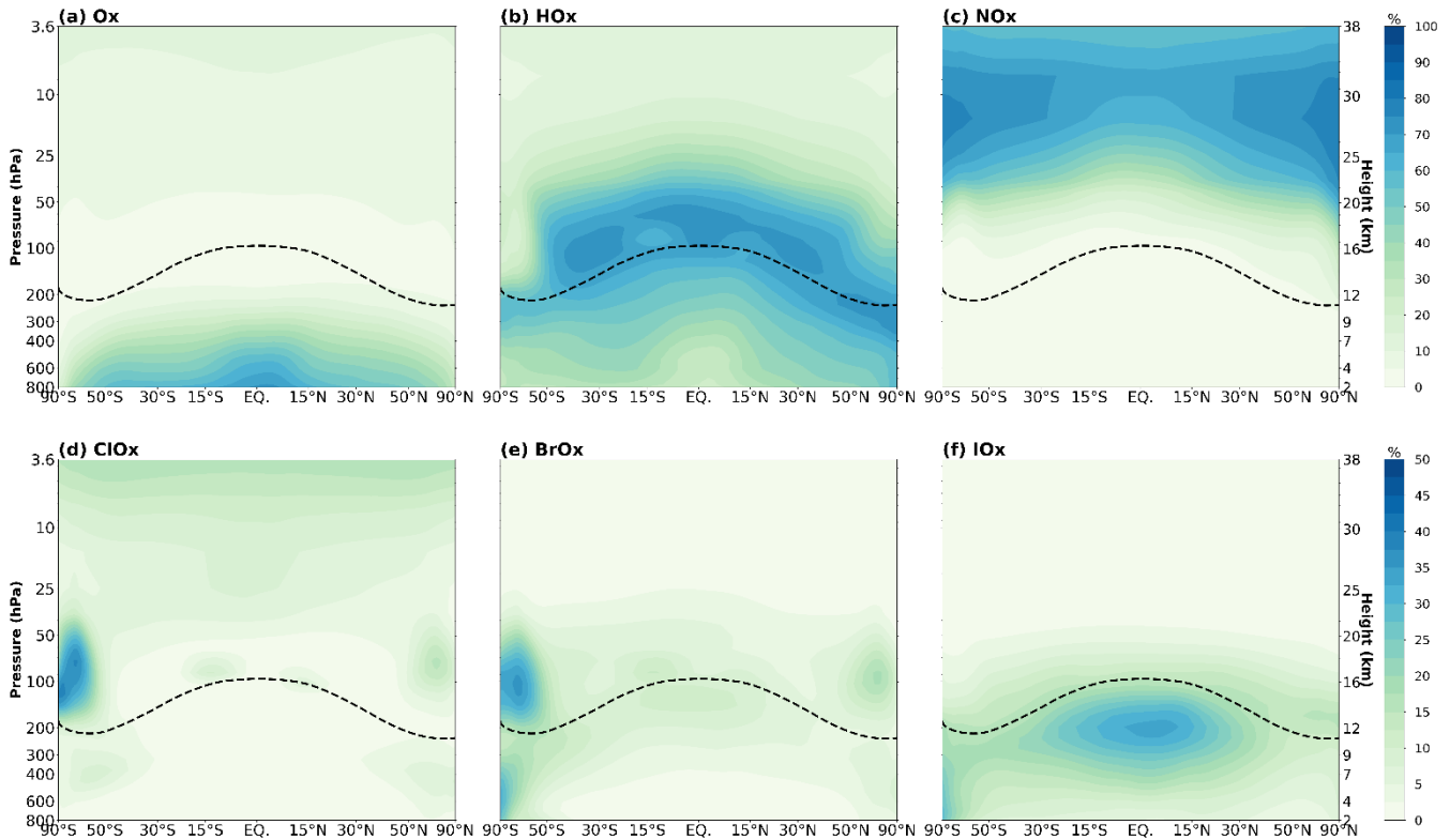
Figure 16: Zonal average distribution of Odd-oxygen loss rates ( OddOx Loss ) for different ozone depleting families during present-day (2015–2020). Each panel presents the percentage contribution of each OddOx Loss family to the total ozone loss for the CC-SLH [2×2-ndg] experiment . The top-row show results for the main OddOx Loss channels when SLH are not considered: a) O x , b) HO x and c) NO x loss cycles, while the bottom-row shows the percentage contribution from the individual halogen-driven OddOx Loss cycles: d) ClO x , e) BrO x and f) IO x . The black-dashed line indicates the model mean tropopause.
