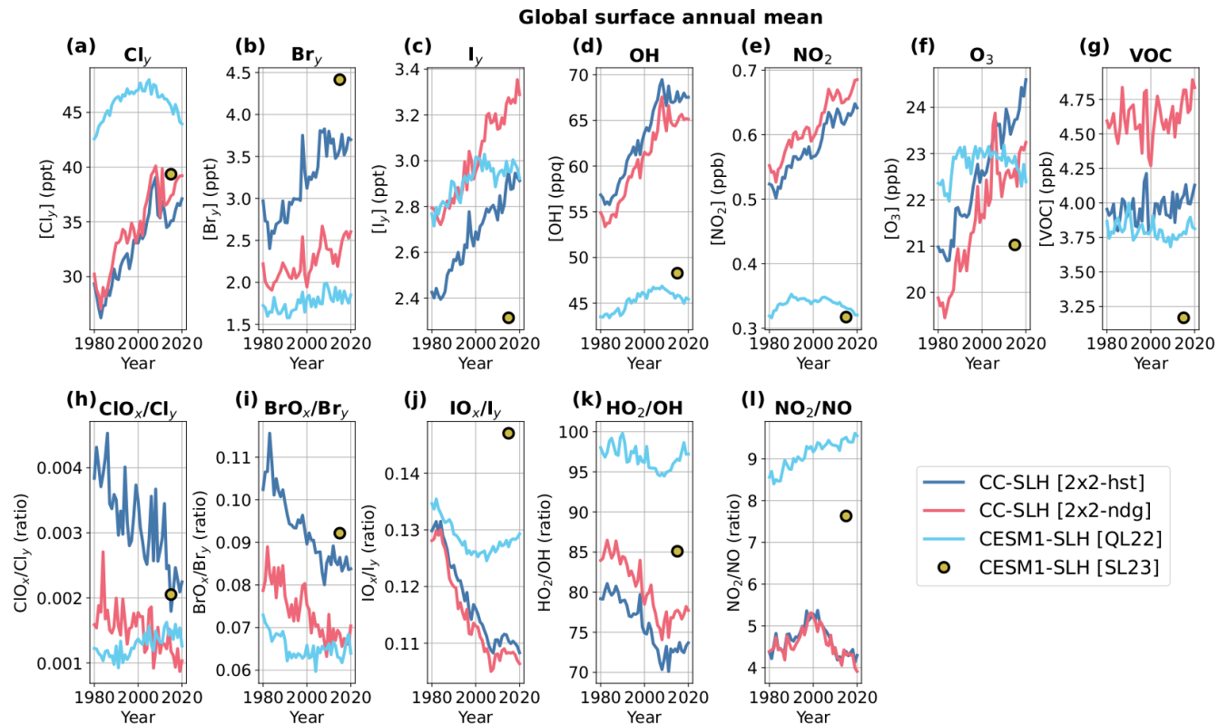
Figure 2: Historical evolution of global annual mean surface abundance and partitioning of main atmospheric components during 1980–2020. Top-row shows the total inorganic halogen surface abundance for a) Cl_y , b) Br_y and c) I_y , as well as the surface mixing ratio for d) OH , e) NO_2 , f) O_3 , and g) VOC (calculated as the sum of species: ISOP, MTERP, CH_3OH , C_2H_5OH , CH_2O , CH_3CHO , CH_3COOH , CH_3COCH_3 , HCOOH , C_2H_2 , C_2H_4 , C_2H_6 , C_3H_8 , C_3H_6 , BIGALK, BIGENE, MEK, TOLUENE, BENZENE, XYLENES). Bottom row shows the reactive ( XO_x ) to reservoir ( X_y ) surface ratio (i.e., XO_x/X_y ) for h) chlorine, i) bromine and j) iodine, as well as the k) HO_2/OH and l) NO_2/NO mean ratio at the model surface. Results for the nudged CC-SLH [2×2-ndg] (pink) and free-running CC-SLH [2×2-hst] (blue) experiments obtained with the CESM2-SLH release are compared with those obtained in previous CESM1 studies (see Section 3.3).
