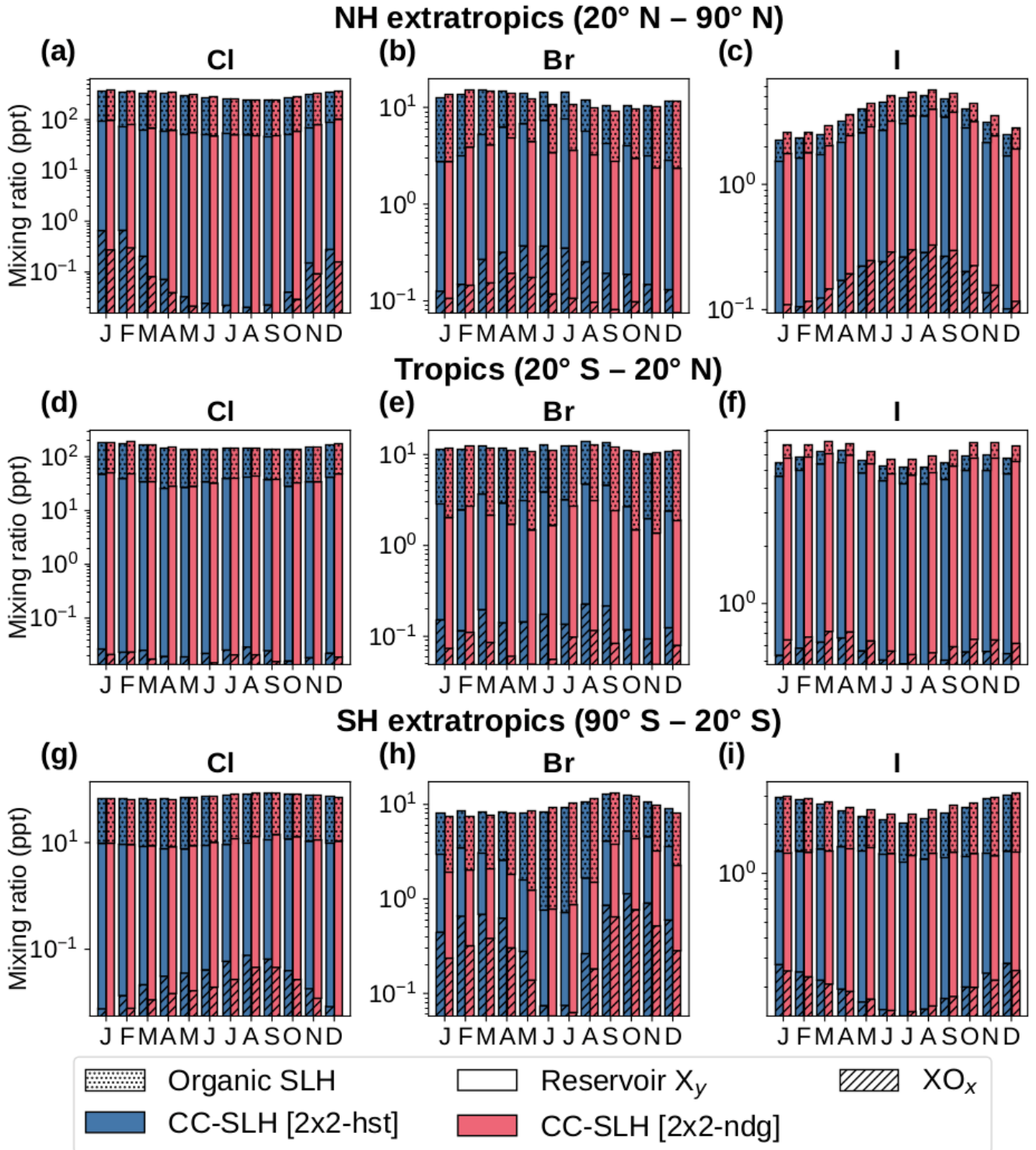
Figure 12: Seasonal distribution of total SLH abundance during present-day (2015-2020) for a-c) Northern Hemisphere (NH = 20° N – 90° N) extratropics ; d-f) Tropical (20°N – 20°S) mean ; and g-i) Southern Hemisphere (SH = 20° S – 90° S) extratropics . Each coloured stacked bar distinguishes the contribution from organic VSL x (stippled bars), reactive (XO x , striped bars) and reservoir (empty unhatched bars) halogens (i.e., the sum of reactive XO x plus reservoir species representing total inorganic halogens, X y ) for the nudged CC-SLH [2×2-ndg] and free-running CC-SLH [2×2-hst] experiments.
