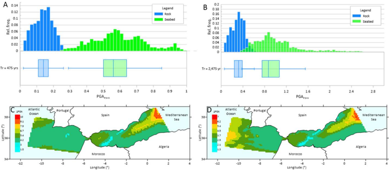
590 Figure 10. Distributions and relative-change maps of PSHA (in terms of PGA) at the seabed. (A–B) Histograms (in relative frequency) and box–whisker plots of estimated PGA values for return periods of 475 years (A) and 2475 years (B), comparing
