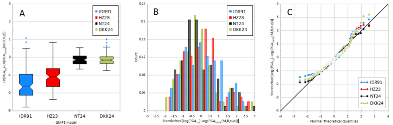
300 Figure 6. Diagnosis of the residuals in logarithms of PGA. A) Box-Whisker plot of residuals for each GMPE model used in this study. B) Stacked histogram in relative frequencies for the residuals in logarithms of PGA. C) Q-Q plot of the standardised residuals in logarithms of PGA.
