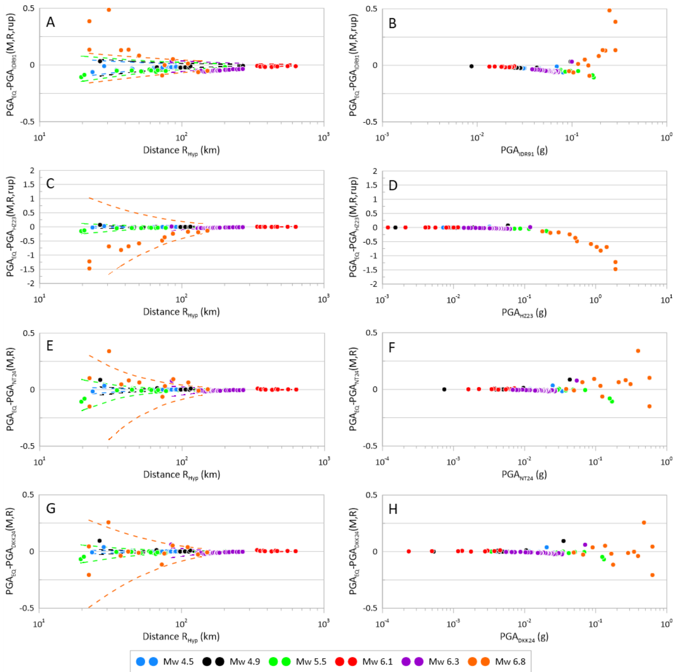
Figure 5. Residual plots of the goodness of fit for the predicted values by the selected GMPEs: IDR91 (A and B), HZ23 (C and D), NT24 (E and F), and DKK24 (G and H), against the registered data in the earthquakes used for diagnosis.
