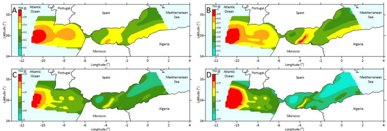
Figure 8. Probabilistic seismic hazard maps for the mean horizontal PGA (g) at APEs of (A) 1/100, (B) 1/475, (C) 1/2475, and (D) 1/5000. All values are estimated under soft soil conditions with V_{s30} = 200 m/s.
