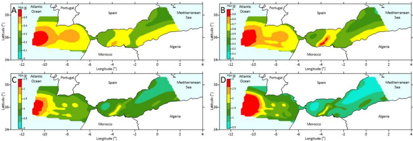
515 Figure 8. Probabilistic seismic hazard maps for the mean horizontal PGA (g) at APEs of (A) 1/100, (B) 1/475, (C) 1/2475, and (D) 1/5000. All values are estimated under soft soil conditions with V_{s30} = 200 m/s.
