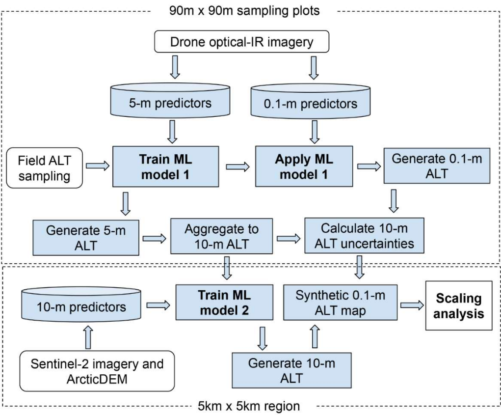
230 Figure 3: An overall flowchart of the machine learning (ML) based active layer thickness (ALT) mapping and analysis.
