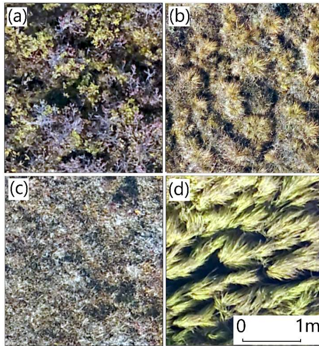
Figure 2: The study region contains characteristic tundra vegetation types, including dwarf shrubs (a), tussock-forming sedges (b), moss-lichen mats (c), and riparian grasses along watercourses (d). The images (0.7cm resolution) were acquired from a drone-based RGB camera.
