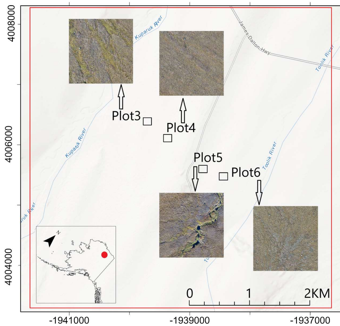
160 Figure 1: The study region encompasses an Arctic tundra area ( 68.6167^{\circ} , -149.3167^{\circ} ; red dot in the inset) in the northern foothills of the Brooks Range, Alaska. The region consists of four intensively sampled plots (Plot 3, Plot 4, Plot 5, and Plot 6; 90 m x 90 m each) with their corresponding true-color RGB (red-green-blue) drone images displayed alongside for visual inspection only, and surrounded by a larger 5km by 5km study region (red rectangle) used for analyzing ALT scaling effects. The map was plotted using Canada Albers Equal Area Conic projection.
