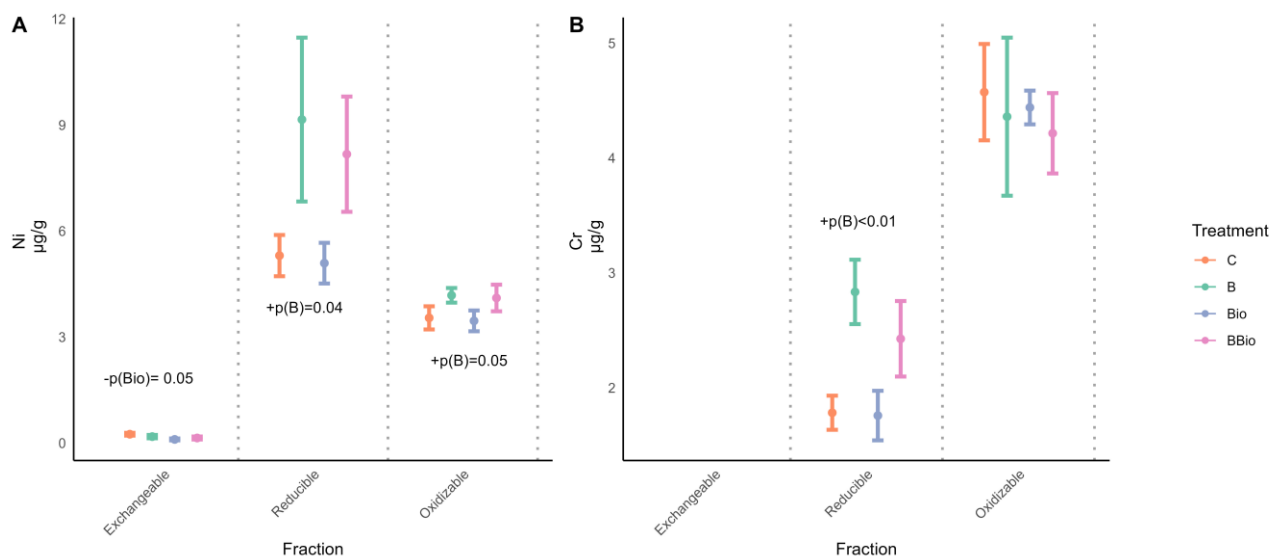
275 Figure 4: Ni and Cr in the 4 different considered soil fractions. These soil elements were extracted after initial soil sampling in clover plots. P(B) and p(Bio) are p values for basalt and biochar, respectively. Carbonate-Ni, carbonate-Cr and exchangeable Cr were below detection limits and are not shown in this plot. Significant positive and negative effects are indicated with a + and – respectively. A vertical dotted line is plotted in between different soil fractions.
