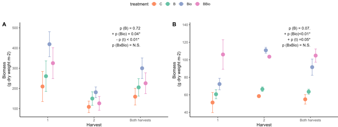
Figure 6: Aboveground dry biomass in function of time after amendment for (A) clover and (B) mustard plots. “N.S.” = Not significant, this is indicated when the interaction effect was tested for but was not statistically significant. p(B), p(Bio), p(t) and p(BxBio) represent p values of basalt, biochar, time and basalt x biochar effects. Dots and error bars represent mean biomass +/- the standard error of the mean. Significant positive and negative effects are indicated with a + and – respectively.
