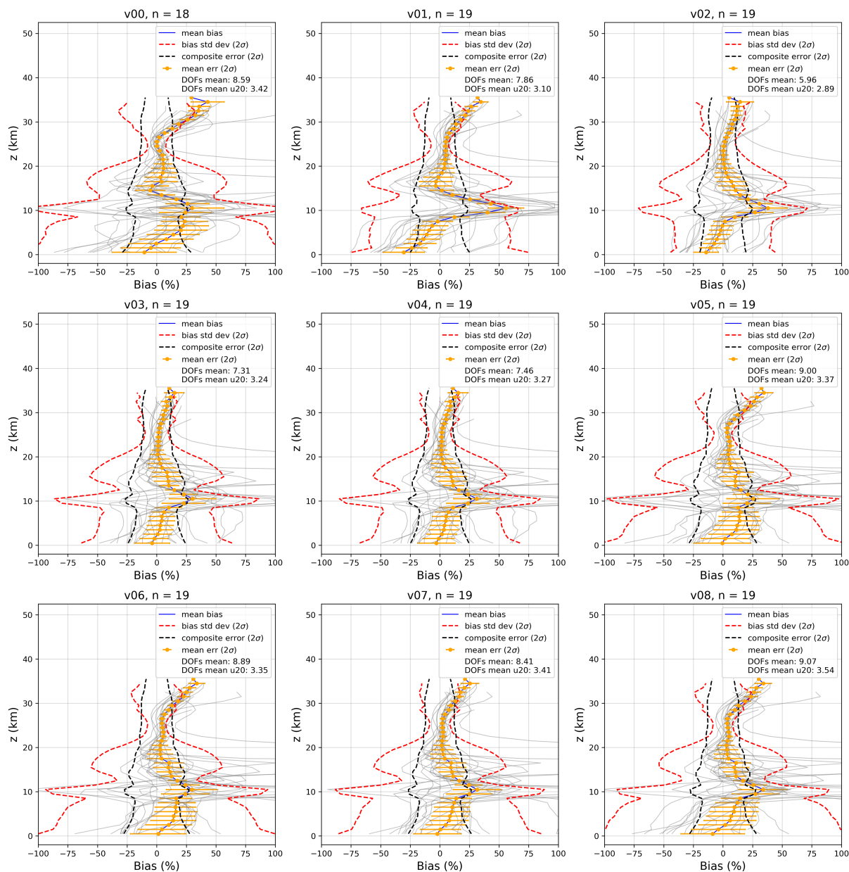
Figure 2. Validation of the 9 versions of the CDF method in the tuning phase, performed in 2008 within the latitudinal band 5^{\circ} - 55^{\circ} N. The blue line represents the average percentage bias between the fused profiles and the smoothed ozonesondes with the AK of the fused profile. The red dashed line indicates the standard deviation of the mean bias ( 2\sigma ), the black dashed line represents the combined error ( 2\sigma ), while the orange bars show the standard error of the mean. The background gray profiles represent the n averaged profiles. In the legend, and DOFs mean u20 represents the average number of degrees of freedom below 20 km.
