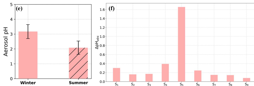
816 Figure 6: Mean fine aerosol pH in winter and in summer at (a) IOA (c) THI, (e) FKL and the respective sensitivity 817 results for winter conducted for each site (Tables S5 - S7). \Delta pH_{abs} = |pH_{winter} - pH_{winter(summerX)}| , where summerX is the 818 mean summer temperature (first simulation, S 1 ), relative humidity (S 2 ), TNO 3 (S 3 ), TNH 3 (S 4 ), SO 4 2- (S 5 ), Na + (S 6 ), K + 819 (S 7 ), Ca 2+ (S 8 ) and OA concentration (S 9 ) in IOA (b), THI (d) and FKL (f).
