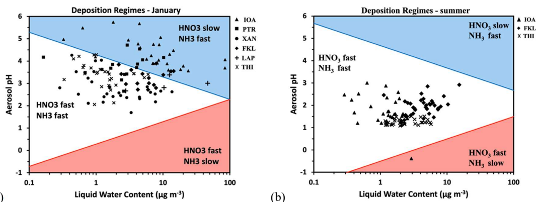
(a) (b) Figure 10: Domains of reactive nitrogen deposition for the studied period (a) in winter (January) and (b) in summer (July and August). The average temperature used here is the mean measured one at all sites, for each season. Daily averaged values in each season for aerosol pH and liquid water content were used. The red line shows the characteristic aerosol pH, as a function of liquid water content, below which \text{NH}_3 deposition is slow and the blue line the characteristic aerosol pH, as a function of liquid water content, above which \text{HNO}_3 deposition is slow.
