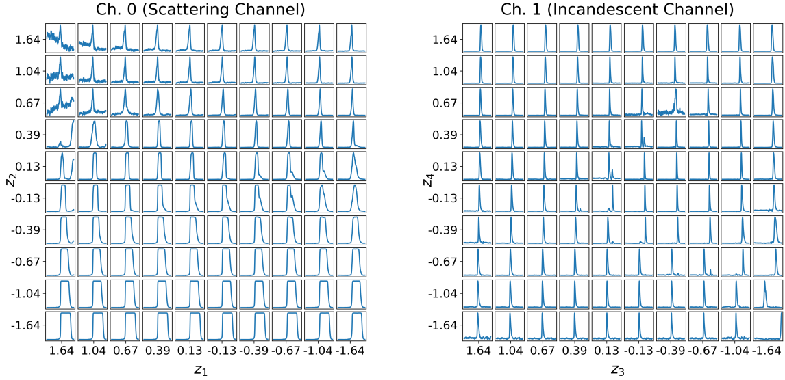
Figure 6. Latent Manifolds for the L-II Signals. By sampling along the deciles of a gaussian distributions for the 2 latent variables from each channel, we visualize characteristic L-II signals using the trained decoder. These learned latent manifolds provide an overview of the modes of variability described by the latent representations of the two channels. Left: Latent Manifold for Channel 0, showing the variability represented by z_1 (x-axis) and z_2 (y-axis). Right: Latent Manifold for Channel 1, showing the variability represented by z_3 (x-axis) and z_4 (y-axis).
