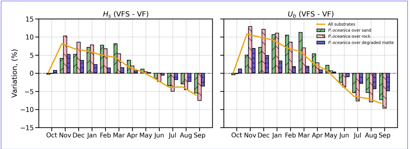
Figure 10. Timeseries of mean monthly H_s and U_b percentage difference between VFS and VF simulations across substrate types ( (H_{VFS} - H_{VF})/H_{VF} \times 100 ). Bars indicate the average differences over vegetated points for each substrate, while the solid orange line represents the weighted average across all vegetated areas in the domain.
