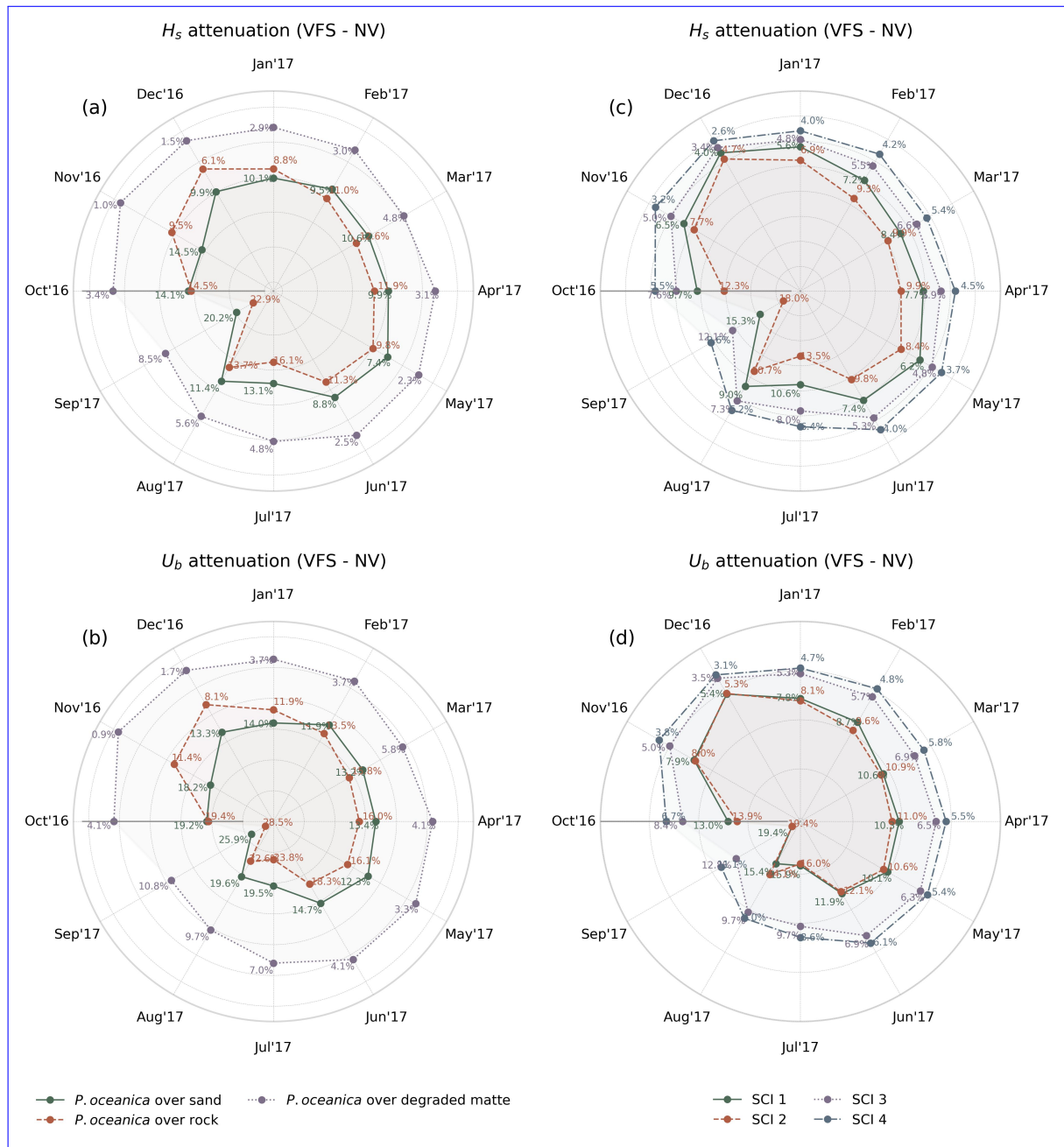
Figure 9. Mean monthly H_s and U_b percentage reduction (VFS experiment) for P. oceanica over different substrates (a,b), and four SCIs (c,d), averaged across vegetated points in the mask.
