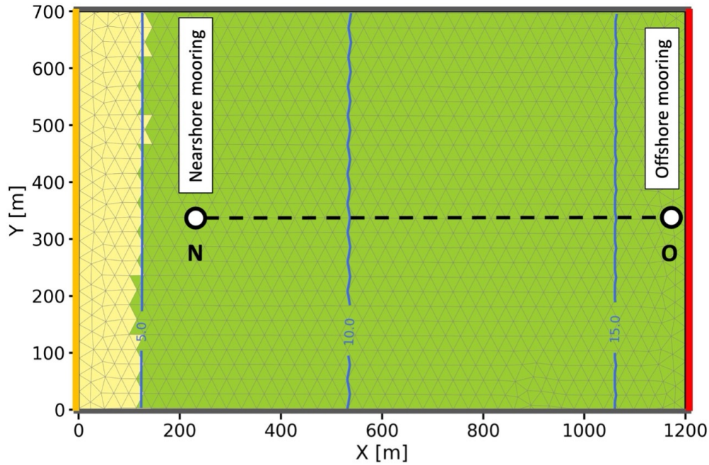
Figure 1. A Cala Millor case study domain and bathymetry customized from Infantes et al. (2012), with location of mooring data. O denotes offshore moorings, while N denotes nearshore moorings. Green mesh elements indicate elements with vegetation, while yellow elements do not include vegetation at the bottom. The dashed line represents the transect N-O analyzed later.
