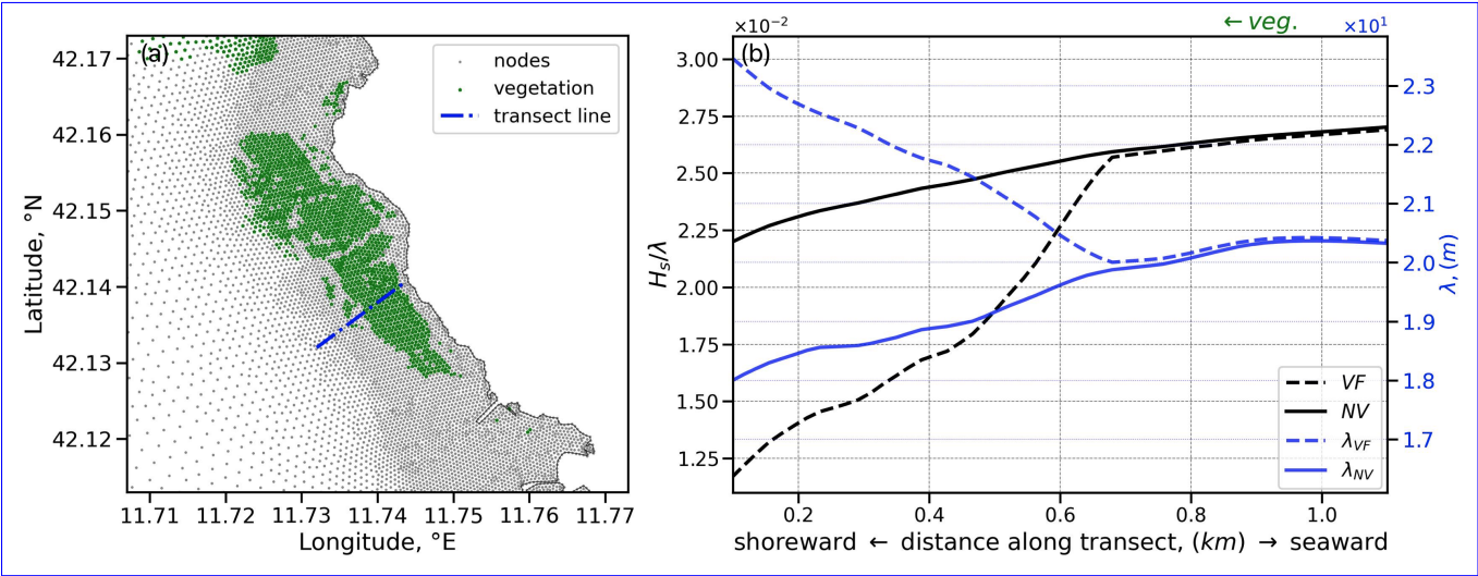
Figure B1. The impact of vegetation on wave characteristics. (a) Transect line at SCI 2 site, near P05 sampling station; (b) Wave steepness and mean wavelength profiles (annual means) along the transect line, where the shore end is the origin of the x-axis.
