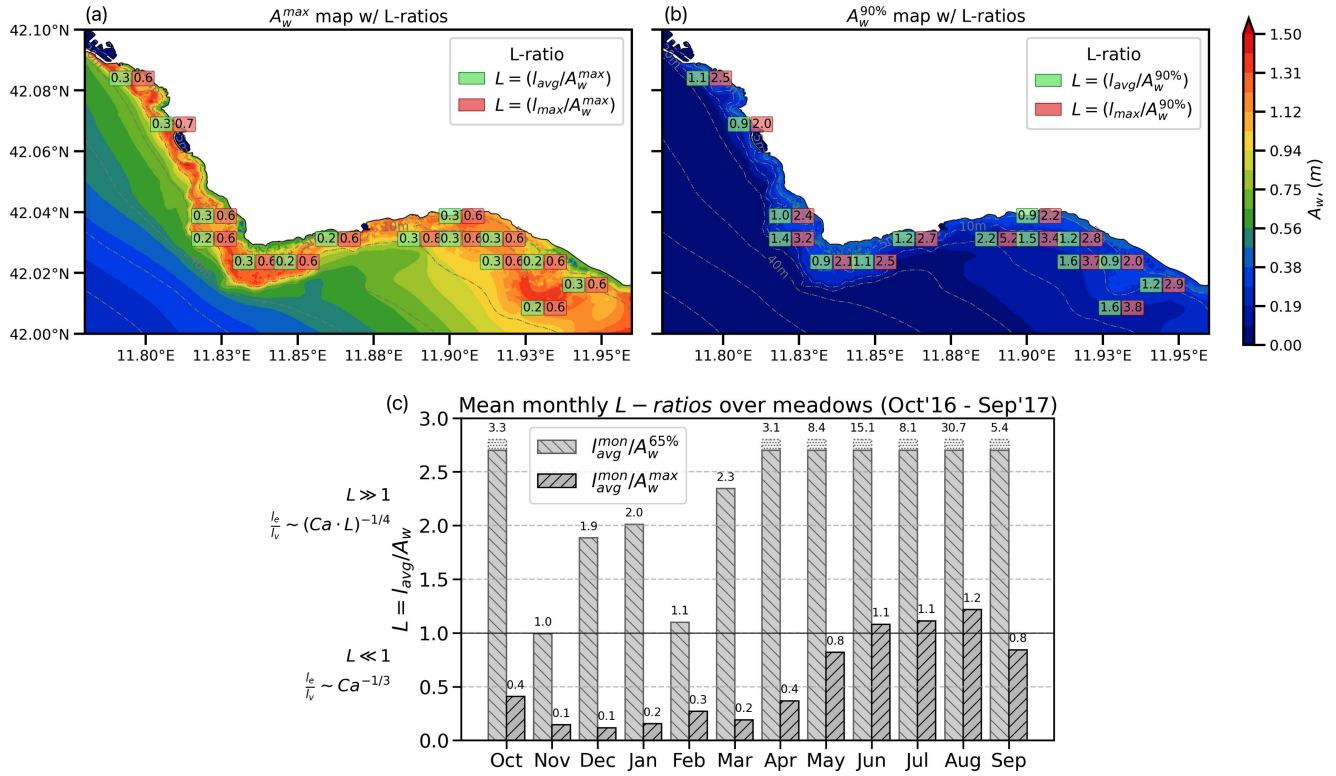
Figure C1. Maps (a, b) of wave orbital excursion ( A_w ) with the L -ratios over the vegetated areas; (c) the domain-averaged (over vegetation only) monthly mean L -ratios.
