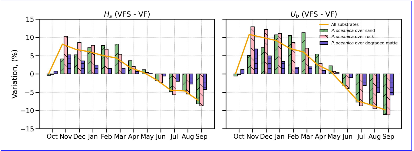
Figure 10. Timeseries of mean monthly SWH-H_s and UBR-U_b percentage difference between VFS and VF simulations across substrate types \bar{H}_{VFS} - \bar{H}_{VF} and \bar{U}_{BFS} - \bar{U}_{BF} averaged over ((H_{VFS} - H_{VF})/H_{VF} \times 100) . Bars indicate the vegetation-average differences over vegetated points per for each substrate in, while the mask (bars) and over all substrates (orange) solid orange line represents the weighted average across all vegetated areas in the domain.
