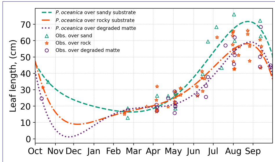
Figure 5. Timeseries of PO leaves height P. oceanica leaf length variation throughout the year, showing seasonal observations alongside fitted growth curves. The corresponding coefficients used for the fitted curves are provided in Appendix A2.
