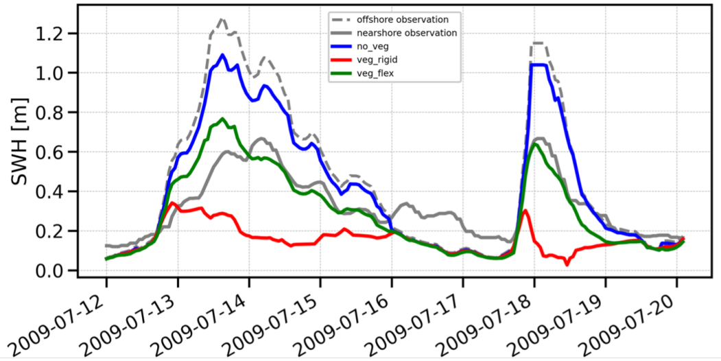
Figure 2. Significant wave height (SWH) timeseries comparison for no_veg , veg_rigid no_veg (no vegetation), veg_rigid (rigid vegetation) and veg_flex (flexible vegetation) experiments against nearshore and offshore moorings in the idealized geometry of Figure 1.
