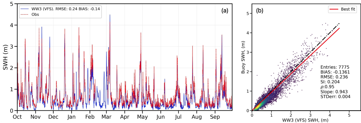
Figure 7. Comparison of the wave model results ( VFS ) with the buoy data (Figure 4a) in terms of timeseries (a) and a scatter plot (b). In plot (b), the dash-dot black line represents the perfect correlation for the reference, while the solid red line shows the model fitting. A statistical summary is also provided.
