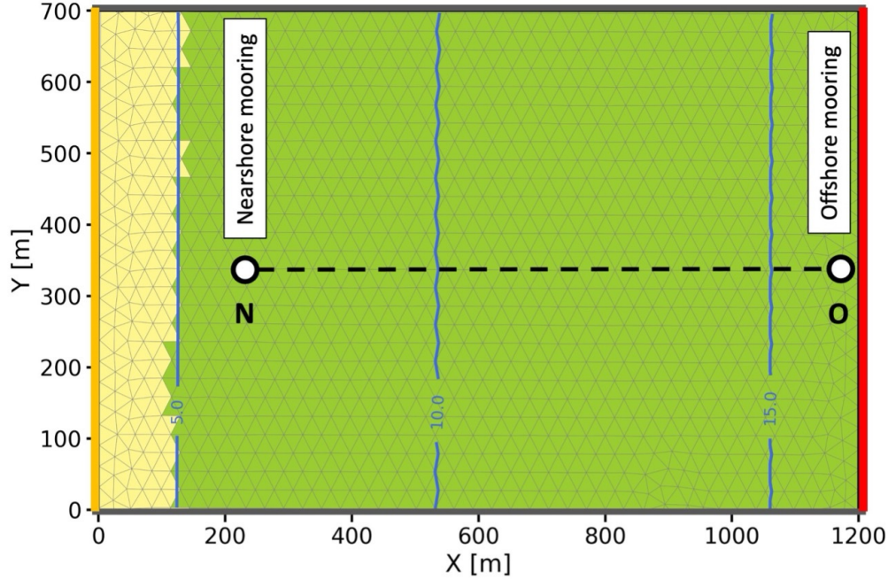
Figure 1. I dealized test-A Cala Millor case ( study domain and bathymetry) customized from Infantes et al. (2012), with location of mooring data. O denotes offshore moorings, while N denotes nearshore moorings. Green mesh elements indicate elements with vegetation, while yellow elements do not include vegetation at the bottom. The dashed line represents the transect N-O analyzed later.
