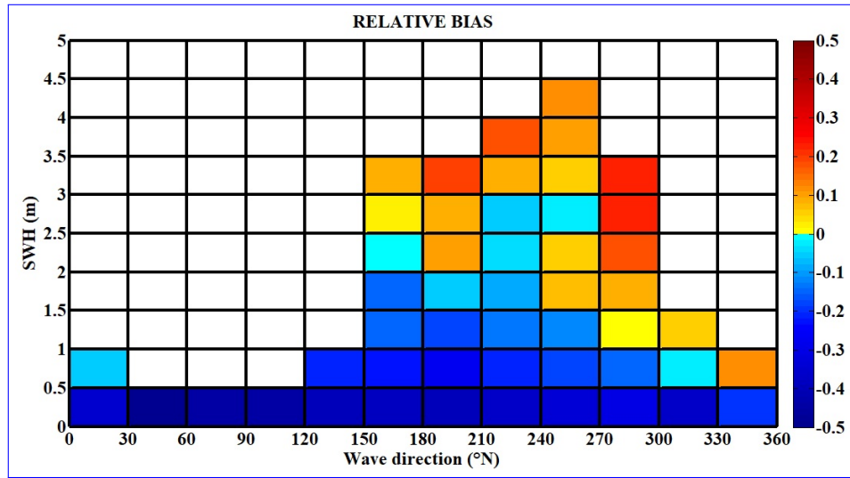
Figure 8. Heatmap of SWH and wave direction relative bias heatmap (mdimensionless), with the relative bias formulation described in Roelvink et al. (2009) .
