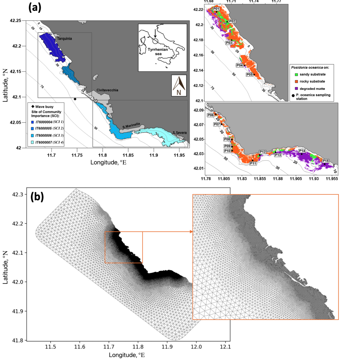
Figure 4. Map of the area of Civitavecchia with bathymetry, Sites of Community Importance (SCI), observations used in the study and distribution of the Posidonia oceanica ( P.O ) P. oceanica over the different substrate types ( P.O P. oceanica on rock, P.O P. oceanica on sand and matte, and degraded matte with P.O P. oceanica ). (b) Mesh of the computational domain with enlarged views in the vicinity of the Civitavecchia harbour.
