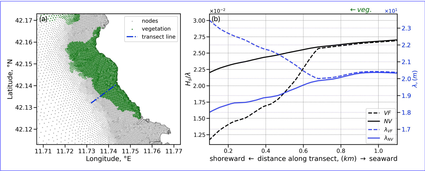
Figure B1. The impact of vegetation on wave characteristics. (a) Transect line at SCI 2 site, near P05 sampling station; (b) Wave steepness and mean wavelength profiles (annual means) along the transect line, where the shore end is the origin of the x-axis.
