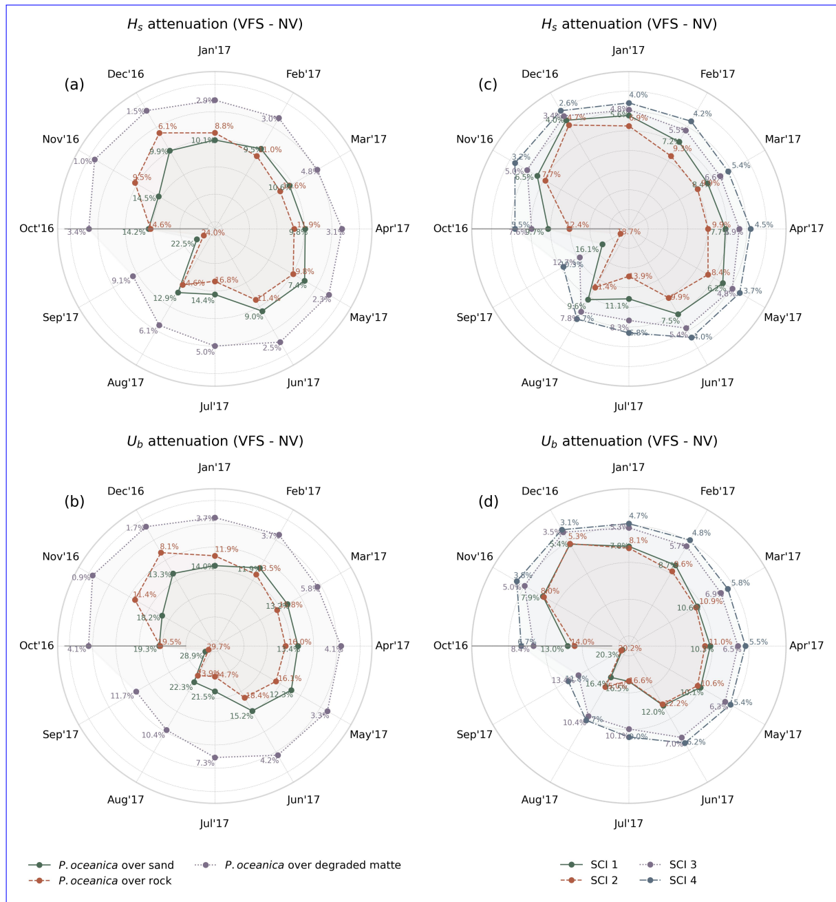
Figure 9. Mean monthly SWH- H_s and UBR- U_b percentage reduction for (VFS configuration experiment) for the three different phenotypic traits of P. oceanica (over rock different substrates (a, sand, degraded matte b), and four SCIs (c, d), averaged across vegetated points in the mask.
