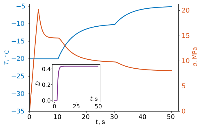
Figure 8. Deviatoric response of a triaxial compression under \sigma_3 = 10 MPa and a constant strain rate of \dot{\epsilon}_q = 1.5 \times 10^{-3} s^{-1} , while the temperature is increased gradually from T = -20^\circ\text{C} to -5^\circ\text{C} . The inset shows the associated change in the damage parameter.
