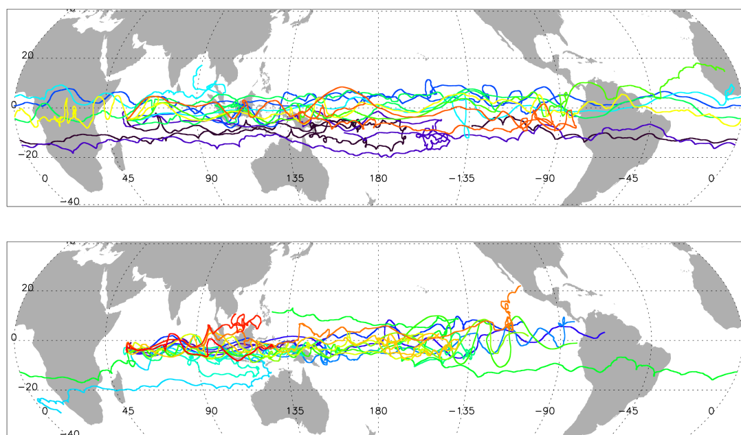
Figure 1. Trajectories of Strateole-2 balloon flights during (top) the 2019 and (bottom) the 2021 campaigns.
