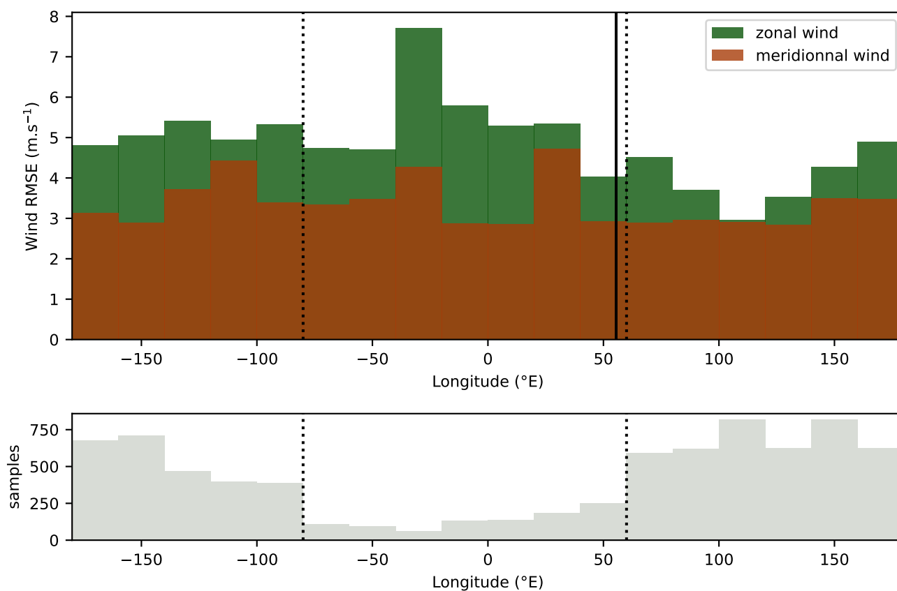
Figure 4. The figure at the top shows the distribution of root mean square error (RMSE) of zonal (green) and meridional wind from ERA-5 as a function of longitude. Only data between 8°S and 8°N are shown. The figure at the bottom gives for each longitude the number of samples available. The solid black line indicates Mahé's longitude. The dashed line highlights the longitudes between which there is a lack of observations.
