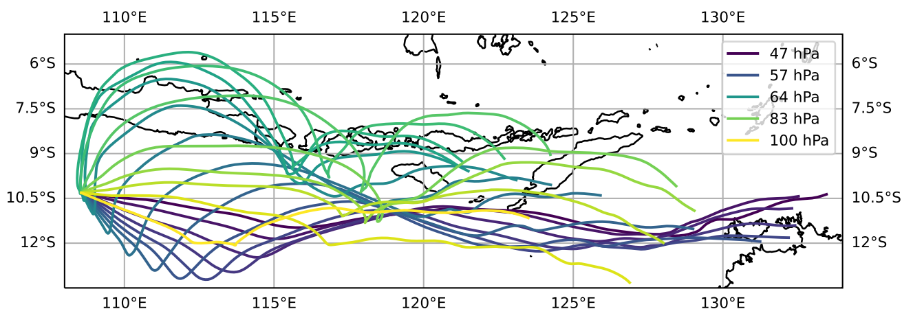
Figure 10. Three-day long isentropic back trajectories starting the 26 th of January from the position of balloon 1 at several pressure level.
