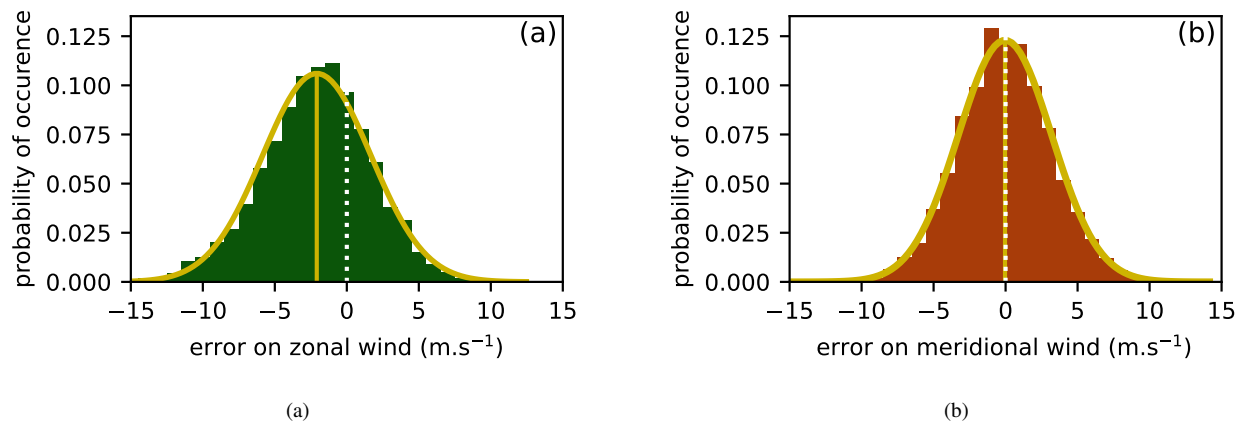
Figure 3. Histograms of ERA-5 wind error from three-hourly data of every balloon from both 2019 and 2021 Strateole campaign. Solid orange line is the Gaussian curve with the same mean and standard deviation as the histogram. Dashed yellow line is the mean. Dotted white line indicates the 0 of the horizontal axis. Bin size for both panels is 1 \text{ ms}^{-1}
