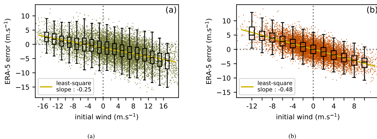
Figure 5. Scatter plot of the ERA-5 wind error as a function of the wind, in the zonal direction (panel (a)) and in the meridional direction (panel (b)). The black boxplot purpose is to visualize the scatter plot distribution. The grey dotted line show the null wind and null error axis.
