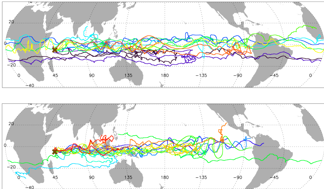
Figure 1. Trajectories of Stratéole 2 balloon flights during (top) the 2019 and (bottom) the 2021 campaigns. Eight balloons flew in 2019 with an average flight duration of 84 days. In 2021, 17 balloons were launched but the average flight duration was only 40 days because of issues with the balloon envelopes encountered in 2021. The balloons are launched from Seychelles Islands (55.5-4.7°E, -4.7°S) which is indicated by a cross.
