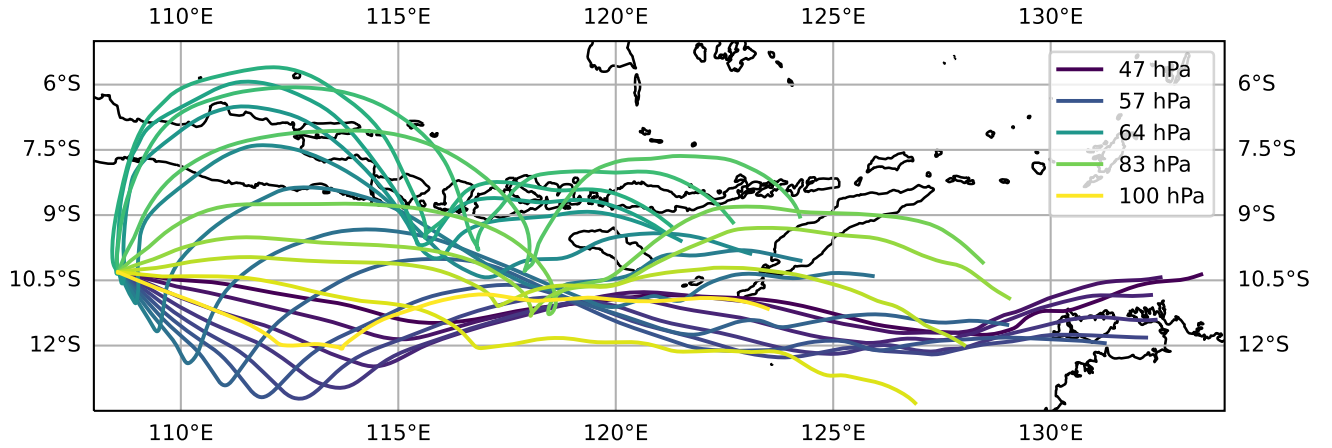
Figure 10. Three-day long isentropic back trajectories starting the 26 th of January from the position of balloon 1 at several pressure level.
