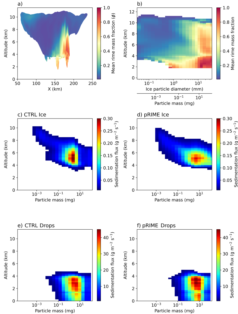
Figure 7. Vertical cross section ( y-direction averaged ) of the mean rime mass fraction \phi ( y-direction-averaged ) a), mean rime mass fraction as function of the particle size and altitude b). Sedimentation flux of ice particle as function of ice particle size or mass and altitude for the CTRL c) and pRIME simulation d). Sedimentation flux of drops as function of their size and altitude for the pRIME c) and CTRL simulation d). All panels are averaged for TWC > 0.01 g m -3 at 2:30h.
