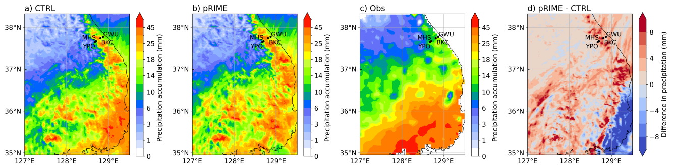
Figure 15. Precipitation accumulation (ice + rain) within the innermost domain from 07 March 00:00 to 09-08 09-08 March 0015:00 0015:00 UTC: a) DESCAM-CTRL , b) DESCAM-pRIME , c) Rain accumulation product from Automatic Weather Stations (AWS) operated by the Korea Meteorological Administration (KMA) interpolated using the method of Cressman (1959) and d) difference between DESCAM pRIME in b) and DESCAM-CTRL in a).
