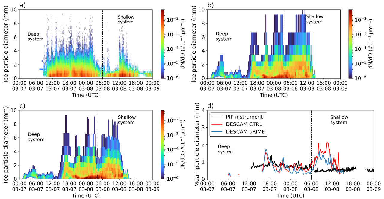
Figure 16. Temporal evolution of ground based observations of ice particle size distribution for a) the PIP instrument at MHS, b) DESCAM -CTRL simulation and c) DESCAM -pRIME simulation. Panel d) presents the number-weighted mean particle diameter (considering particles larger than 100 \mu\text{m} ) for both simulations and the PIP observations.
