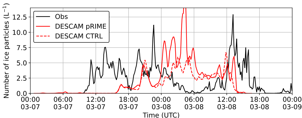
Figure 17. Temporal evolution of the number of ice particle (10-minute averaged) larger than 100 \mu\text{m} at MHS station, observed by the PIP instrument (black line) and simulated by DESCAM, with the CTRL and pRIME simulations shown in dashed and solid red lines, respectively.
