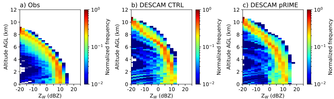
Figure 10. Frequency of W-band radar reflectivity as function of the altitude above ground level for the deep cloud system ( i.e. before 6:00 UTC on March 8 ) presented in Fig. 9 with: a) observations, b) DESCAM -CTRL simulation and c) DESCAM pRIME simulation.
