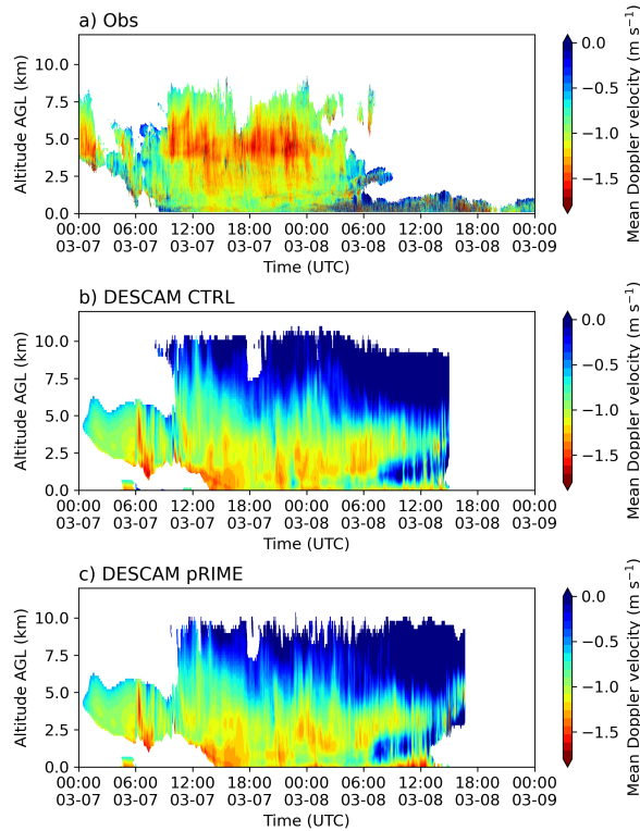
Figure 12. Mean Doppler velocity (defined positive upwards) at the MHS station for a) W-band radar observations in and b) DESCAM CTRL simulation and c) DESCAM -p PRIME simulation. Data are presented for reflectivity values exceeding -20 dBZ (see Fig. 9).
