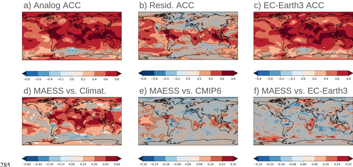
Figure 6: The same as Figure 1, but for annual TAS predictions (January - December). The evaluation period is 1962-2018. The predictions are initialized each November in both analog-based predictions and EC-Earth3. The dynamic forecasts system evaluated in c,f is EC-Earth3.
