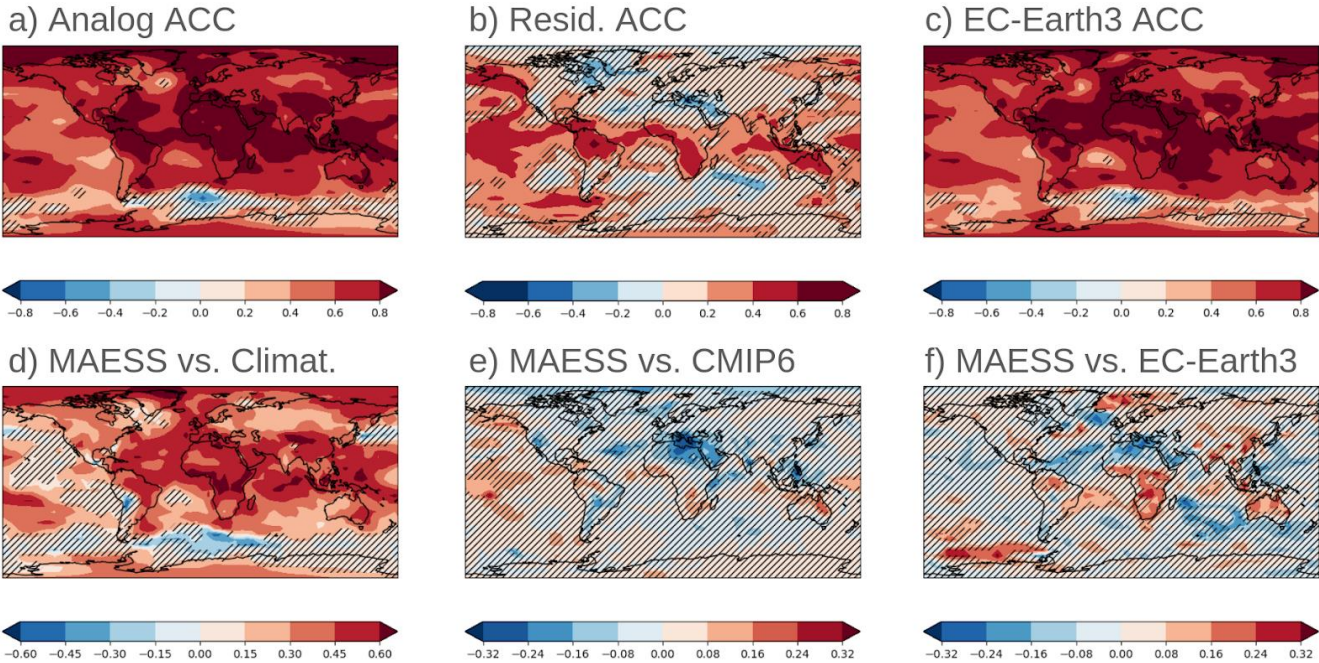
305 Figure 7: The same as Figure 1, but for biennial TAS predictions (January - December+1year). The evaluation period is 1962-2018. The predictions are initialized each November in both analog-based predictions and EC-Earth3. The dynamic forecasts system evaluated in c,f is EC-Earth3.
