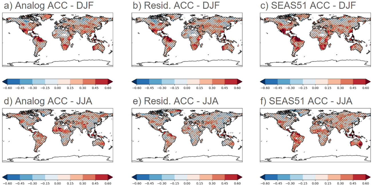
230 Figure 3: a) ACC between December-February analog-based ensemble mean predictions and observations of SPI3 b) Residual ACC between December-February analog-based ensemble mean predictions and observations of SPI3 c) ACC between ECMWF-SEAS51 December-February ensemble mean predictions and observations of SPI3. d) ACC between June-August analog-based ensemble mean predictions and observations of SPI3. e) Residual ACC between June-August analog-based ensemble mean predictions and observations of SPI3. f) ACC between ECMWF-SEAS51 235 June-August ensemble mean predictions and observations of SPI3. The evaluation period is 1982-2018. The predictions are initialized each November (a-c) and each May (d-f). The hatched regions in all figures indicate statistically non-significant values ( p < 0.1 ) using a two-sided t-test.
