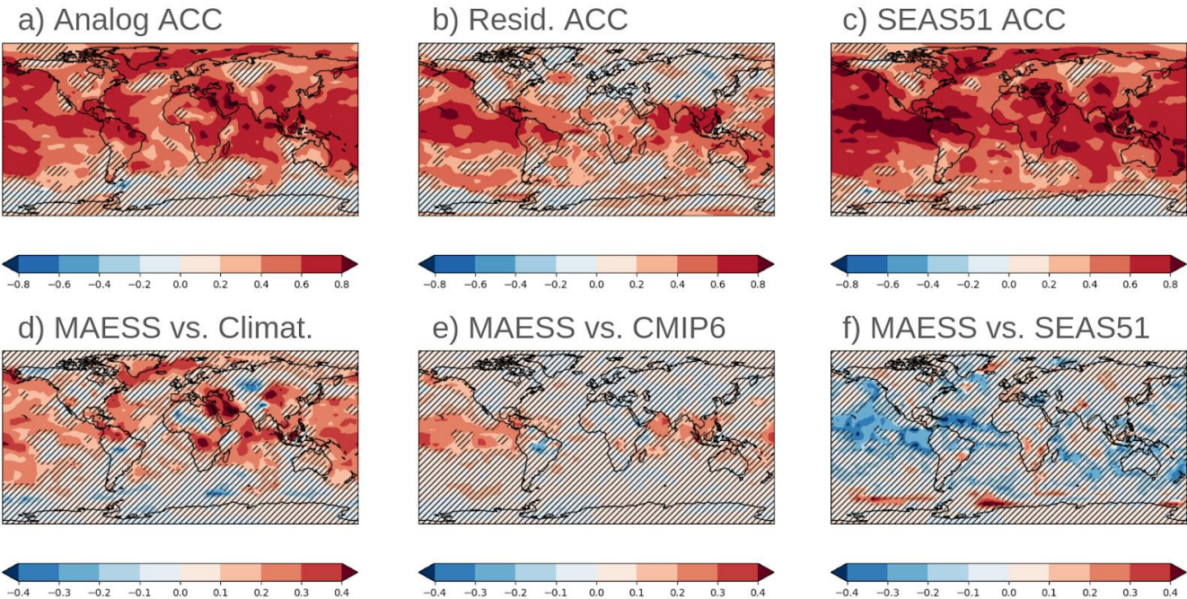
215 Figure 2: The same as Figure 1, but for June-August TAS predictions. The predictions are initialized each May.
