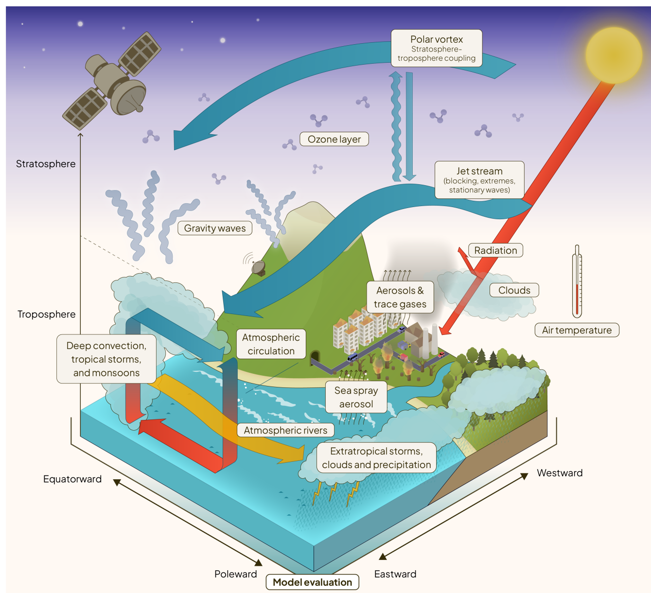
Figure 1 Processes covered by the Atmospheric theme opportunities. The 'Model evaluation' label and box implies that model evaluation encompasses all atmospheric processes. Figure originally published at Dingley et al., 2025 (see https://doi.org/10.5281/zenodo.15681839 )
