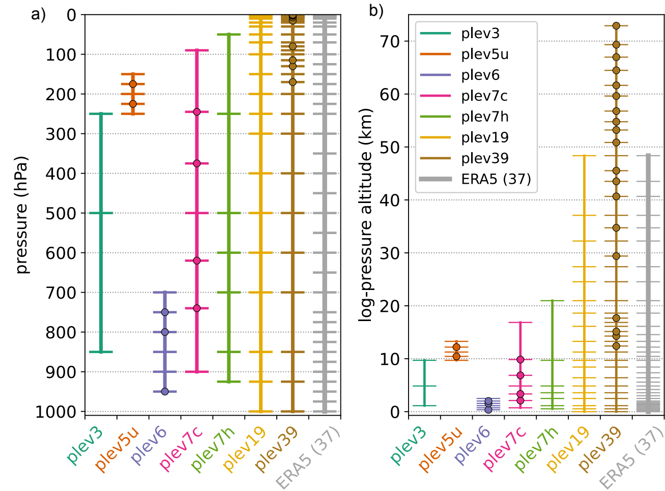
Figure 2: Pressure level sets utilised in the CMIP7 Data Request. Pressure level set names shown on the x-axis are ordered from fewest to most pressure levels. For comparison the standard pressure levels from the ERA5 reanalysis are also shown as the right-most line (light grey). The y-axis shows a) pressure altitude in hectopascals, and b) the log-pressure altitude in kilometres, in order
