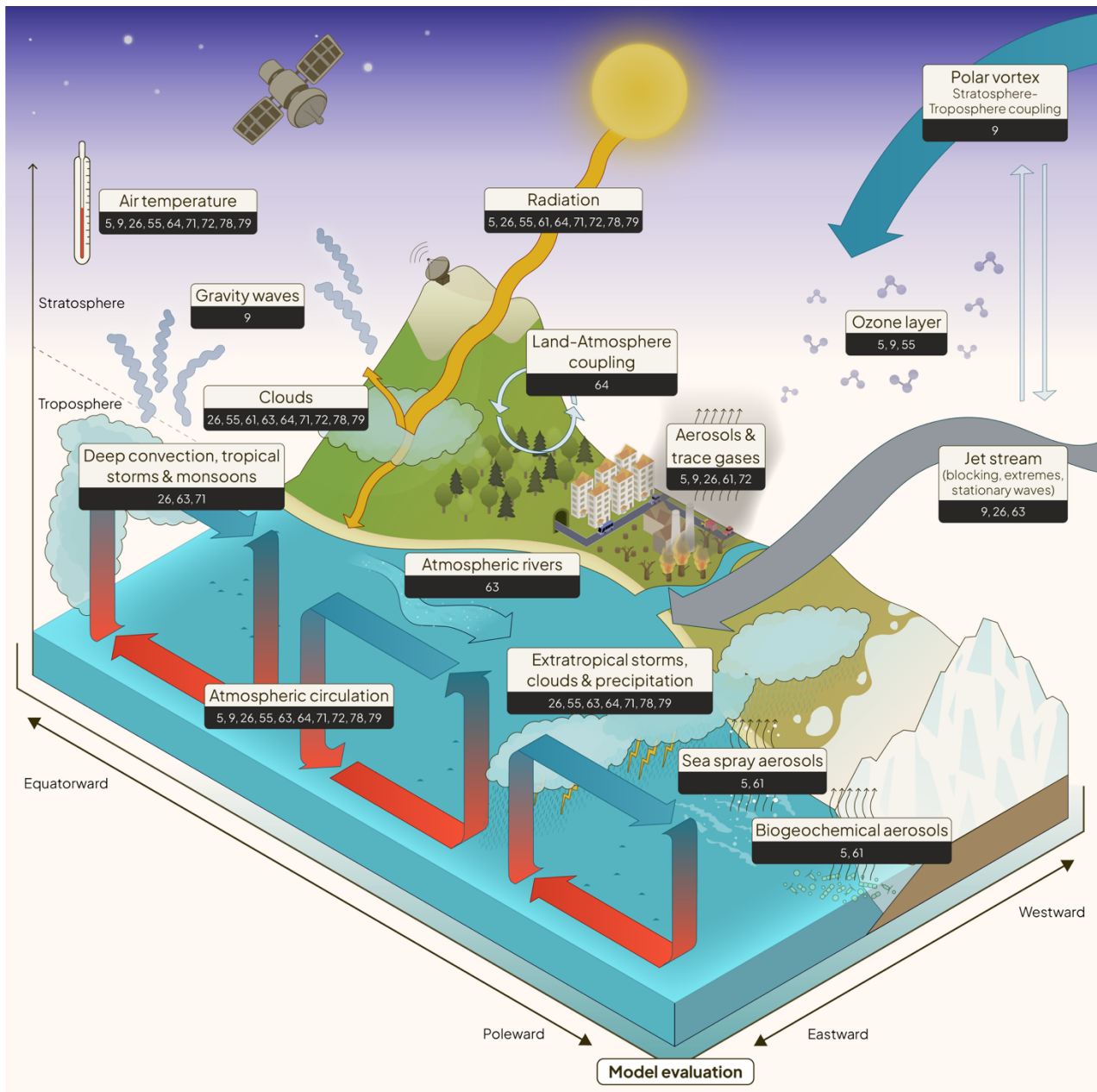
105 Figure 1 Processes covered by the Atmospheric theme opportunities. The 'Model evaluation' label and box implies that model evaluation encompasses all atmospheric processes. The numbers beneath each process indicate which Opportunity IDs in the Atmosphere theme address that process. Figure originally published at Dingley et al., 2025 (see https://doi.org/10.5281/zenodo.15681839 )
