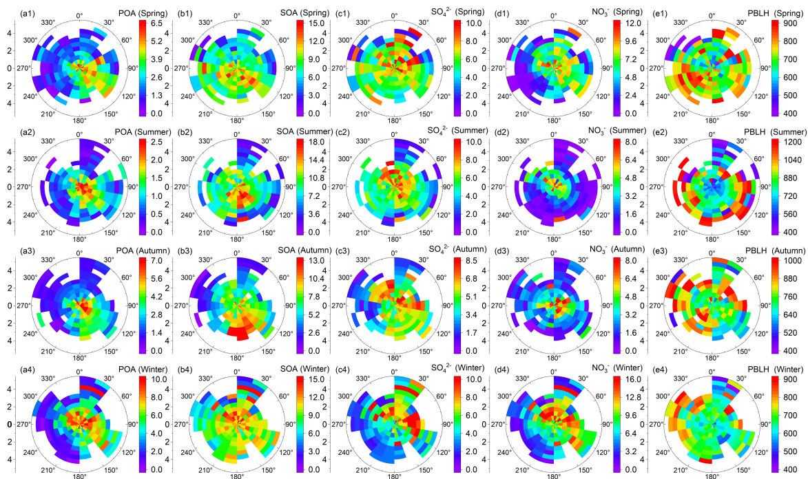
Figure 10: Pollution roses of (a) POA, (b) SOA, (c) sulfate, (d) nitrate and (e) PBLH during four seasons. The data are grouped into grids with increments of WS and WD being 0.5 \text{ m s}^{-1} and 20^\circ , respectively. The unit of color scale is \mu\text{g m}^{-3} .
