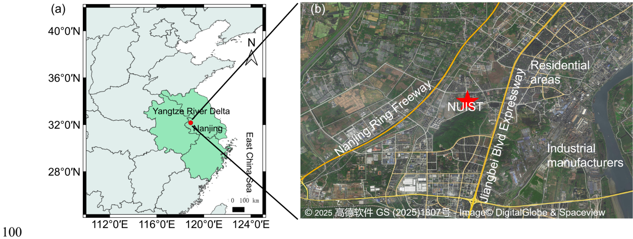
Figure 1: (a) Geographical location of Nanjing in the Yangtze River Delta and (b) the distribution of pollution sources around the NUIST observation site (source: Gaode Map, GS (2025)1807). The base map contains data from DigitalGlobe and Spaceview.
