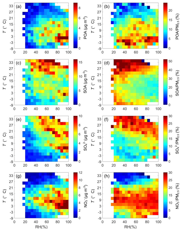
Figure 3: RH / T dependence of mass concentrations and mass fractions in \text{PM}_{2.5} of POA, SOA, sulfate, and nitrate for the entire period. The data are grouped into grids with increments of RH and T being 5 % and 3 °C, respectively. Grid cells with the number of data points fewer than 10 are excluded.
