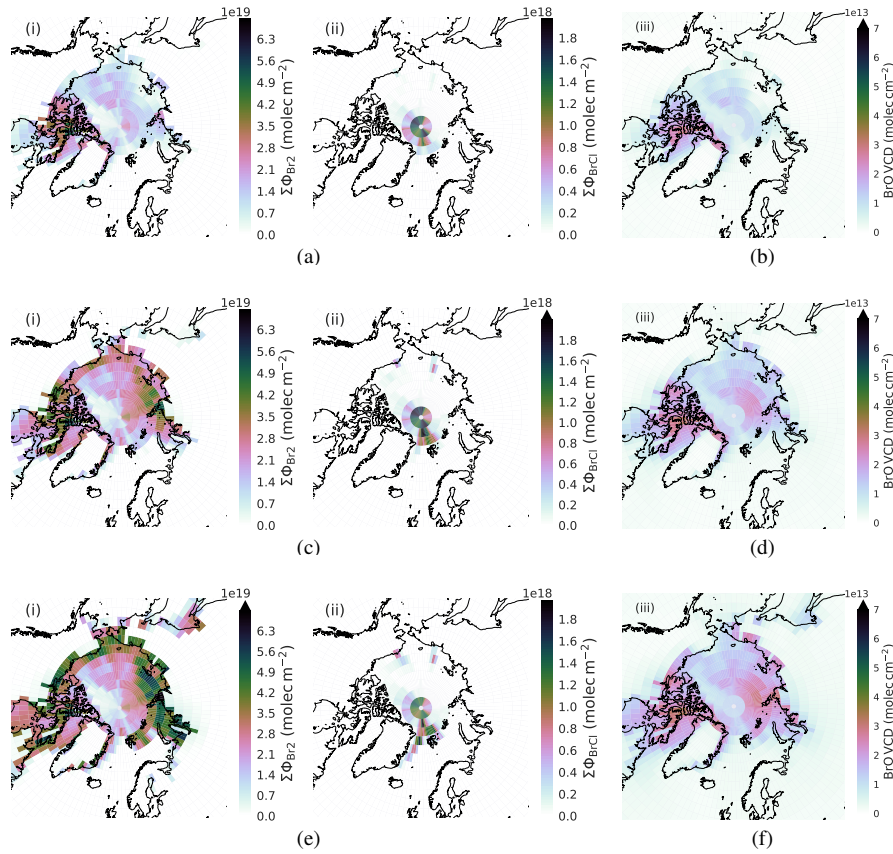
Figure 6. Br 2 (i) and BrCl (ii) flux integral and monthly mean tropospheric BrO VCD at 13–14 h local time (iii) for April 2019. The EMAC total column BrO has been split into tropospheric and stratospheric contributions using the modeled PV-tropopause height on hourly basis. (a, b) T_{\text{crit}} = -15^\circ\text{C} (sfa010); (c, d) T_{\text{crit}} = -10^\circ\text{C} (sfa011); (e, f) T_{\text{crit}} = -2.5^\circ\text{C} (sfa012).
