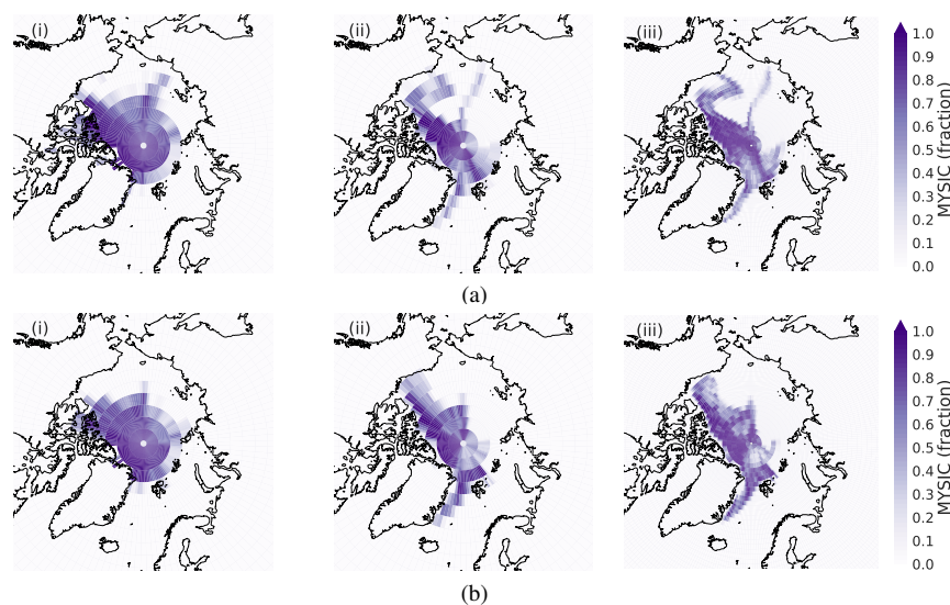
Figure A1. Maps of multi-year sea ice cover in April. (i) Estimated from ERA5 sea ice cover at seasonal low of the previous year, (ii) ICDC Age of Sea Ice product (T42), and (iii) ICDC Age of Sea Ice product (T106). The comparison between T42 and T106 illustrates the potential benefit of a higher model resolution for resolving inhomogeneity in the characteristics of sea ice such as its age. (a) 2019; (b) 2020.
