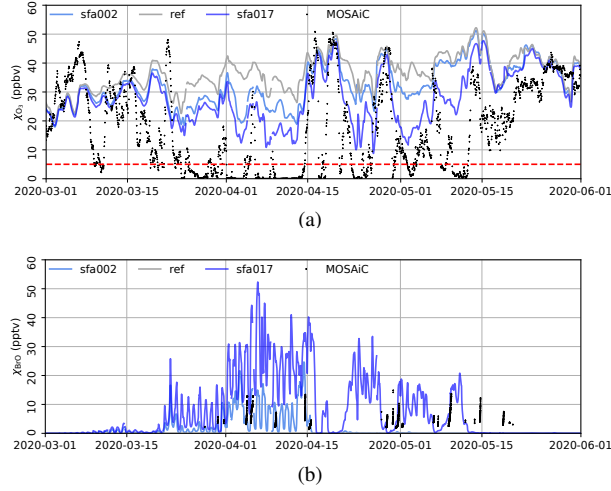
Figure 9. Evaluation of EMAC experiments (ref, sfa002, sfa017) interpolated onto MOSAiC drift track. Compared to MOSAiC observations. (a) O_3 ; (b) BrO. Note that \chi_{BrO} were not present in the reference experiment.
