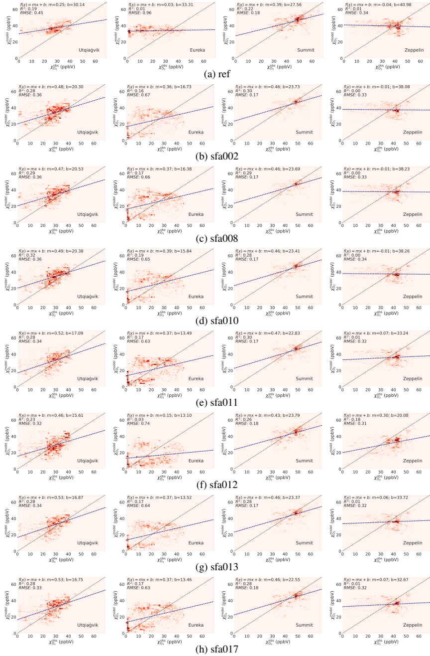
Figure A4. Sensitivity test. 2D histogram and linear fit of \chi_{O_3}^{\text{model}} vs \chi_{O_3}^{\text{obs}} for 2019, March–May. The respective root-mean-square error (RMSE) and coefficient of determination R^2 are listed in Appendix Table A1. From top to bottom: model experiments as given in Tab. 2. Ozone monitoring sites from left to right: Utqiagvik, Eureka, Summit, and Zeppelin.
