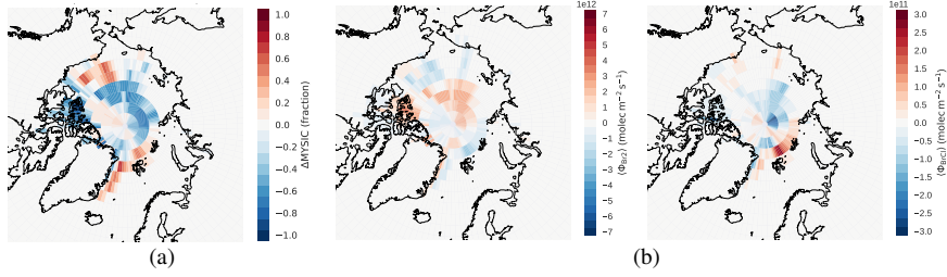
Figure 5. Influence of MYSIC on AirSnow emission fluxes. (a) MYSIC difference ICDC AoSI-ERA5. (b) Br 2 (left) and BrCl (right) flux difference between a model experiments with ICDC AoSI (sfa010) and ERA5 (sfa008).
