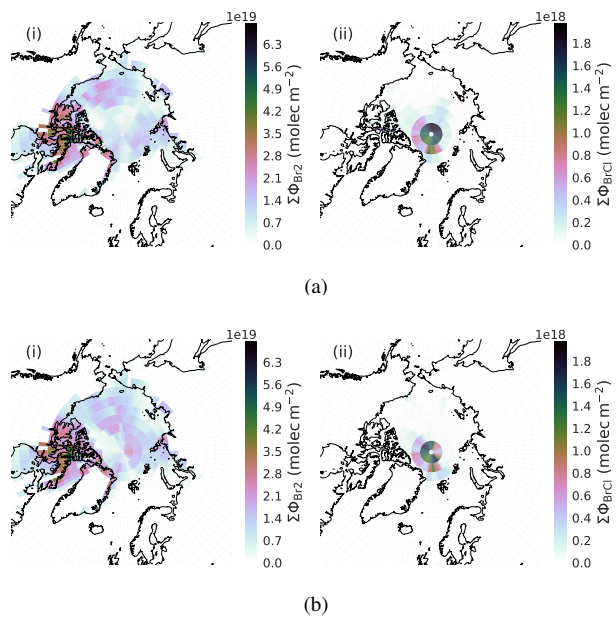
Figure A3. \text{Br}_2 (i) and \text{BrCl} (ii) flux integral for April 2019 with MYSIC based on (a) ERA5 SIC (sfa008); (b) ICDC AoSI (sfa010).
