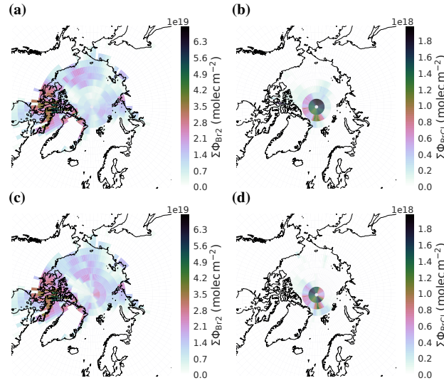
Figure A3. Comparison of modeled bromine emissions due to BEs. Flux integral of (ia, c) Br 2 and (ib, d) flux integral BrCl for April 2019 with MYSIC based on (a, b) ERA5 SIC (sfa008); (bc, d) ICDC AoSI (sfa010).
