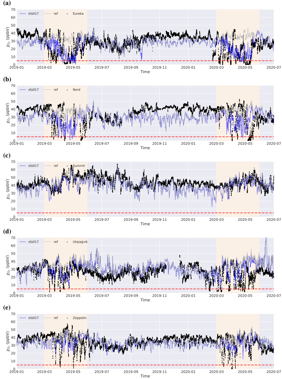
Figure 7. Time series comparing observational records of \chi_{\text{O}_3} at Arctic ozone monitoring sites with EMAC model output (ref, sfa017) interpolated to the station location. The periods March–May are highlighted in light yellow. The dashed red line indicates the 5 ppb 5 ppbv threshold for ODEs. (a) Eureka; (b) Nord; (c) Summit; (d) Utqiagvik; (e) Zeppelin.
