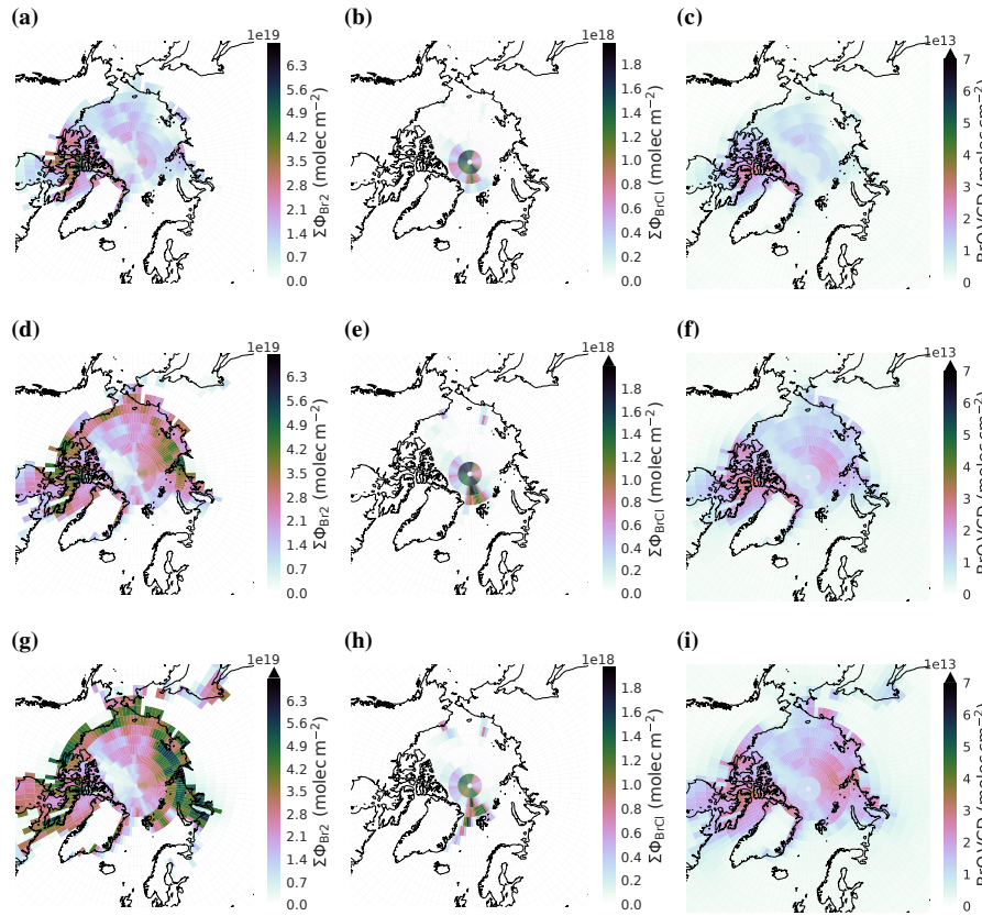
Figure 6. Comparison of modeled bromine emissions due to BEs and tropospheric BrO VCD. Flux integral of (a, d, g) \text{Br}_2 and (b, e, h) flux integral-BrCl and monthly mean tropospheric BrO VCD at 13 – 14h local time (c, f, i) for April 2019. The EMAC total column BrO has been split into tropospheric and stratospheric contributions using the modeled PV-tropopause height on hourly basis. (a, b, c) T_{\text{crit}} = -15^\circ \text{C} (sfa010); (d, e, f) T_{\text{crit}} = -10^\circ \text{C} (sfa011); (g, h, i) T_{\text{crit}} = -2.5^\circ \text{C} (sfa012).
