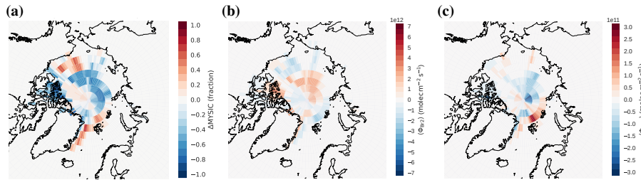
Figure 5. Influence of MYSIC on AirSnow emission fluxes. (a) MYSIC difference ICDC AoSI-ERA5. (b) Br 2 (left) and (right) BrCl flux difference between a model experiments with ICDC AoSI (sfa010) and ERA5 (sfa008).
