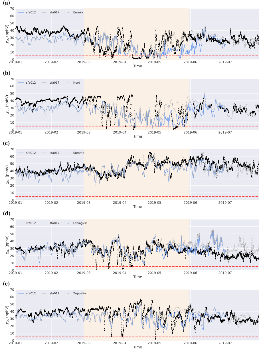
Figure B2. Time series comparing observational records of \chi_{\text{O}_3} at Arctic ozone monitoring sites with EMAC model output (sfa012, sefa017) interpolated to the station location. The periods March–May are highlighted in light yellow. The dashed red line indicates the 5 ppb 5 ppbv threshold for ODEs. (a) Eureka; (b) Nord; (c) Summit; (d) Utqiaġvik; (e) Zeppelin. For early spring (March to April), no differences are expected. The difference in T_{\text{crit}} will only affect May if surface temperatures rise above -10^\circ\text{C} .
