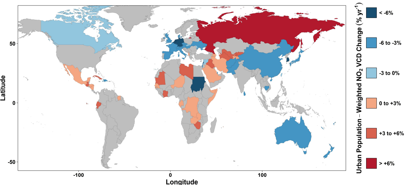
233 234 Figure 4: Global spatial representation of the urban population-weighted NO 2 VCD % change yr -1 from 2019 to 2024. Gray fill 235 denotes statistical insignificance ( p > 0.05 ).
