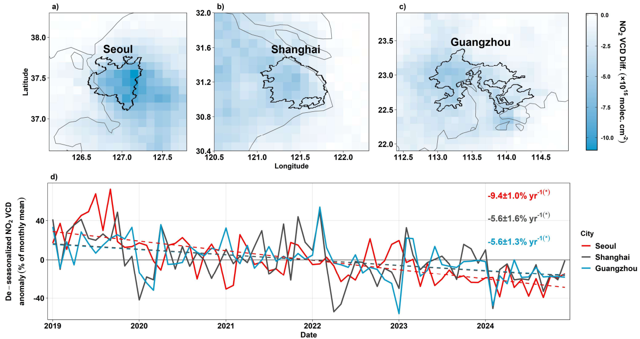
220 Figure 3: Absolute change in mean annual NO 2 VCD from 2019 to 2024 for three East Asian cities: (a) Seoul, South Korea, (b) 221 Shanghai, China and (c) Guangzhou, China. Colors in panels a-c show magnitude of VCD change, thin lines show national borders 222 or coastlines, and thick lines show the GHS-SMOD urban boundary. (d) Solid lines show de-seasonalized monthly VCD anomaly 223 from 01/2019 through 12/2024, colored by city. Dashed lines are produced from ordinary least-squares regression. The % change 224 yr -1 , standard error and statistical significance is reported in the top right of panel d.
