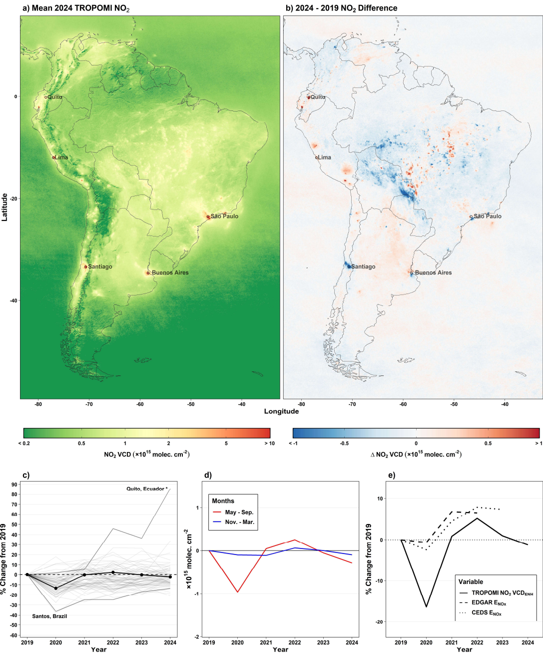
431 432 Figure 11: Same as Fig. 6, but for South America.
