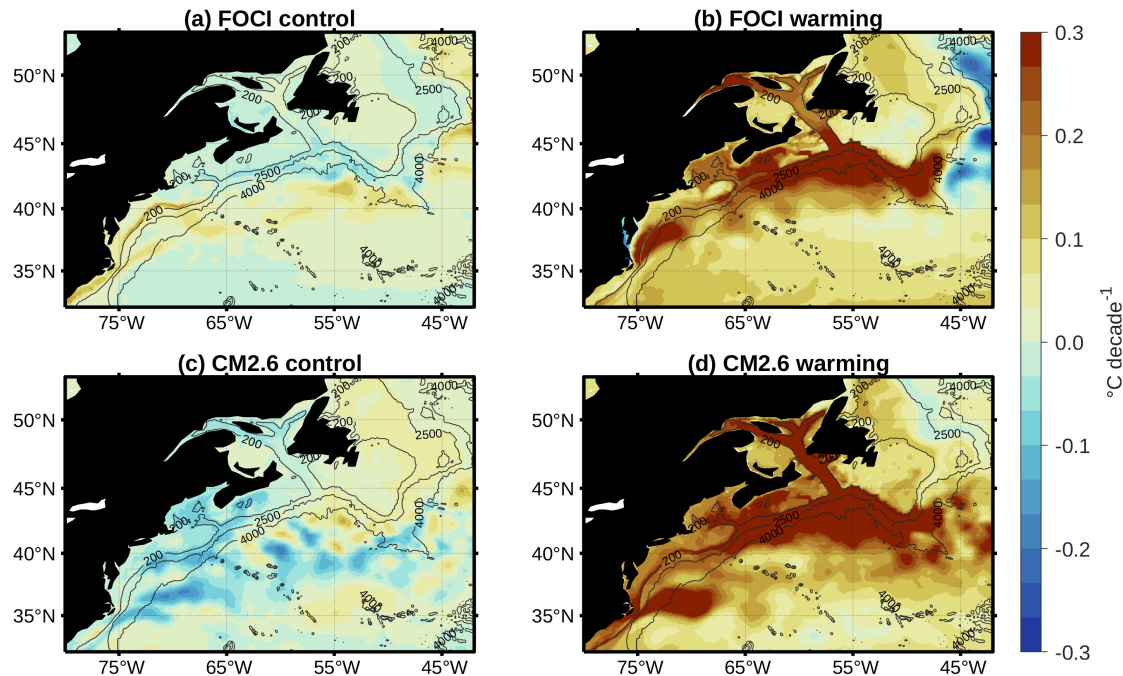
165 Figure 1 Linear trends in annual-mean bottom (or 200 m where the water column is deeper than 200 m) temperature between 2015 and 2100 for (a) FOCI control, (b) FOCI warming, (c) CM2.6 control, and (d) CM2.6 warming simulations. Trends are calculated from annual means.
