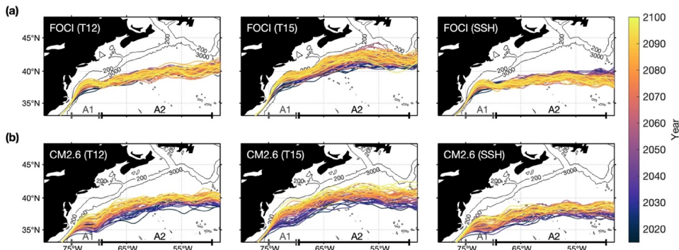
Figure 4 Annual mean location of the GS path based on temperature (T12 and T15) and SSH criteria in the warming simulations of FOCI (a) and CM2.6 (b). Colors indicate different years from 2015 to 2100. Regions A1 and A2 (shown along the x-axis) indicate the longitude bands over which latitudes are averaged in Figure 5.
