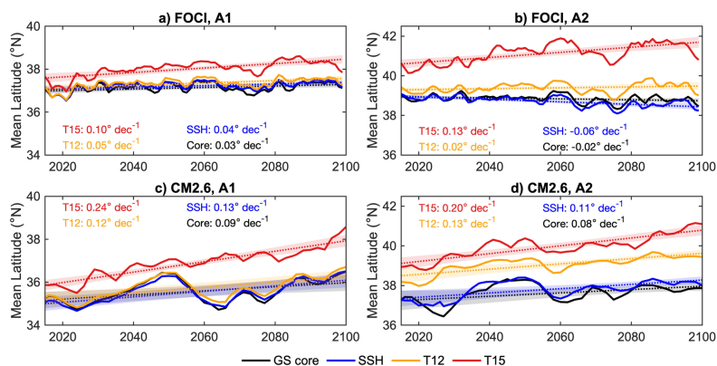
Figure 5 Mean latitude of the temperature-based (T12 and T15) and SSH-based Gulf Stream path criteria averaged over two regions: A1 (75° W to 70° W, grey bracket in Fig. 4) and A2 (71° W to 50° W, black bracket in Fig. 4) in FOCI (a, b) and CM2.6 (c, d) simulations. Solid lines show the annual mean latitude of each proxy, along with the reference Gulf Stream core position (GS core). Dotted lines indicate the corresponding linear trends, and shaded bands represent the 95% confidence interval of the fitted mean trend. Trend magnitudes (in ° latitude per decade) are reported within each panel for each proxy. Trend statistics are provided in Table S1.
