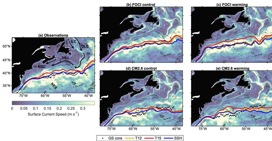
175 Figure 2 Annual mean surface velocity and GS position from observations (a), FOCI (b, c), and CM2.6 (d, e) in 2015. Background shading shows the mean surface current speed ( \text{m s}^{-1} ). Orange contours are the 12\text{ }^{\circ}\text{C} isotherm at 450 m depth (T12). Red contours indicate the 15\text{ }^{\circ}\text{C} isotherm at 200 m depth (T15). Blue contours show the SSH of -0.23\text{ m} for CM2.6, 0.1\text{ m} for FOCI, and 0.25\text{ m} for the observations. Black points represent the locations of maximum surface velocity (GS core). Black arrows in (a) show the approximate location of the Nova Scotia current (NSC), shelfbreak jet (SBJ) and the inner (ILC) and outer (OLC) Labrador Current. NES: New England Seamounts.
