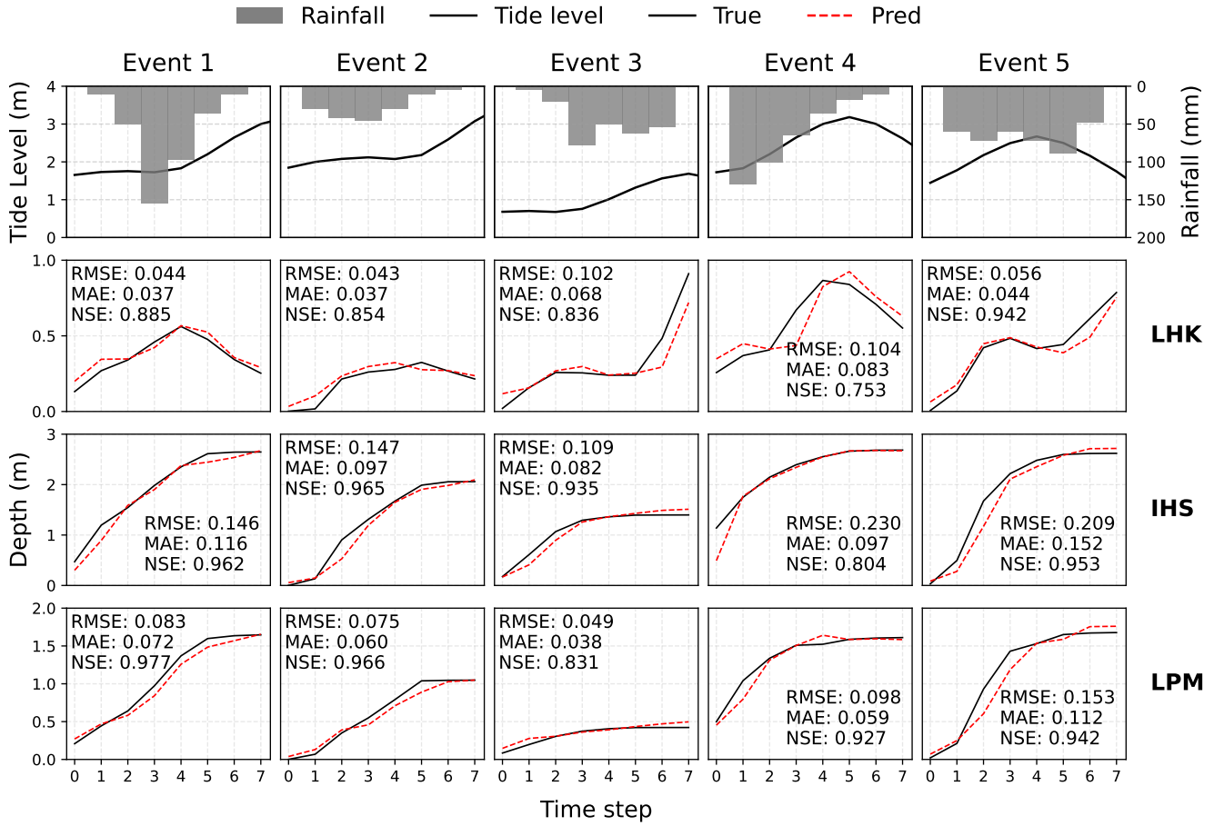
Figure 8. Observed and predicted water depth processes at three flood-prone locations (LHK, IHS, and LPM) during five rainfall events. Tide level and rainfall are shown in the top row, followed by time series of observed and predicted water depths at each site. Model performance for each event is quantified using RMSE (m), MAE (m), and NSE.
