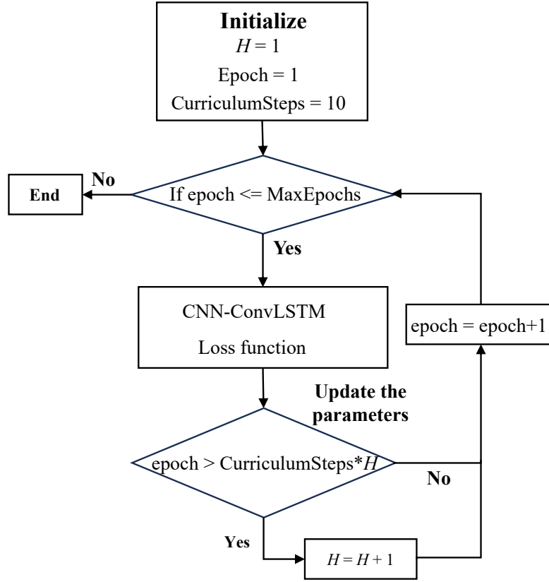
Figure 6. Workflow of curriculum learning strategy. The workflow includes initialization, progressive training stages across epochs, and parameter updates designed to improve convergence and predictive stability.
