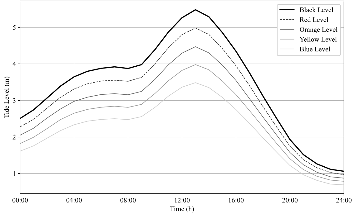
Figure 3. The designed tidal process lines. Temporal variations in tide level (m) are shown for five threshold processes (black, red, orange, yellow, and blue lines), illustrating daily tidal fluctuations used in model simulations.
