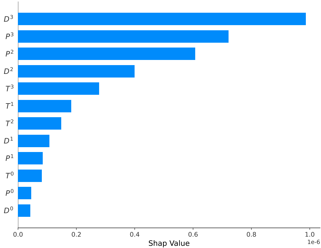
Figure 13. SHAP values of dynamic features. P^t , D^t , and T^t represent rainfall, inundation depth, and tide level at time step t , respectively. Bar lengths indicate the magnitude of each feature's contribution to model predictions, with larger SHAP values reflecting stronger influence.
