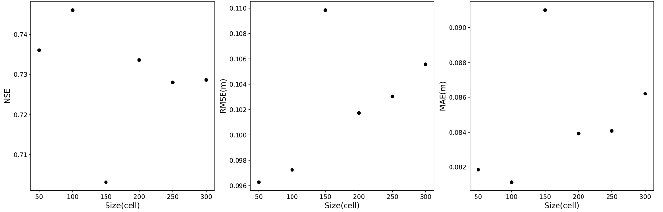
Figure 7. Sensitivity of model performance to tile size (50–300 cells), with the best overall scores at 100 cells. NSE (left), RMSE (middle), and MAE (right) are shown as functions of tile size. Each black marker corresponds to one model run for a given tile size evaluated on the same dataset. Higher NSE and lower RMSE/MAE indicate better performance.
